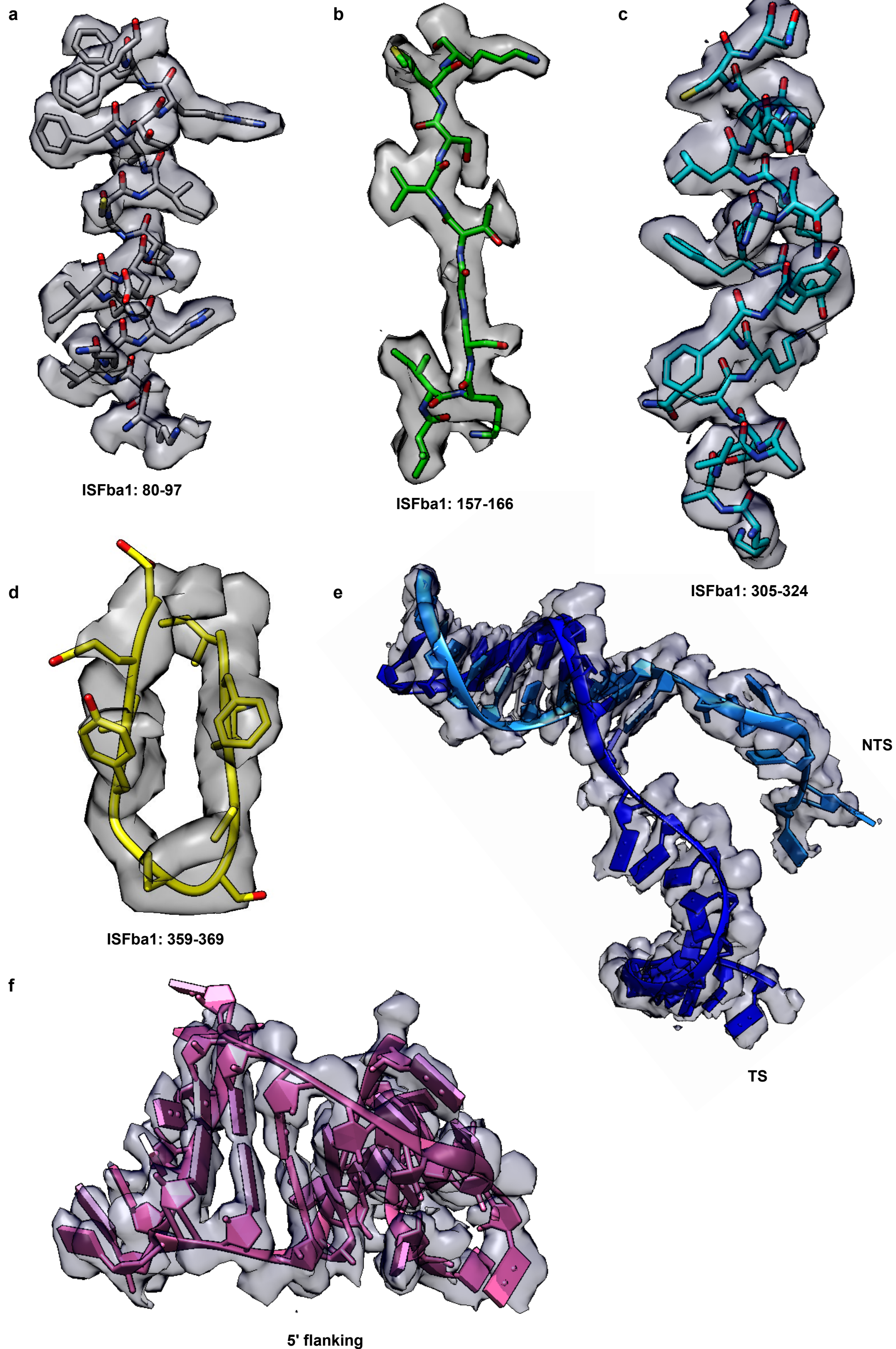
Supplementary information, Fig.S5: Representative local map density for the IS607 TnpB complex.
