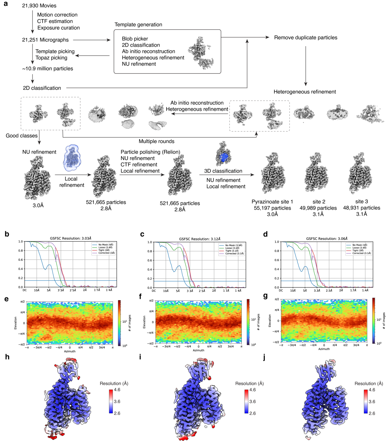
Fig. S4 Cryo-EM analyses of URAT1 in pyrazinoate-bound states
