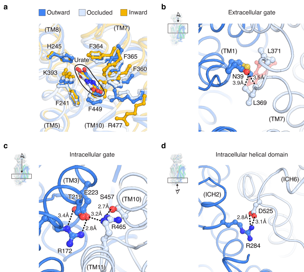
Fig. S9 Structural analyses of the urate pocket and transporter gates
