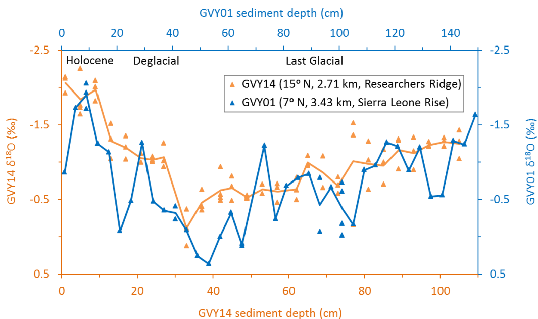
160 161 Supplementary Figure 9. Planktonic \delta^{18}\text{O} records of GYV14 and GYV01. The measurements were carried out on 162 10–12 specimens of the planktonic foraminifera, G. ruber , picked from the 250–355 \mu\text{m} size fraction, and 163 analysed using a Thermo Delta V Plus mass spectrometer coupled with a Kiel IV automated carbonate-sample 164 preparation device, in the New Core Lab stable isotope laboratory at the Lamont-Doherty Earth Observatory. 165 Calibration of measurements to the Vienna Peedee belemnite (VPDB) isotope scale was carried out using NBS-19 166 and NBS-18 reference materials 22 . The in-house standard 1 s.d. reproducibility for \delta^{18}\text{O} is \pm 0.06 ‰.
