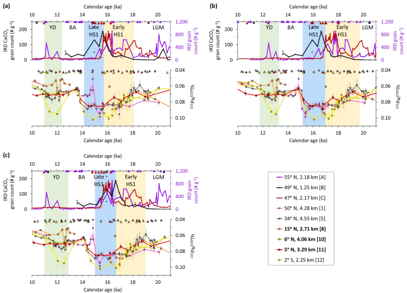
Supplementary Figure 14. Sediment reservoir uncertainty in sediment core age models. Age models were developed using several combinations of surface reservoir values derived for high latitudes ( >45^{\circ} N) and low latitudes ( <35^{\circ} N/S) over the last 25 kyr 27 : (a) maximum surface reservoir values at all sites, (b) minimum surface reservoir values at all sites, (c) maximum values at eastern high latitudes, minimum values at western high latitudes, and mean values at low latitudes. No changes were made to the age model for the Rockall basin core ( 50^{\circ} N, 4.28 km) which was developed using non- ^{14}\text{C} chronological tie-points 9 . Triangle and diamond symbols indicate respectively the ^{14}\text{C} and non- ^{14}\text{C} chronological tie-points of the sediment core age models. Bracketed numbers denote the core identities marked in main text Fig. 1, with references listed in main text Table 1. Bold characters in the figure legend and the square symbols indicate ^{231}\text{Pa}/^{230}\text{Th} reconstructions from this study. Error bars represent 2 s.e.m.
