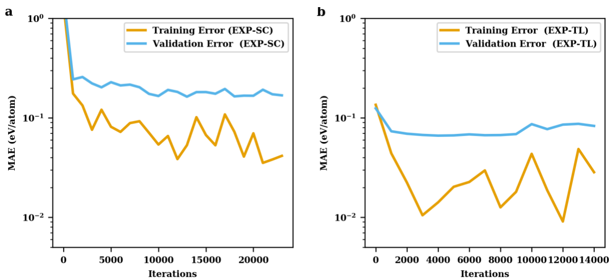
Supplementary Figure 3: Training curve for an ElemNet model trained on experimental dataset containing 1,643 observations from one split of the ten-fold cross validation. We present the training error curve for ElemNet [1] model trained on the experimental dataset from scratch- EXP-SC and using transfer learning from OQMD-SC model- EXP-TL. The training curves show the training and validation error during training the models. When training from scratch in case of EXP-SC (a), the weights are initialized randomly from a uniform distribution; for transfer learning in case of EXP-TL (b), the model weights are initialized from the OQMD-SC model and then fine-tuned using the corresponding dataset. The OQMD-SC model is trained from scratch using a 9:1 random split of training and test set from OQMD. The models were trained using a minibatch size of 64; they were evaluated every 1000 iterations (the training error corresponds to evaluation using current mini-batch, the validation error corresponds to evaluation using whole validation set); since the dataset size is small, the error curve has fewer points and hence not smooth. A patience of 200 minibatch iterations is used for early stopping; the training stops if the validation error does not improve in next 200 minibatch iterations. The error curves are typically used for analyzing the convergence of the model and overfitting to training dataset for proper training.
