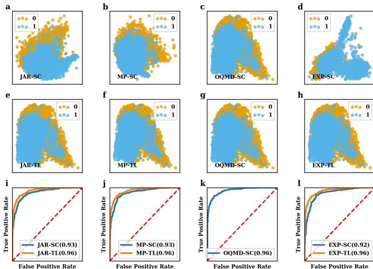
Supplementary Figure 2: Analysis of the activations from the first hidden layer of the ElemNet architecture for the insulator vs metallic class (1 and 0) from JARVIS dataset. The four columns represent the models trained using four different datasets- (a, e and i) JARVIS (JAR), (b, f and j) Materials Project (MP), (c, g and k) OQMD and (d, h and l) the experimental observations (EXP); the first (a-d) and second (e-h) rows represent the models trained from scratch (SC) and using transfer learning (TL), while the third row (i-l) represents the ROC curves from the Logistic Regression model trained using all activations from the same hidden layer (the corresponding AUC values are shown in brackets) on the respective datasets. The scatter plots demonstrate the first two principal components of the activations using principal component analysis (PCA) technique.
