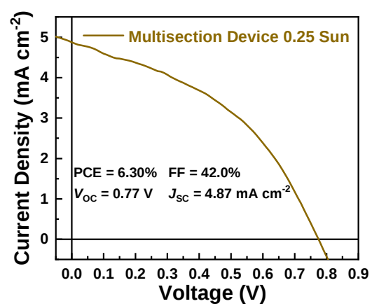
Supplementary Figure 4. The J - V curve of the interdigital lateral-structure \text{MAPbI}_3 single-crystalline device.
