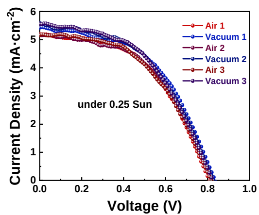
Supplementary Figure 2. The J - V curves measured in vacuum and air condition.
