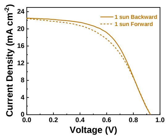
Supplementary Figure 1. The J - V plots of lateral structured device in both forward and backward direction under 1 Sun.
