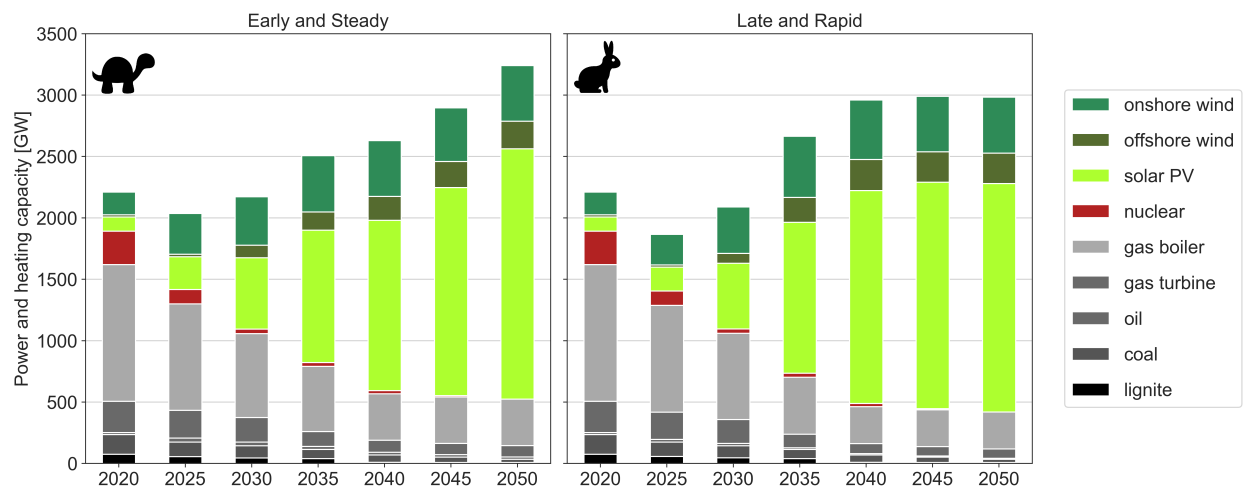
Supplementary Figure 7: Installed capacities for different technologies throughout transition paths shown in Fig. 1 in the main text.
