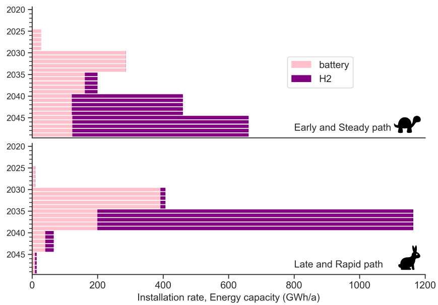
Supplementary Figure 9: Annual build rates for batteries and hydrogen storage throughout transition paths shown in Fig. 1 in the main text.
