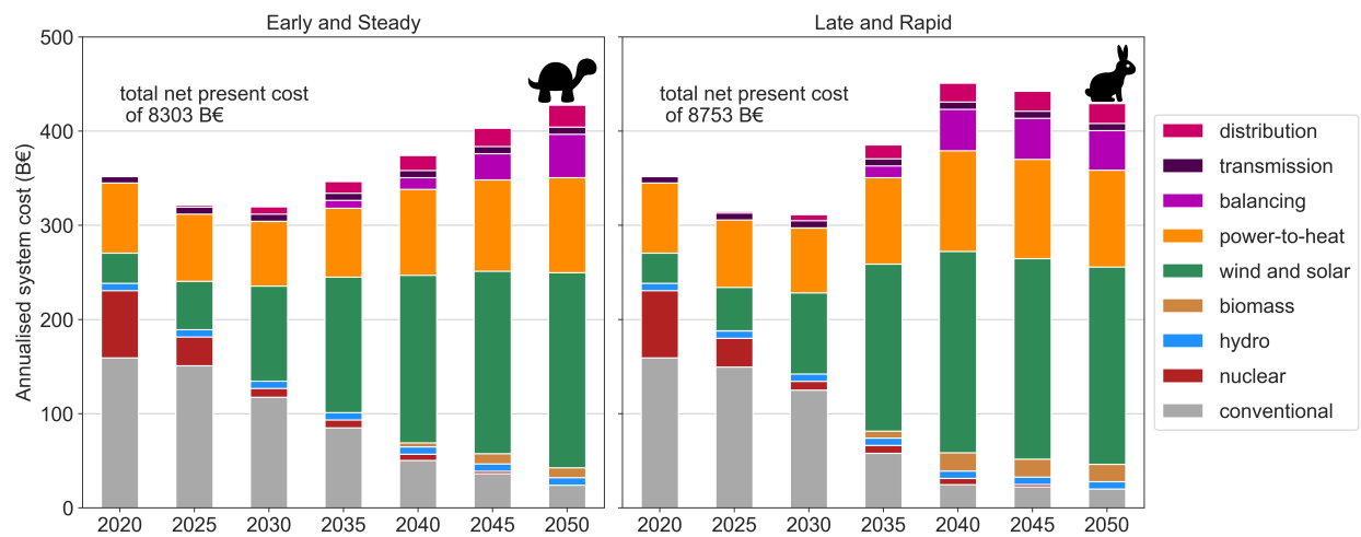
Supplementary Figure 19: Annualised system cost for the European electricity, heating and transport system throughout transition paths Early and Steady and Late and Rapid. Conventional includes costs associated with coal, lignite, and gas power plants producing electricity as well as costs for fossil-fueled boilers and CHP units. Power-to-heat includes costs associated with heat pumps and heat resistors. Balancing includes costs of electric batteries, H 2 storage, and methanation.
