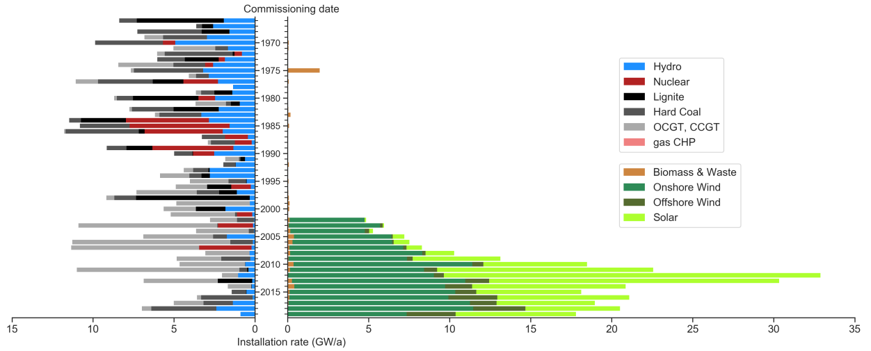
Supplementary Figure 25: Age distribution of European power plants in operation [3, 6].
