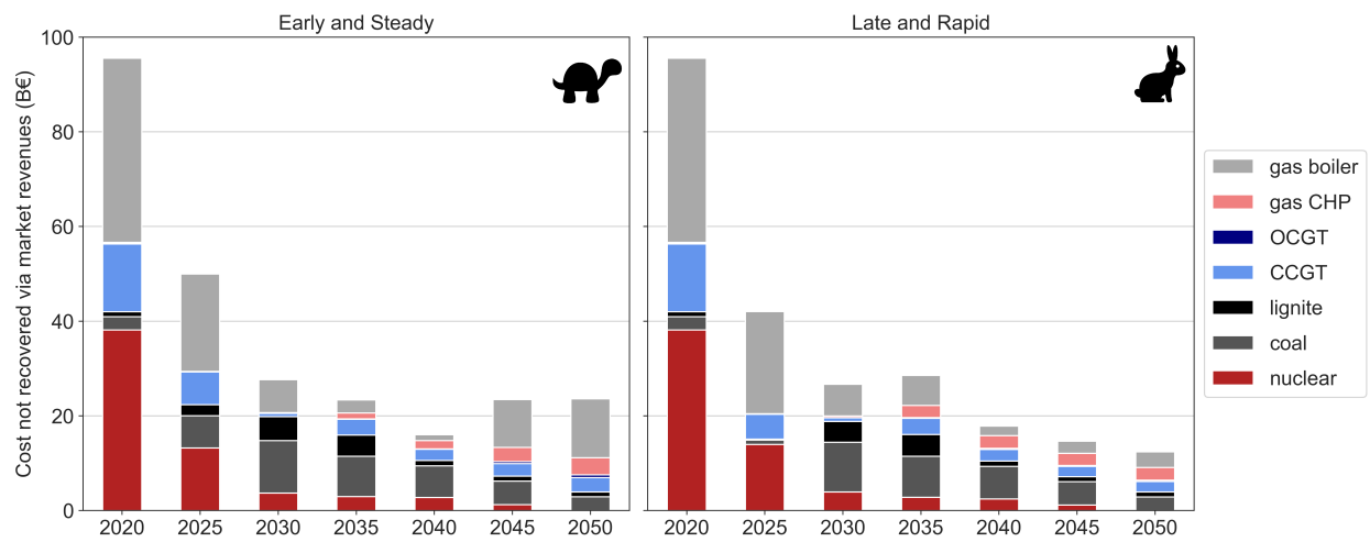
Supplementary Figure 14: Expenditures not recovered via market revenues for lignite, coal, OCGT, CCGT, nuclear power plants and gas boilers throughout transition paths shown in Fig. 1 in the main text.
