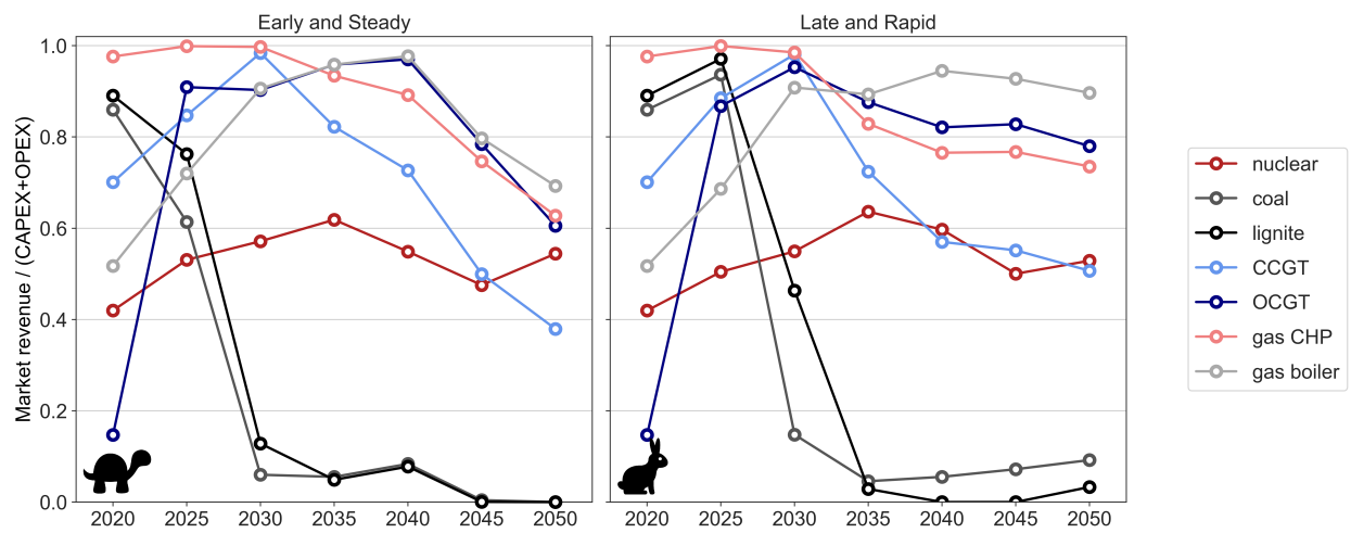
Supplementary Figure 12: Ratio of market revenues to total expenditure for lignite, coal, OCGT, CCGT, nuclear power plants and gas boilers throughout transition paths shown in Fig. 1 in the main text. Total expenditure includes fixed and variable costs, fuel costs and cost associated with CO 2 price.
