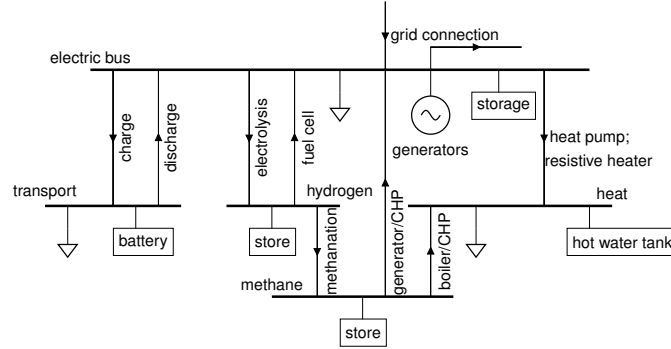
Supplementary Figure 23: Energy flow at a single node representing a country. Within each node, there is a bus (thick horizontal line) for every sector (electricity, transport and heating), to which different loads (triangles), energy sources (circles), storage units (rectangles) and converters (lines connecting buses) are attached. This is equivalent to the diagram shown in Fig. 7 in the main text.
