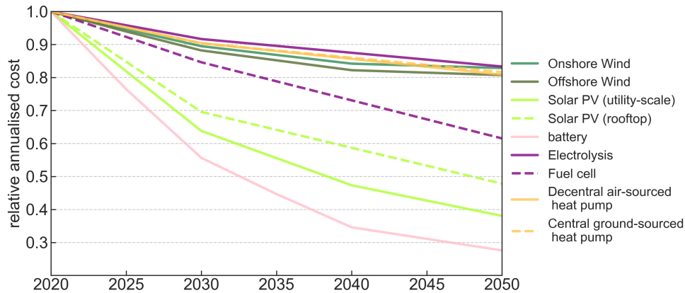
Supplementary Figure 26: Evolution of annualised costs, relative to 2020, for some selected technologies.
