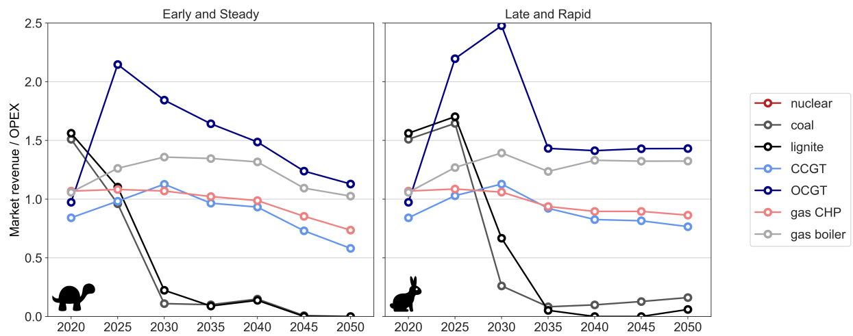
Supplementary Figure 13: Ratio of market revenues to operational expenditure (OPEX) for lignite, coal, OCGT, CCGT, nuclear power plants and gas boilers throughout transition paths shown in Fig. 1 in the main text. OPEX includes fixed and variable operation and maintenance costs, fuel costs and cost associated with CO 2 price.
