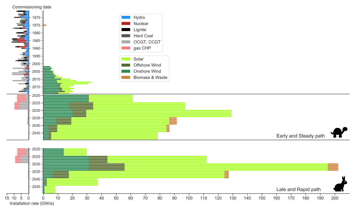
Supplementary Figure 5: Age distribution of European power plants in operation [3, 6] and required annual installation throughout the Early and Steady and Late and Rapid paths.
