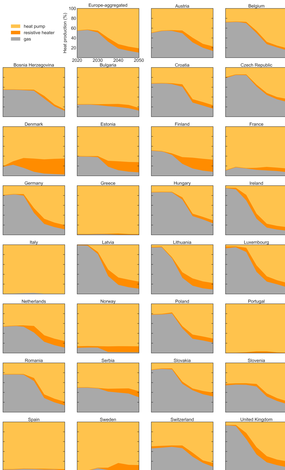
Supplementary Figure 17: Evolution of technologies used to supply heating in the residential and services sector in the Early and Steady path. Fuel used in gas boilers is synthetic methane produced by combining electrolysed-H 2 and direct-air-captured CO 2 .
