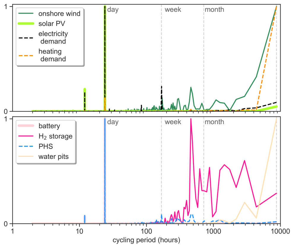
Supplementary Figure 18: Fourier power spectra of wind and solar PV generation, electricity and heating demand, as well as storage technologies dispatch. Time series represent the Europe-aggregated generation/demand for the Early and Steady path in 2050.
