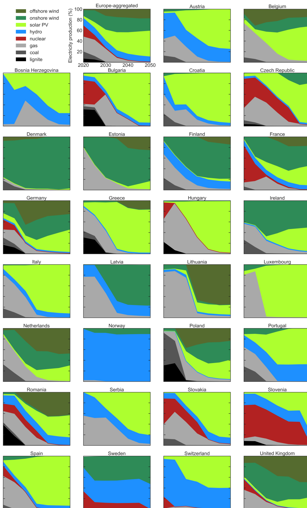
Supplementary Figure 16: Evolution of the electricity generation mix in every country for the Early and Steady transition path. Fuel used in OCGT plants is synthetic methane produced by combining electrolysed-H 2 and direct-air-captured CO 2 .
