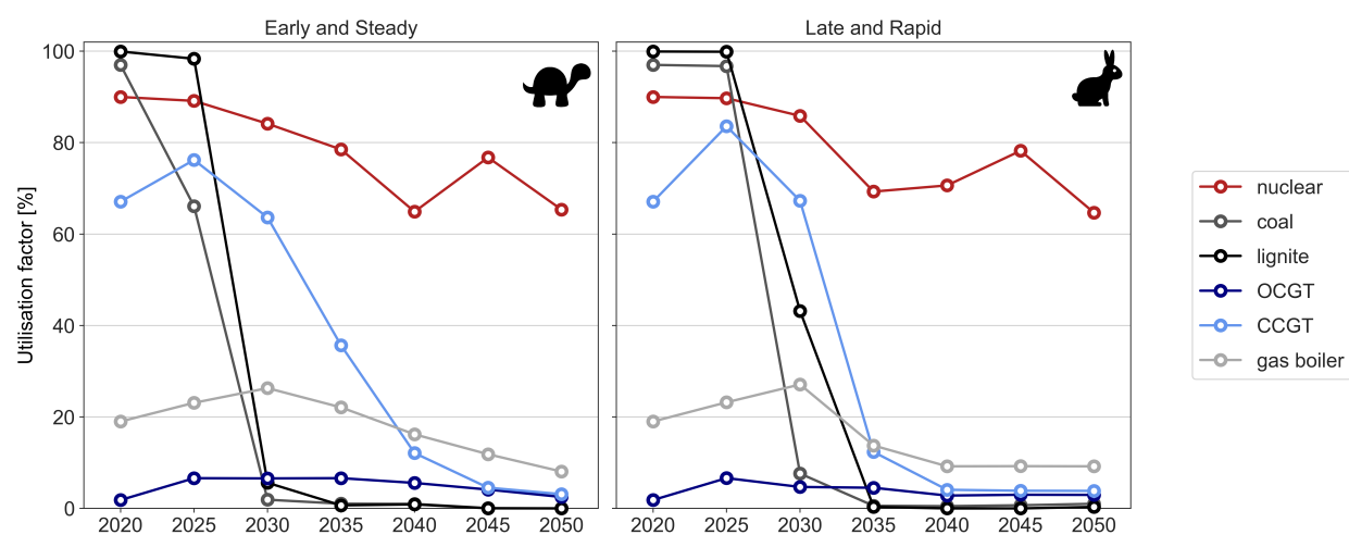
Supplementary Figure 11: Utilisation factors for lignite, coal, OCGT, CCGT, nuclear power plants and gas boilers throughout transition paths shown in Fig. 1 in the main text.
