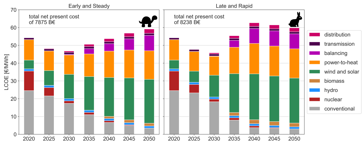
Supplementary Figure 6: Levelized Cost of Energy (LCOE) for the European electricity and heating system throughout transition paths Early and Steady and Late and Rapid shown in Fig. 1 in the main text. Conventional includes costs associated with coal, lignite, and gas power plants producing electricity as well as costs for fossil-fueled boilers and CHP units. Power-to-heat includes costs associated with heat pumps and heat resistors. Balancing includes costs of electric batteries, H 2 storage, and methanation.
