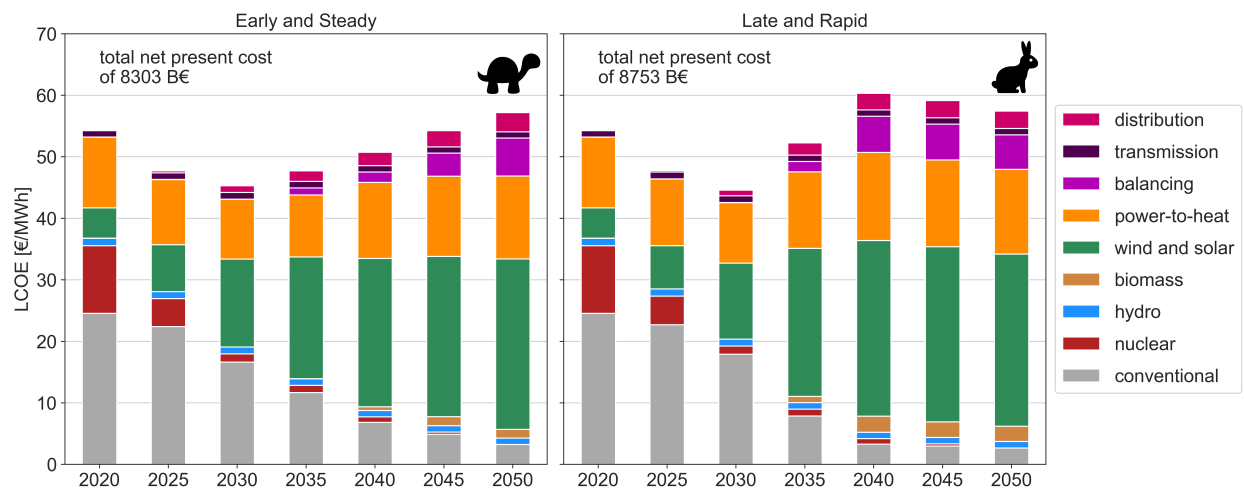
Supplementary Figure 20: Levelized Cost of Energy (LCOE) for the European electricity, heating and transport system throughout transition paths Early and Steady and Late and Rapid. Conventional includes costs associated with coal, lignite, and gas power plants producing electricity as well as costs for fossil-fueled boilers and CHP units. Power-to-heat includes costs associated with heat pumps and heat resistors. Balancing includes costs of electric batteries, H 2 storage, and methanation.
