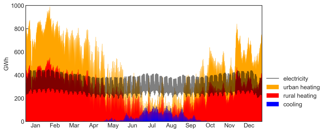
Supplementary Figure 24: Electricity, rural and urban heating, and cooling demands for Europe.
