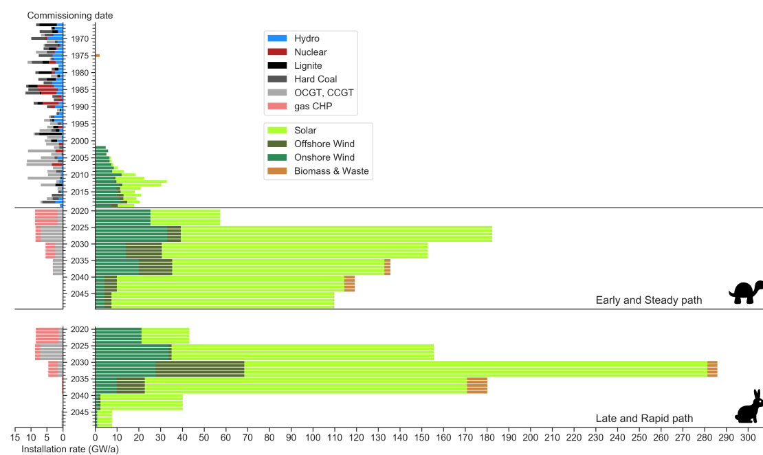
Supplementary Figure 22: Age distribution of European power plants in operation [3, 6] and required annual installation throughout the Early and Steady and Late and Rapid paths when the electricity, heating and transport sectors are included. .
