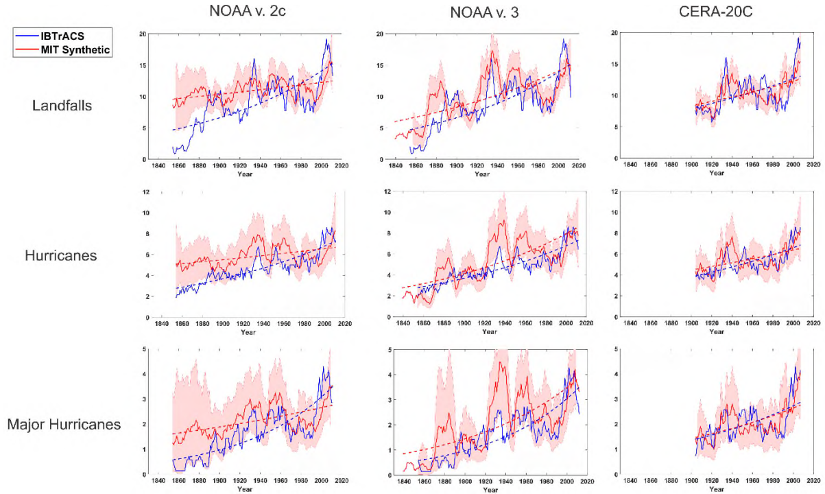
Figure 1: Time series of North Atlantic landfall events (top row), basin hurricanes (middle row) and major hurricanes (bottom row). The landfall frequency includes only storms whose lifetime maximum winds speeds exceed 40 kts ( 21 \text{ ms}^{-1} ). Red curves show quantities associated with tropical cyclones downscaled from three global climate reanalyses (left to right) and blue curves are derived from uncorrected historical tropical cyclone (IBTrACS) data. All quantities have been smoothed with a 7-year running mean. The downscaled counts have been multiplicatively rescaled to match the mean of the last 50 years of the historical data. The dashed curves show the Poisson regressions of the downscaled and historical data. The shading around the downscaled counts shows the bounds within which 90% of subsamples of the downscaled data lie, with the subsample size equal to the historical counts.
