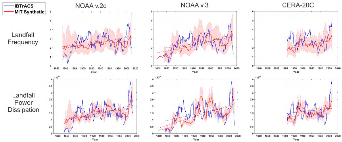
Figure 2: As in Figure 1 but showing the continental U.S. annual landfall frequency (top row) and U.S. landfall power dissipation index ( \text{m}^3\text{s}^{-3} ; bottom row). The landfall frequency includes only storms whose lifetime maximum winds speeds exceed 40 kts ( 21 \text{ ms}^{-1} ). The linear regression lines in the bottom row are from ordinary linear regression.
