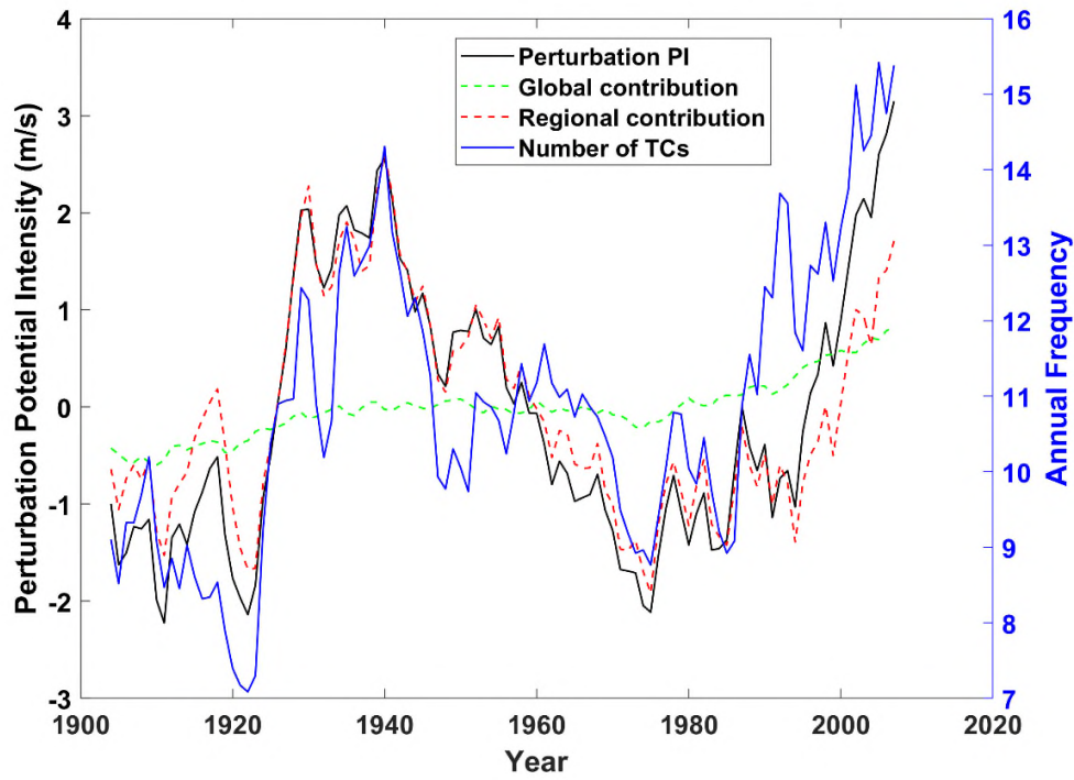
Figure 4: 7-year running means of Atlantic Main Development region (6-18 N, 20-60 W) August-October departures of potential intensity (black, \text{ms}^{-1} ) from its mean over the record, and its decomposition into global (dashed green) and regional (dashed red) components. The 7-year running mean of the annual frequency of tropical cyclones downscaled from CERA-20C is shown in blue (right axis).
