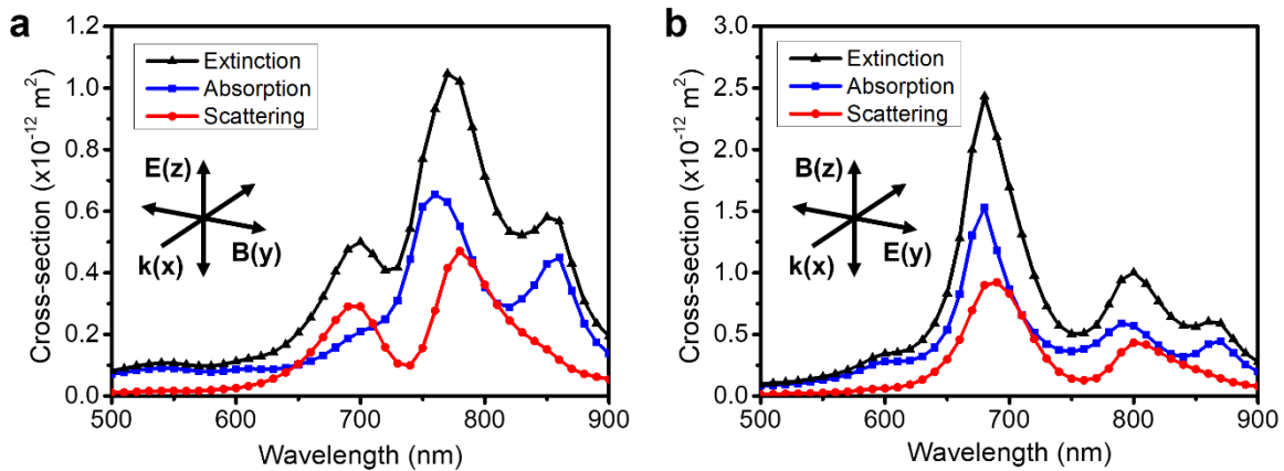
Supplementary Figure 7. Calculated optical extinction of Au dual-rim NFs under an electric field with different oscillating field directions. Simulated absorption, scattering, and extinction spectra under an electric field of light oscillating along the (a) z-axis and (b) y-axis.
