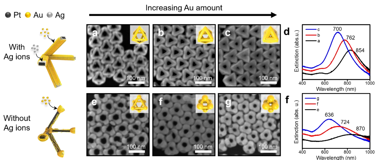
Supplementary Figure 2. The effect of Ag precursors during the well-faceted growth of Au octahedral mono-rim NFs. (a-c) FE-SEM images of Au octahedral mono-rim NFs with different gap distances as the amount of Au increases under the presence of Ag ions (well-faceted growth) and (d) corresponding UV-vis-NIR spectra with sequential blue-shifts of plasmonic bands from 854 to 762 to 700 nm. (e-g) FE-SEM images of Au octahedral tip-blobbed NFs with increasing Au ions without Ag ions and (f) corresponding UV-vis-NIR spectra with plasmonic blue-shifting from 870 to 724 to 636 nm.
