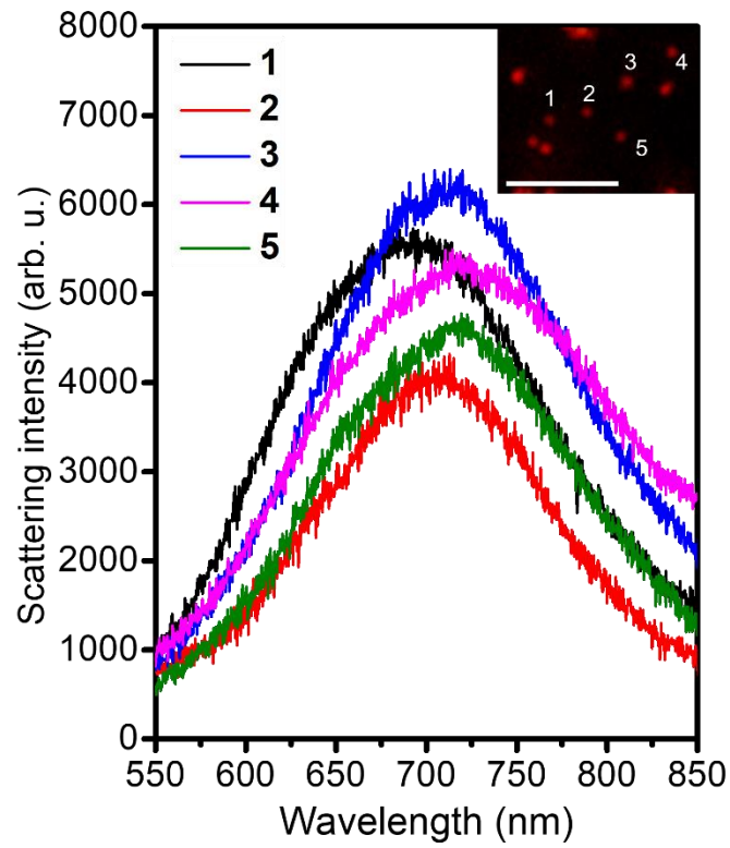
Supplementary Figure 8. Dark-field spectra of Au dual-rim NFs. We obtained dark-field scattering spectra of individual single Au dual-rim NFs and observed that the scattering bands were centered around 695 nm to 720 nm. Inset shows an optical image and each number indicate single Au dual-rim NFs. The scale bar in the inset denotes 1 \mu\text{m} .
