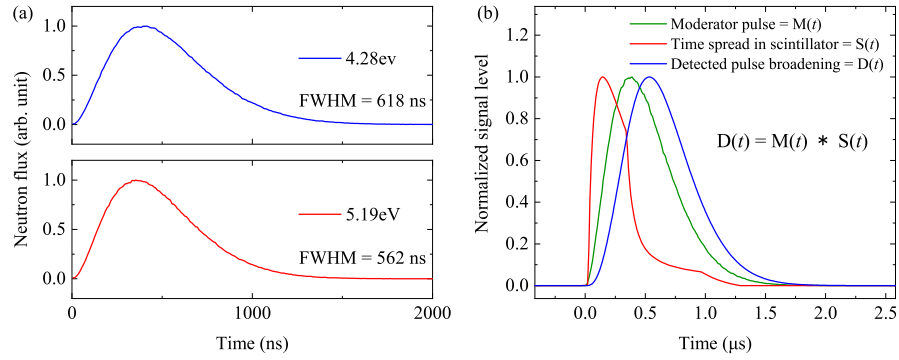
Figure 1: The PHITS simulation of moderated neutron pulse and the evaluated broadening in neutron beamline. (a) Simulated pulse duration for 5.19 eV and 4.28 eV neutrons at the exit of the moderator. (b) Simulated results of pulse broadening at the neutron moderator (green line) and the ^6\text{Li} glass scintillator (red line). The convolved result at the detector at 1.78 m is shown as a blue line.
