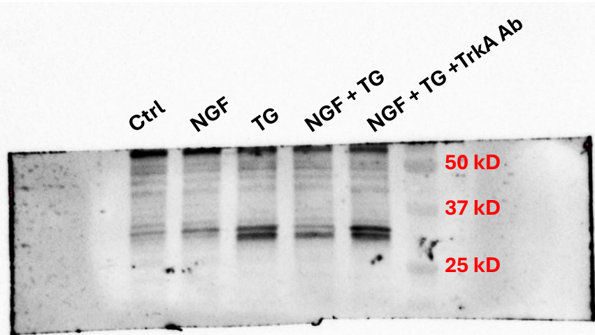
CHOP western blot
