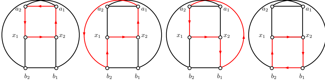
Supplementary Figure 4: The independence complex \Sigma_2 = I(G_2) associated to n = 2 non-interacting qubits. The simplicial complex has 4 independent 1-cycles, corresponding to H_1(\Sigma_2) \cong \mathbb{C}^4 . The four basis states \{|00\rangle, |01\rangle, |10\rangle, |11\rangle\} are indicated in red.
