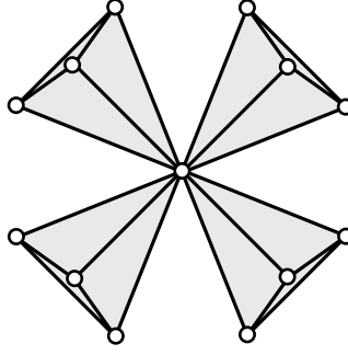
Supplementary Figure 6: Four solid tetrahedra connected at a single mediator vertex m . The base of each tetrahedron is glued to a face in the 2-cycle to be filled in.
