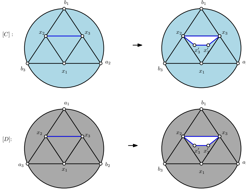
Supplementary Figure 12: The [C] , [D] and [C + D - B] cycles are cut open by cutting a slit in the [x_1x_2x_3] triangle by duplicating the points x_2 and x_3 . Then, the open cycles are connected with each other by gluing through the common one-cycles [x_2x_3] + [x_3x'_2] + [x'_2x'_3] + [x'_3x_2] , ensuring the orientation is consistent. The [C + D - B] cycle is cut open and glued together in the same way - the figure for that cycle is omitted as it is significantly more cluttered than the original cycles.
