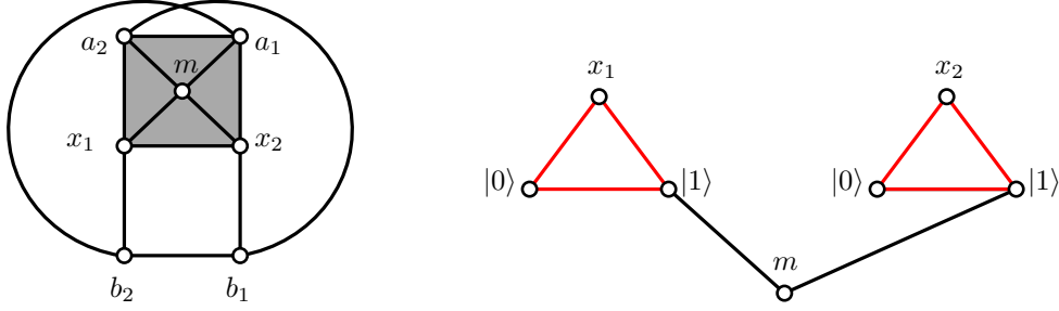
Supplementary Figure 5: Filling in the face |\Psi\rangle bounded by the cycle |00\rangle leads to the simplex \Sigma'_2 , rendering the state |00\rangle a trivial element of homology. This is accomplished by adding the additional vertex m and the 2-simplices [a_1a_2m] , [a_2x_1m] , [x_1x_2m] , and [x_2a_1m] . In the corresponding graph G'_2 shown on the right this amounts to adding a mediator vertex and connecting it as depicted.
