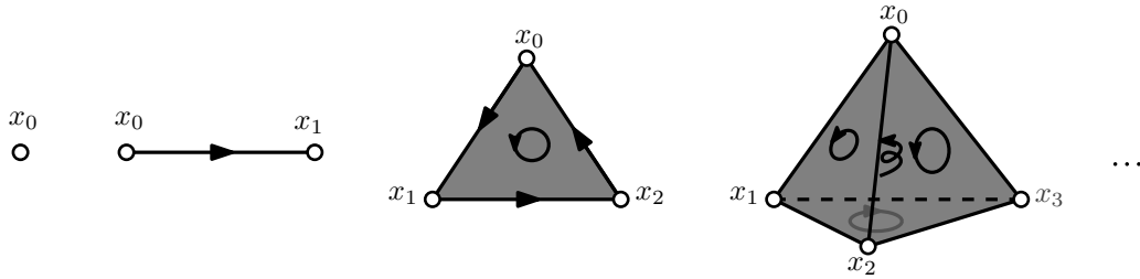
Supplementary Figure 1: Geometric representation of a 0-simplex, oriented 1-simplex, oriented 2-simplex, etc.
