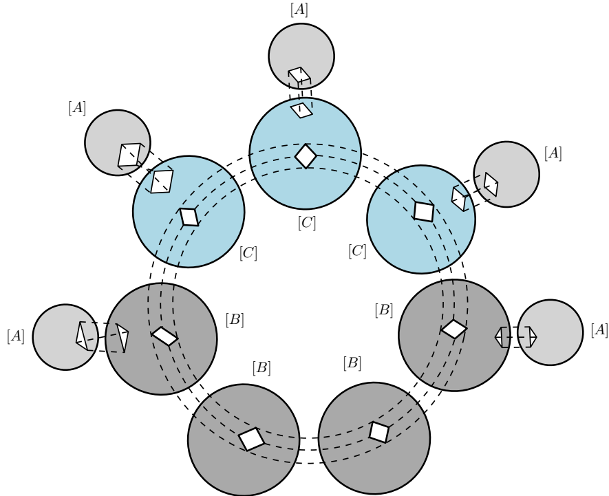
Supplementary Figure 10: The Pythagorean cycle to be filled in is obtained by attaching five copies of [A] which corresponds to the cycle |011\rangle with that face [x_1x_2x_3] missing.
