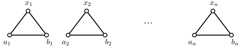
Supplementary Figure 2: A graph G_n representing a system of n disconnected triangles. We will order the vertices (and hence induce an orientation on the simplices in the independence complex) by x_i > a_i > b_i and \alpha_i > \beta_j for i < j and for \alpha, \beta \in \{x, a, b\} .
