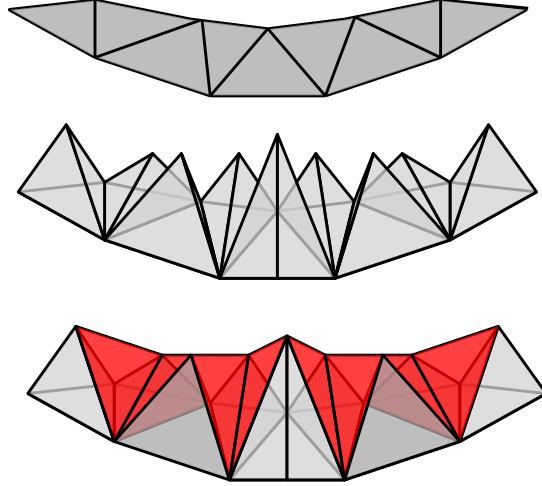
Supplementary Figure 8: General approach to filling a 2-dimensional cycle. The first picture is a part of a 2-dimensional closed surface. For each face [f_i] in the surface we add include a mediator m_i and connect the mediator to all the vertices of [f_i] to form a solid tetrahedron [f_i m_i] . This leaves some empty voids in between the tetrahedra, which are filled by connecting mediators whose corresponding faces share an edge. This leads to a closed shell with an inner void. Finally, choosing one of the mediators to connect to all others fills the void and we obtain a three-dimensional space whose boundary is \sum_i [f_i] , as desired.
