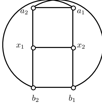
Supplementary Figure 3: The independence complex I(G_2) associated to two disjoint triangles.
