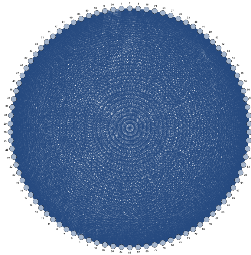
Supplementary Figure 11: The Pythagorean gadget graph G_{Pyth} . The maximum degree of G_{Pyth} is \delta = 81 .
