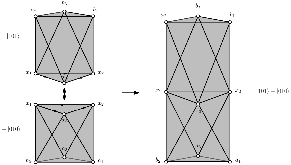
Supplementary Figure 7: Combining the two 2-dimensional voids |101\rangle and -|010\rangle into the 2-dimensional void bounded by the entangled state |101\rangle - |010\rangle . Note that the face [x_1x_2x_3] is common to both cycles but comes with opposite orientations and thus cancels in the superposition, leaving only one void to be filled. Additional vertices and edges which are not relevant have been omitted for clarity.
