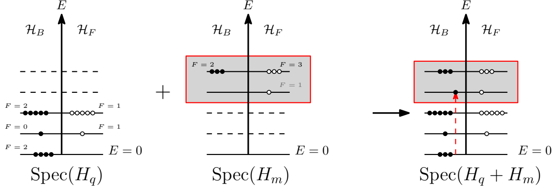
Supplementary Figure 18: Lifting a single SUSY ground state by introducing a mediator vertex connecting to two triangles as in eq. (120). H_q is a supersymmetric Hamiltonian, so all non-zero eigenvalues are paired up. The Hamiltonian H_m is not supersymmetric, and includes unpaired non-zero eigenvalues. When the two Hamiltonians are added together an unpaired eigenvalue from H_m can pair up with a zero eigenvalue from H_q , lifting one state from the SUSY groundspace, as desired.
