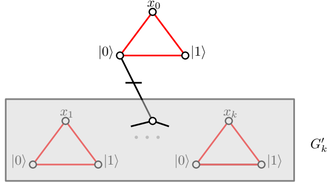
Supplementary Figure 14: The qubit 0 at the top realizes the 1-qubit projector |1\rangle\langle 1| and the bottom gadget G'_k implements \Pi^{(k)} . Connecting them as in the figure implements the (k+1) -qubit projector \Pi^{(k+1)} = |1\rangle\langle 1| \otimes \Pi^{(k)} .
