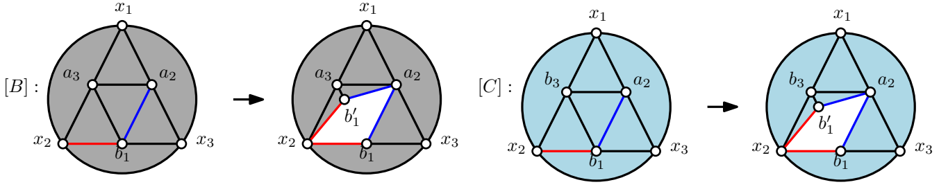
Supplementary Figure 9: The [B] and [C] cycles are cut open by cutting a slit along [x_2b_1] + [b_1a_2] by duplicating the middle point b_1 . Here we have omitted vertices and edges to keep the pictures clear but one should bear in mind that before performing the cut each is a closed 2-cycle, homeomorphic to S^2 . Then, the open cycles are connected with each other by gluing through the common one-cycles [x_2b_1] + [b_1a_2] + [a_2b'_1] + [b'_1x_2] , ensuring the orientation is consistent, and attaching the [A] -cycles by deleting the common face [x_1x_2x_3] . The resulting space, A_5B_4C_3 is a closed surface composed of the [B] and [C] cycles with the five [A] -cycles attached, as shown in Fig. 10. As a whole, the space A_5B_4C_3 is homeomorphic to S^2 and it is this topological S^2 which we wish to fill.
