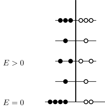
Supplementary Figure 17: The spectrum of supersymmetric quantum mechanics. Black dots represent bosonic states and white ones fermionic states. All states with E > 0 come in boson/fermion pairs. Supersymmetric ground states ( E = 0 ), if there are any, are not necessarily paired.
