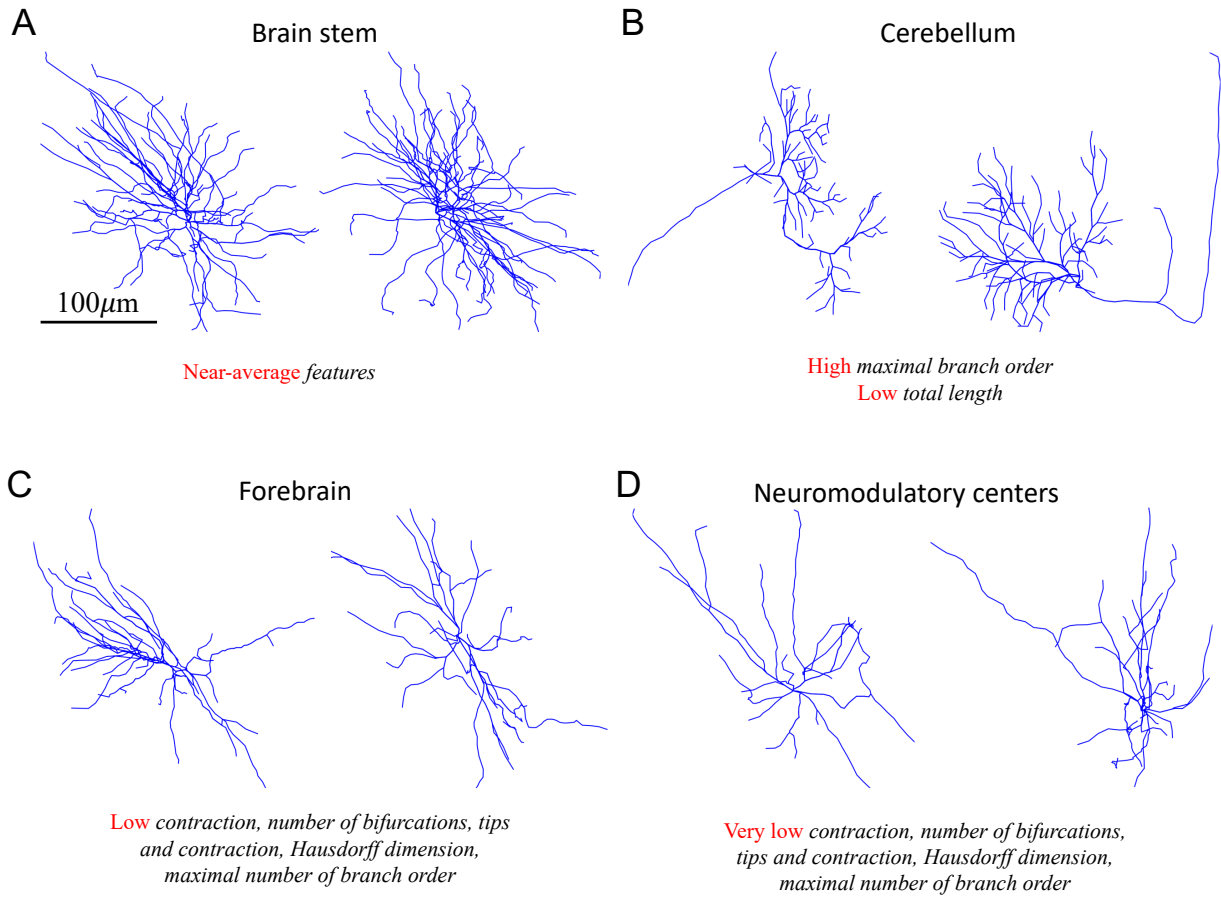
Supplementary Figure S15. Representative neurons for brain stem, cerebellum, forebrain and neuromodulatory centers. Sagittal views of the local morphologies of two representative neurons for each brain area are displayed. The most discriminative L-Measure Vaa3D features for each area are summarized below the examples. Scale bar: 100 µm.
