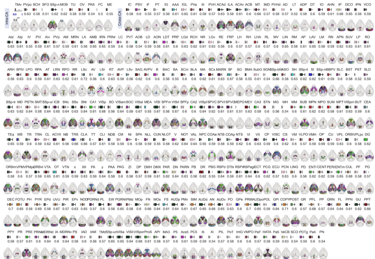
Supplementary Figure S13. Correlated region sets for 313 brain regions. Horizontal projections on the CCFv3 template of regions with a Spearman correlation coefficient of at least 0.5 with the target region (specified at the top of each brain image). The box plot on the top of each brain image is the distribution of the pairwise correlations between these regions and the target region, with the box colored by compound areas (CA) as in Figure 2A. An intra-CA region set contains only regions from the same compound area, while cross-CA set contains regions from at least two different compound areas.
