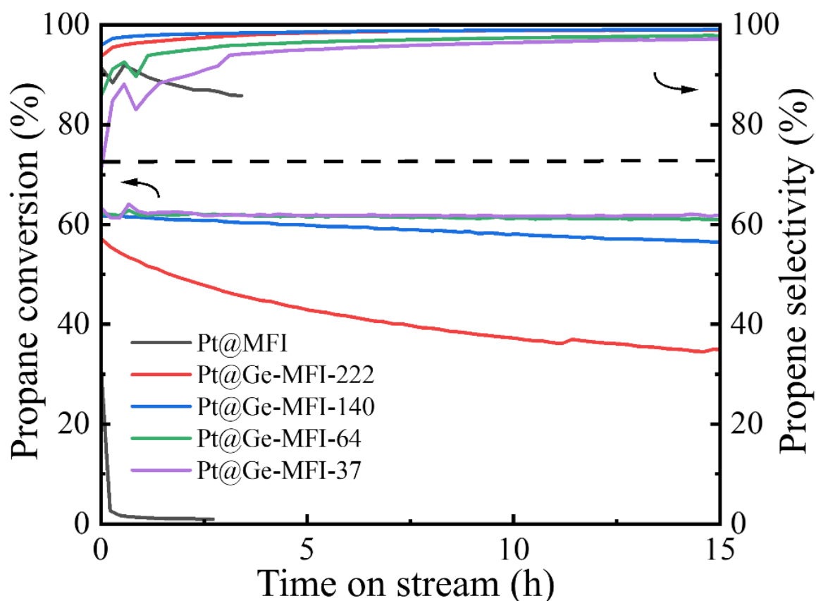
Figure S6. The catalytic performance of Pt@Ge-MFI catalysts with various Si:Ge ratios, which are indicated as suffixes in the sample names. The catalysts were pre-treated in \text{H}_2 flow for 4 hours, and the PDH reaction was carried out under the condition of \text{WHSV}_{\text{propane}} = 1.75\text{h}^{-1} , propane/ \text{N}_2 = 1/3 , 873 K and atmospheric pressure.
