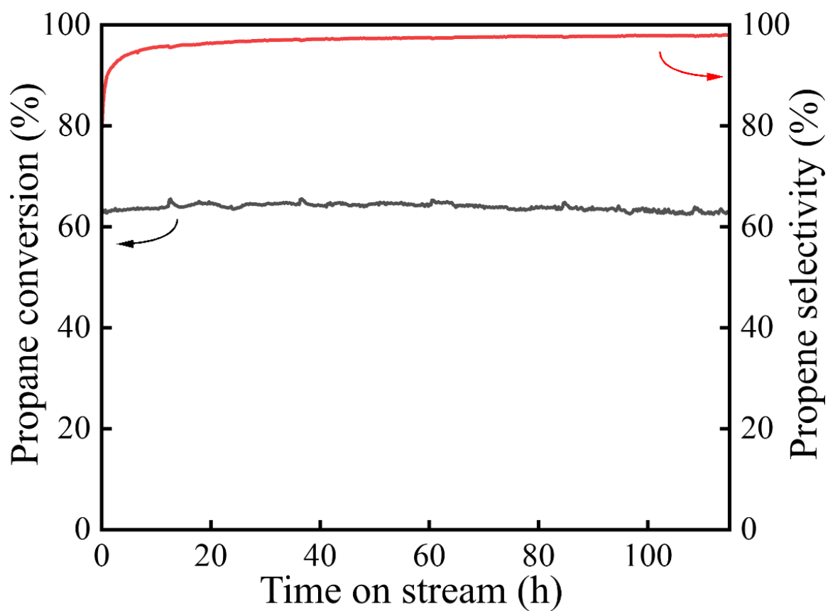
Figure S13. The catalytic performance of Pt@Ge-MFI under the condition of \text{WHSV}_{\text{propane}} = 1.75 \text{ h}^{-1} , \text{propane}/\text{N}_2 = 1/3 , 873 K and atmospheric pressure.
