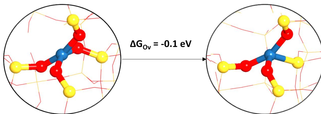
Figure S17. The scheme of oxygen removal of [PtO 4 ] in pure silica MFI zeolite framework.
