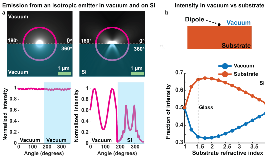
Supplementary Figure 41: Emission profiles from isotropic emitters on different surfaces. (a) Emission profile of an isotropic emitter placed in vacuum and at the Si-vacuum interface. (b) Fraction of intensity emitted into vacuum and the substrate for different refractive indices of the substrate. For analysis in (b), only the real part of the refractive index was considered. Simulations were performed using Lumerical FDTD. Source data are provided as a Source Data file.
