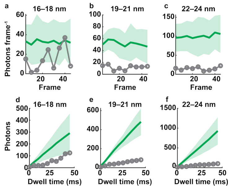
Supplementary Figure 36: Electobleaching of NaDyF 4 LNPs. (a–c) Photons frame -1 collected from NaDyF 4 for three different LNP diameters. Photons frame -1 obtained from NaGdF 4 are also shown for a comparison (gray). Images had an effective beam dwell time of 5 ms. (d–f) Cumulative photons collected from NaDyF 4 LNPs in a CL image for different beam dwell times. Images were obtained by summing photons frame -1 shown in (a–c). In (a–f), photons frame -1 correspond to the integrated area under the 2D Gaussian fit to the CL image of LNPs. CL was measured in the Dy 3+ color channel. In (a–f), solid lines and shaded regions correspond to the mean and standard deviation of the data. Source data are provided as a Source Data file.
