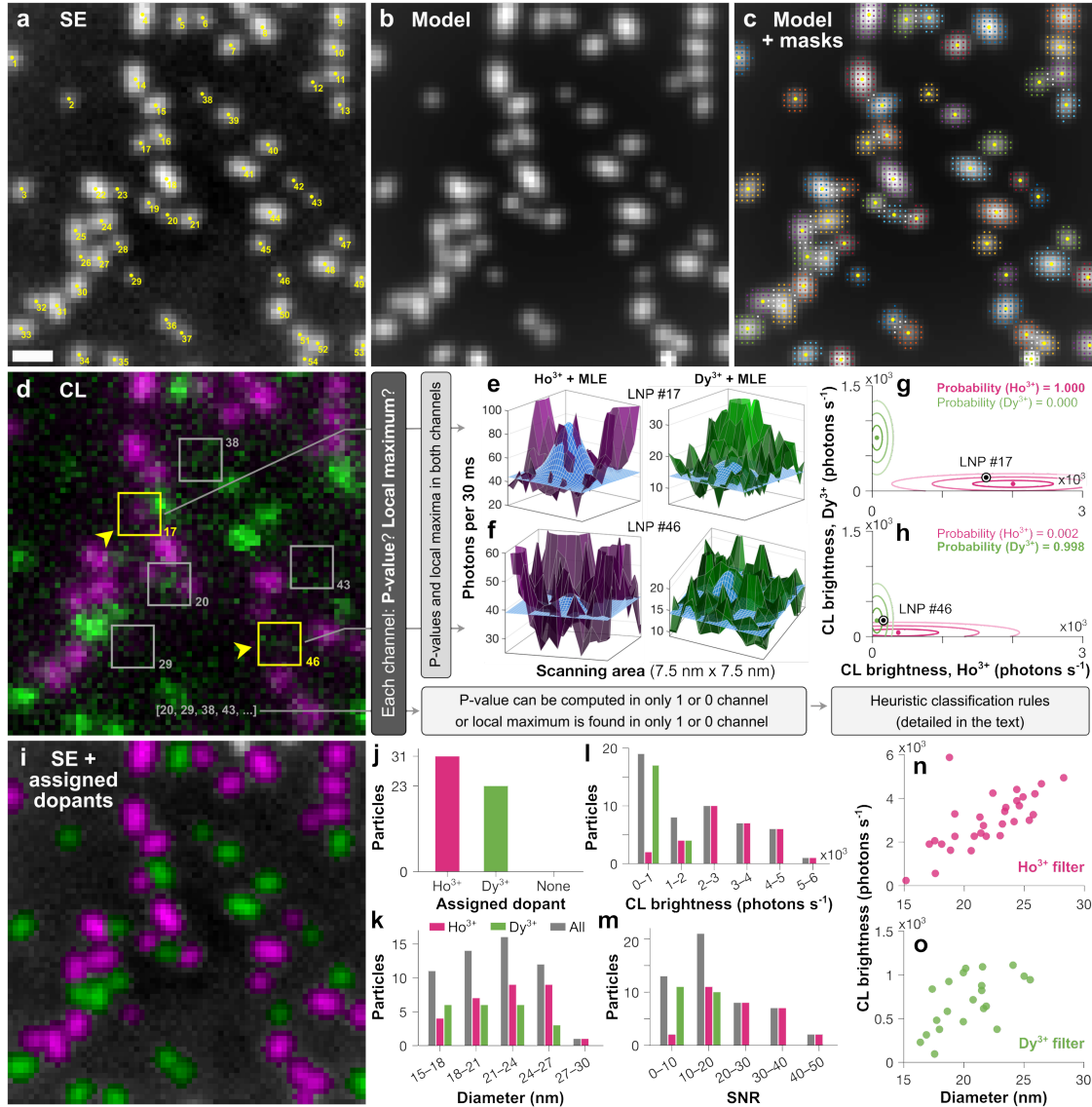
Supplementary Figure 19: Automated dopant assignment in multicolor samples. (a) SE image containing \text{NaHoF}_4 and \text{NaDyF}_4 LNPs (identical to Fig. 3g) with numerical identifiers overlaid. (b) Model for the SE image in (a), in which each LNP is represented as a bivariate Gaussian distribution and the background as a quadratic surface. (c) LNP-specific masks (small color dots) and centers (large yellow dots) obtained from, and overlaid on, (b). Pixels shared between two or more LNPs are excluded from all masks (white dots). (d) CL image showing overlaid \text{Ho}^{3+} and \text{Dy}^{3+} channels (identical to Fig. 3h). The yellow boxes highlight the two LNPs (#17 and #46) whose probabilistic dopant assignment analyses are detailed in (e-h). The yellow arrowheads indicate the viewing angles used in (e,f). Gray boxes show LNPs whose dopants were assigned by heuristic classification. (e,f) Estimation of CL detection rates. CL signal in the \text{Ho}^{3+} (left, magenta) and \text{Dy}^{3+} (right, green) channels for LNPs #17 (e) and #46 (f), and associated bivariate Gaussian distributions (blue) resulting from MLE of the CL signal under the LNP-specific masks. (g,h) Bayesian probabilistic dopant assignment. The estimated CL detection rates of LNPs #17 (g) and #46 (h) (bull's-eyes) are compared to our model trained on single-LNP datasets (ellipses and dots; magenta, \text{NaHoF}_4 ; green, \text{NaDyF}_4 ). The concentric ellipses represent the 1- \sigma , 2- \sigma , and 3- \sigma levels of the bivariate Gaussian distributions modeling the CL detection rates in the trained model. The color dots are the expected values. We assigned to each LNP the dopant with the greatest posterior probability. (i) SE image colored according to assigned dopant (magenta, \text{Ho}^{3+} ; green, \text{Dy}^{3+} ). (j-m) Multicolor sample characterization (also see Supplementary Table 1). (j) Dopant assignment statistics. (k) Occurrences of LNP diameters. (l,m) Occurrences of estimated LNP CL detection rates (l) and occurrences of SNR (m) in the channel of the assigned dopant. (n,o) CL detection rates in the channel of the assigned dopant as a function of LNP diameter for \text{Ho}^{3+} -doped (n) and \text{Dy}^{3+} -doped (o) LNPs. (a-d, i) Contrast was adjusted. Scale bar: 50 nm. Source data are provided as a Source Data file.
