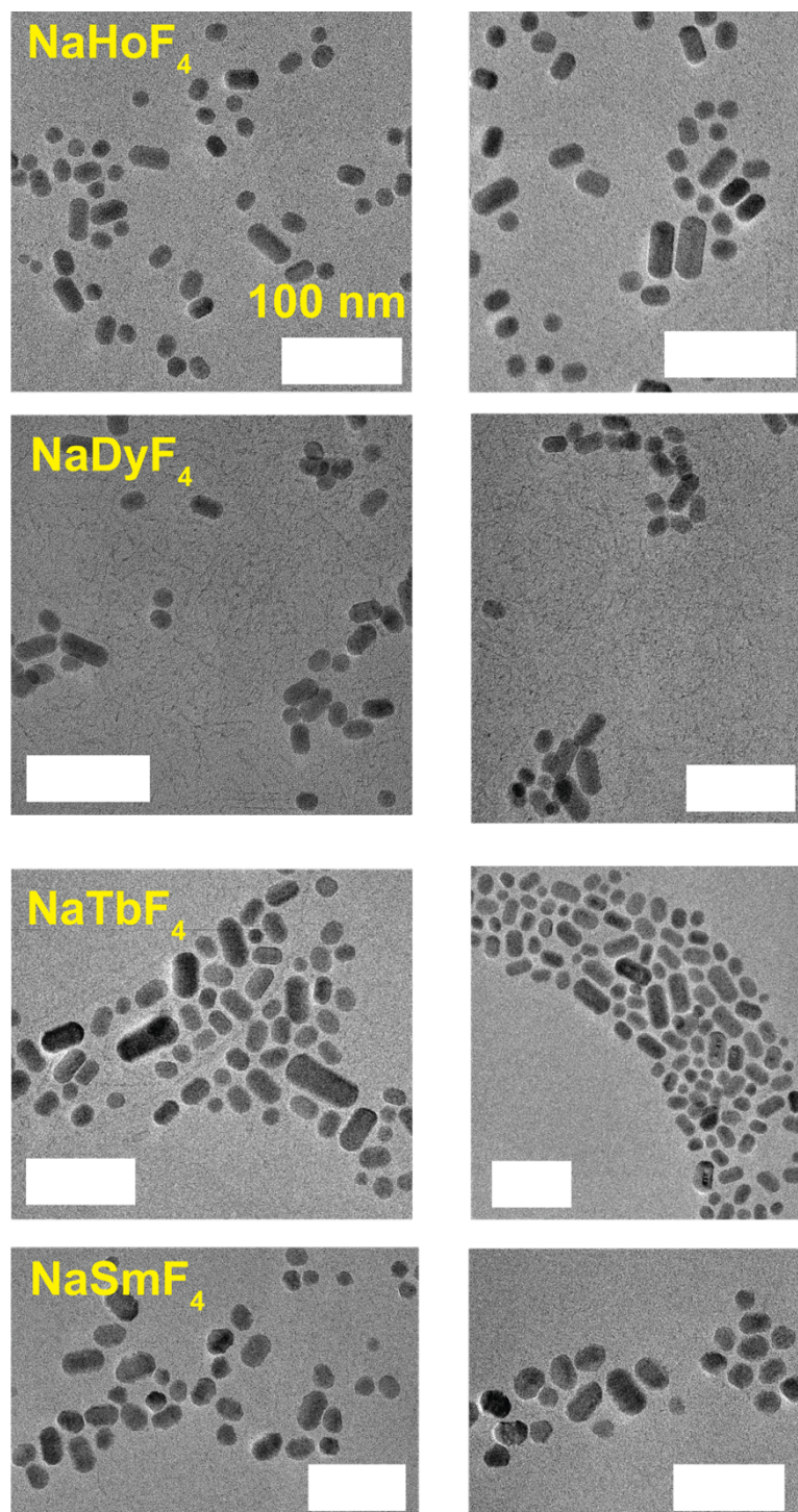
Supplementary Figure 2: TEM imaging of LNP s with 60-min growth step. TEM characterization of NaHoF 4 , NaDyF 4 , NaTbF 4 , and NaSmF 4 LNP s synthesized using a 60-min growth step. Images were acquired at 200 keV beam energy using a JEOL JEM-F200 S/TEM in TEM mode. Scale bars: 100 nm.
