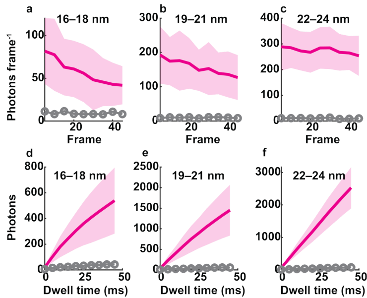
Supplementary Figure 35: Electobleaching of NaHoF 4 LNPs. (a–c) Photons frame -1 collected from NaHoF 4 for three different LNP diameters. Photons frame -1 obtained from NaGdF 4 are also shown for a comparison (gray). Images had an effective beam dwell time of 5 ms. (d–f) Cumulative photons collected from NaHoF 4 LNPs in a CL image for different beam dwell times. Images were obtained by summing photons frame -1 shown in (a–c). In (a–f), photons frame -1 correspond to the integrated area under the 2D Gaussian fit to the CL image of LNPs. CL was measured in the Ho 3+ color channel. In (a–f), solid lines and shaded regions correspond to the mean and standard deviation of the data. Source data are provided as a Source Data file.
