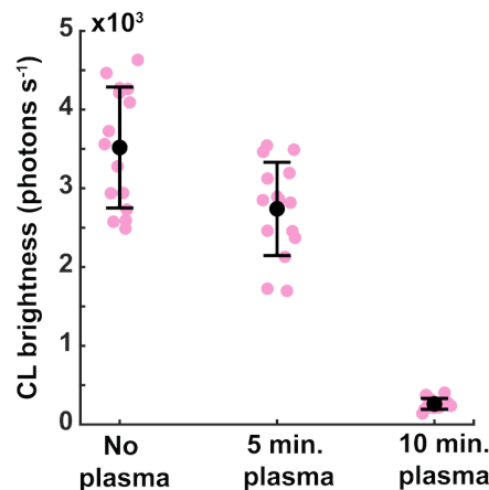
Supplementary Figure 39: Impact of plasma on CL brightness. CL brightness of \text{NaHoF}_4 LNPs under different exposures to plasma. The experiments were performed with a PE-25 plasma cleaner from Plasma Etch, Inc. 15 LNPs were imaged for each condition. Error bars show the mean and standard deviation. Source data are provided as a Source Data file.
