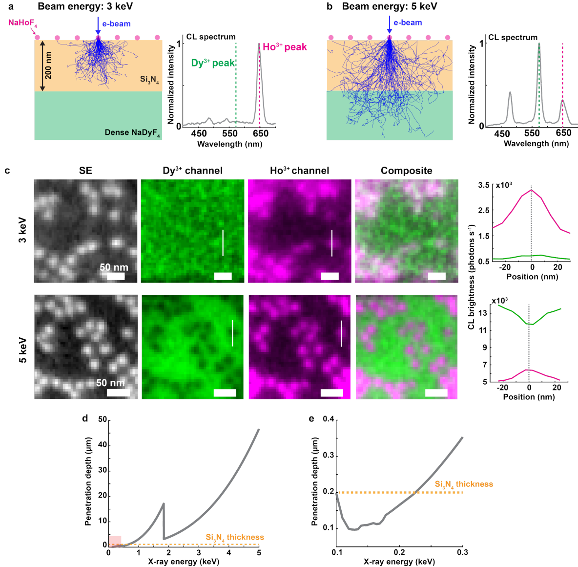
Supplementary Figure 10: Photonic emission from LNP does not cause nonlocal excitation. (a,b) Monte Carlo simulations and measured CL spectra of the sample where sparse (NaHoF 4 ) and dense (NaDyF 4 ) LNP were separated by a 200-nm-thick layer of Si 3 N 4 coated with a 5-nm-thick layer of 80:20 Pt:Pd on its top surface (not shown). (c) Left: SE and CL images acquired from the sample shown in (a,b), at beam energies of 3 keV and 5 keV. Right: Cross-sectional profiles corresponding to the white lines shown in CL images (left). Profiles are shown for both Dy 3+ (green) and Ho 3+ (magenta) channels. (d) Penetration depth of X-rays inside Si 3 N 4 as a function of X-ray energy. (e) Zoom-in of the graph from the shaded region in (d) over 0.1 to 0.3 keV. Dotted lines in (d,e) highlight the thickness of Si 3 N 4 used. Source data are provided as a Source Data file.
