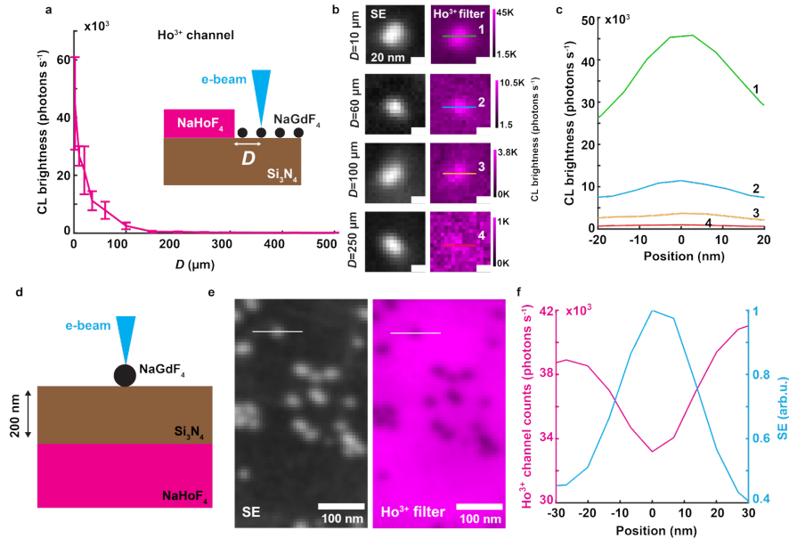
Supplementary Figure 13: Nonlocal excitation on Si 3 N 4 substrate. (a) CL signal in the Ho 3+ channel from NaGdF 4 LNPs on Si 3 N 4 at different distances, D , from the dense layer of NaHoF 4 LNPs. (b) CL images of NaGdF 4 LNPs at different distances from the layer. (c) Cross-sectional profiles of LNPs from (b). (d) A schematic of imaging NaGdF 4 LNPs on a 200-nm-thick Si 3 N 4 window coated with a 5-nm-thick layer of 80:20 Pt:Pd on its top surface (not shown). Dense NaHoF 4 LNPs were deposited on the opposite, lower side. A beam energy of 5 keV was used to penetrate through the Si 3 N 4 layer and excite the NaHoF 4 LNPs ( Supplementary Figure 10 ). (e) SE and CL images of the setup in (d). (f) Cross-sectional profiles of a particle marked in (e). In (a) three LNPs were imaged at each D . Error bars show mean and standard deviation. Source data are provided as a Source Data file.
