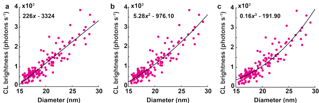
Supplementary Figure 33: Comparison of linear and nonlinear fits to CL vs. LNP size data. (a) Linear ( r = mx + b ), (b) quadratic ( r = mx^2 + b ), and (c) cubic ( r = mx^3 + b ) fits to the CL brightness vs. LNP diameter for NaHoF 4 LNPs in the Ho 3+ channel. r is CL brightness in photons s -1 , x is the diameter of LNPs in nm, b is the y -intercept in photons s -1 , m is the co-efficient of x in (a) photons s -1 nm -1 , (b) photons s -1 nm -2 , and (c) photons s -1 nm -3 . Note that the factor 10 3 in the y -axis was included in all fits.
