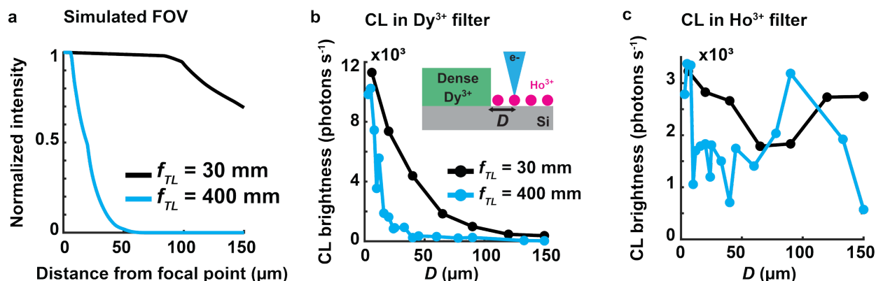
Supplementary Figure 8: Nonlocal excitation and field of view (FOV) of the parabolic mirror. (a) Simulation of light captured from a point source on a PMT of 5 mm diameter (matched to the PMTs used in this work). The point source was imaged at different distances from the focal point of the parabolic mirror for two different focal lengths of the tube lens (lenses placed in front of the PMTs in Supplementary Figure 6 ). The intensity was obtained by ray tracing and served as a measure of the FOV of the CL imaging system. The FOV had >150 \mu m radius for the 30 mm focal length tube lens, which was reduced to \approx 25 \mu m for the 400 mm focal length tube lens. (b,c) Edge experiment with dense NaDyF 4 and sparse NaHoF 4 LNPs. Sparse NaHoF 4 LNPs were imaged at different distances from the dense region's edge. CL in Dy 3+ and Ho 3+ color channels are shown in (b) and (c), respectively. Source data are provided as a Source Data file.
