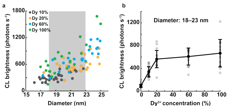
Supplementary Figure 5: CL brightness and dopant concentration. (a) Brightness of LNPs in the \text{Dy}^{3+} channel as a function of size for different dopant concentrations. At least 25 LNPs were imaged for each condition. (b) Brightness of LNPs of sizes between 18 and 23 nm as indicated by the shaded region in (a). Brightness is plotted as a function of dopant concentration. Different dopant concentrations were achieved by mixing \text{Dy}^{3+} ions with \text{Y}^{3+} ions, except for 0% \text{Dy}^{3+} , which shows emission of \text{NaGdF}_4 ions in the \text{Dy}^{3+} channel. Error bars in (b) show mean and standard deviation of 18, 20, 17, 12, and 14 LNPs, for dopant concentrations of 0%, 10%, 20%, 60%, and 100% respectively. Source data are provided as a Source Data file.
