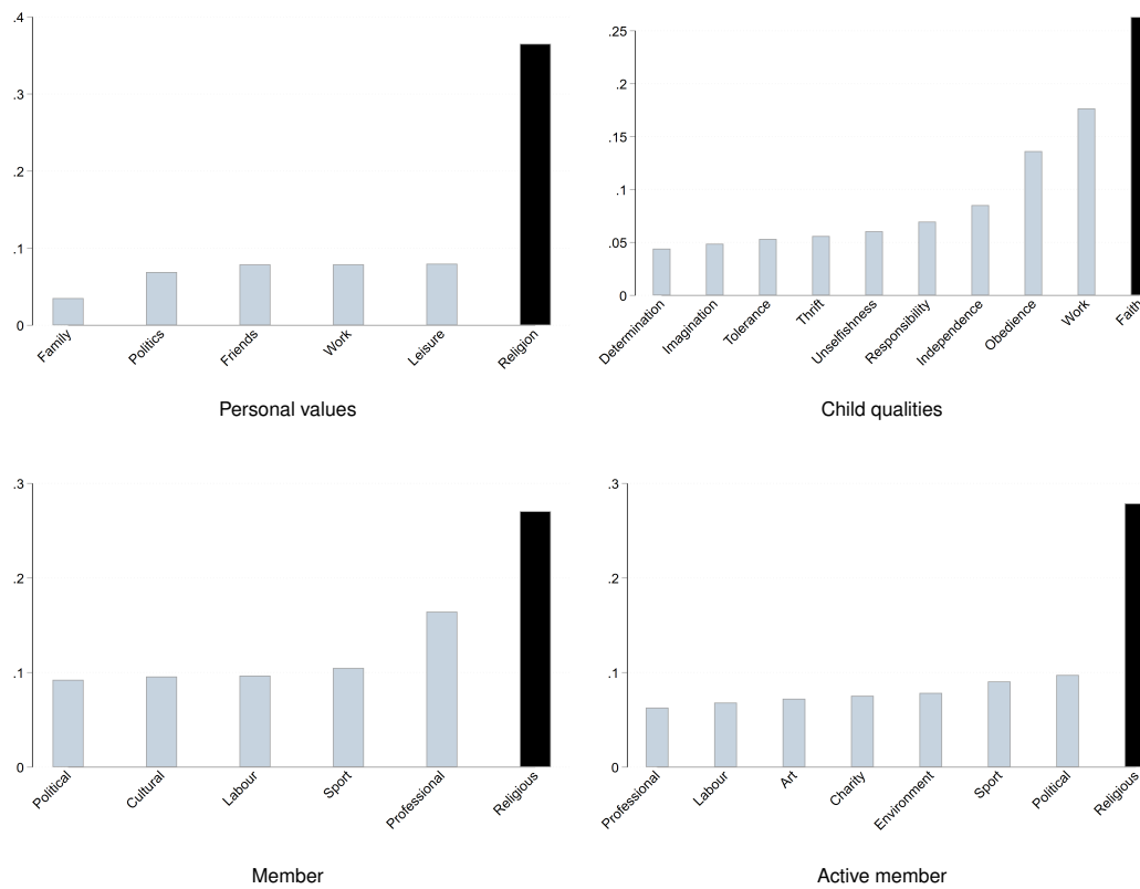
Fig. S16. CF_{st} across countries, controlling for income levels. Note: Each cultural dimension is regressed on 10 dummies for respondents' income level before computing CF_{st} across countries. The samples used are the same as in the left panels of Fig. 1. Code to reproduce the figure is provided in Harvard Dataverse. Result: Religious values continue to dominate global diversity when comparing individuals within the same income group.
