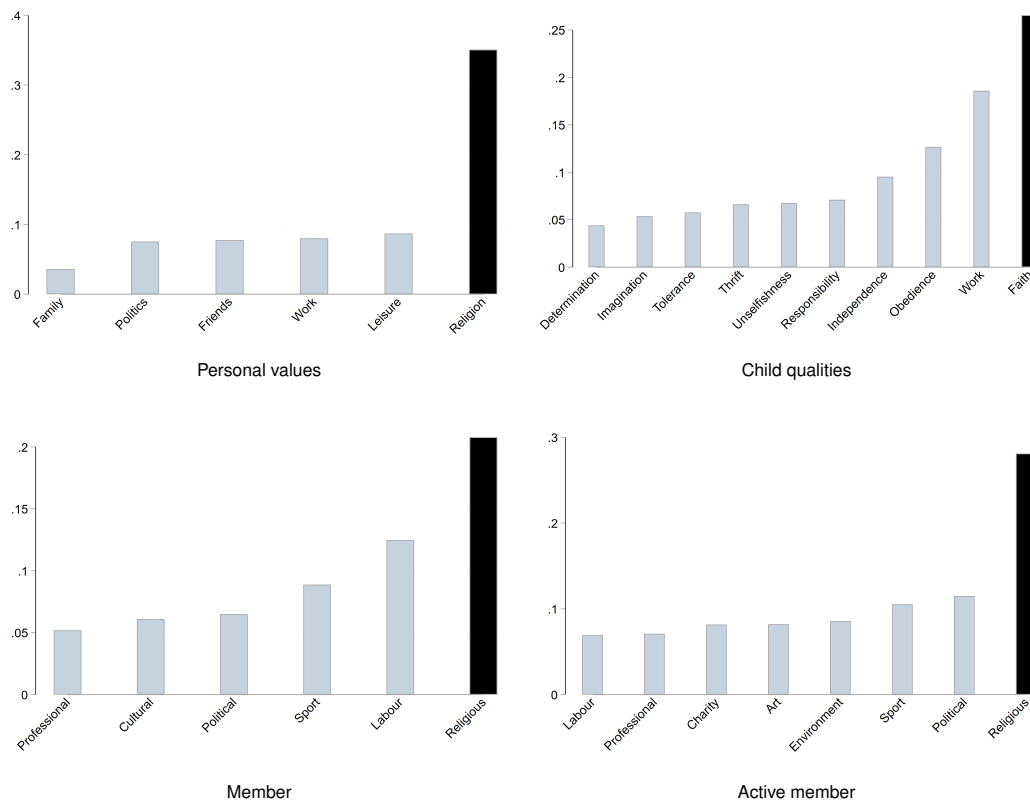
Fig. S15. CF_{st} across countries, controlling for educational attainment. Note: Each cultural dimension is regressed on 8 dummies for respondents' highest educational attainment before computing CF_{st} across countries. The samples used are the same as in the left panels of Fig. 1. Code to reproduce the figure is provided in Harvard Dataverse.
