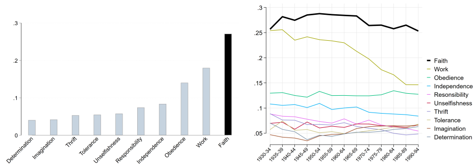
Fig. S17. CF_{st} for Child qualities excluding invalid responses. Note: The left panel shows the diversity across countries based on the full sample, excluding 22,658 respondents who selected more than five values. The right panel shows cohort-based diversity, excluding 18,133 respondents who selected more than five values. Code to reproduce the figure is provided in Harvard Dataverse.
