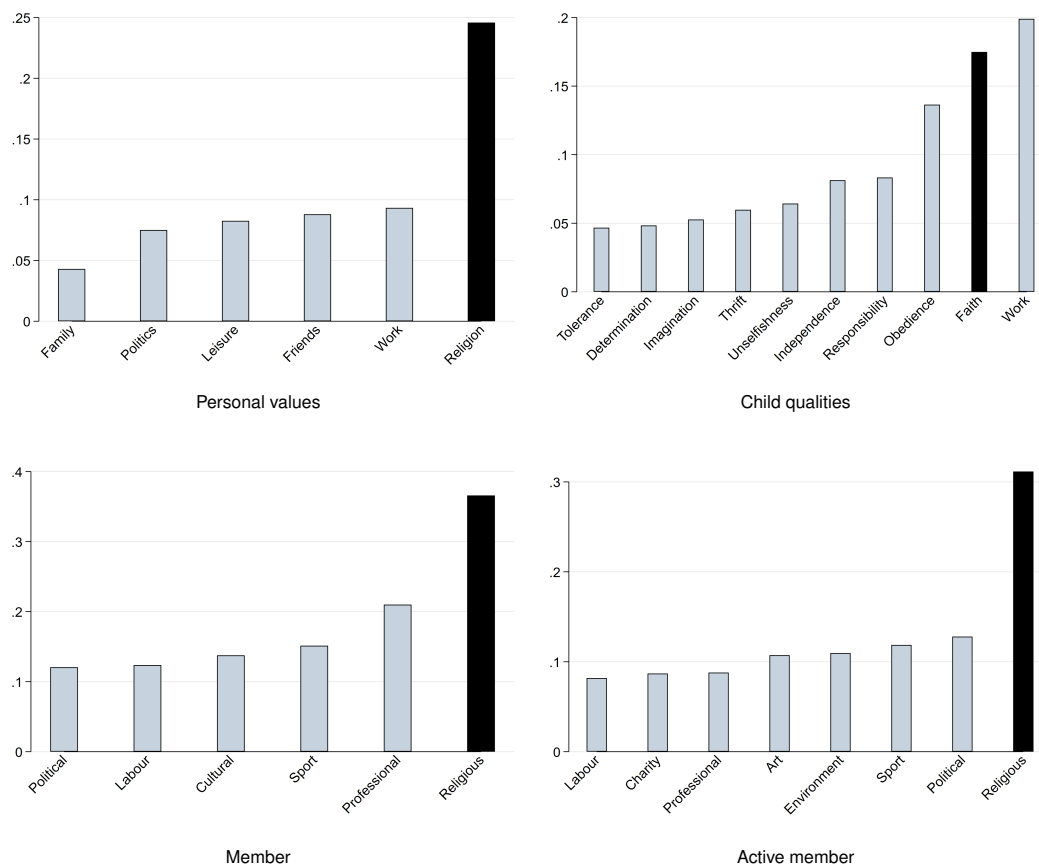
Fig. S12. CF_{st} across countries within denomination: Christianity. Note: CF_{st} is computed within the subsample of respondents who identify as "Christian" (Roman Catholic, Protestant, Orthodox, or Other Christian). Respondent counts are: 308,790 across 104 countries for Personal values , 335,032 across 105 countries for Child qualities , 190,671 across 89 countries for Membership , and 151,893 across 91 countries for Active membership . Code to reproduce the figure is provided in Harvard Dataverse. Result: Religiosity remains the most culturally diverse dimension within Christianity, with the exception of "Hard Work" among Child qualities.
