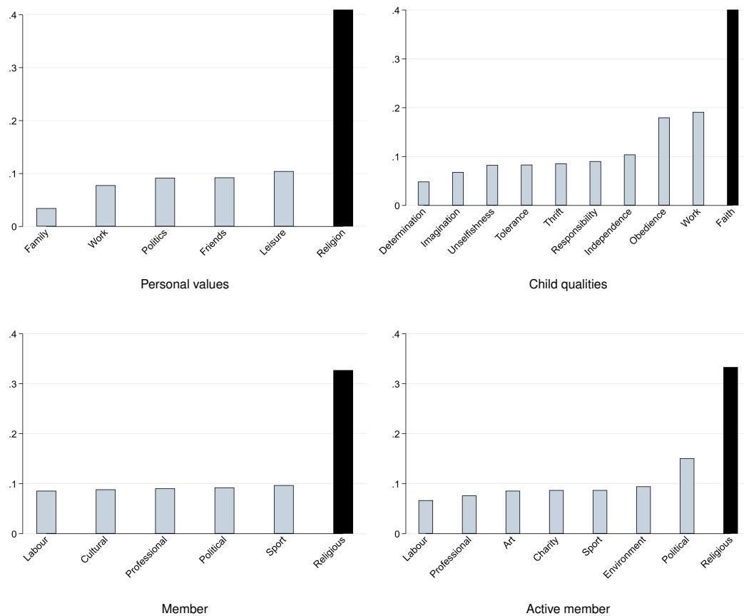
Fig. S11. CF_{st} across countries within denomination: No religion. Note: Each panel shows the cross-country cultural diversity ( CF_{st} ) among respondents who report no religious affiliation ("None"). The number of respondents is 129,066 across 98 countries for Personal values , 137,187 across 99 countries for Child qualities , 89,692 across 88 countries for Membership , and 65,543 across 85 countries for Active membership . Code to reproduce the figure is provided in Harvard Dataverse.
