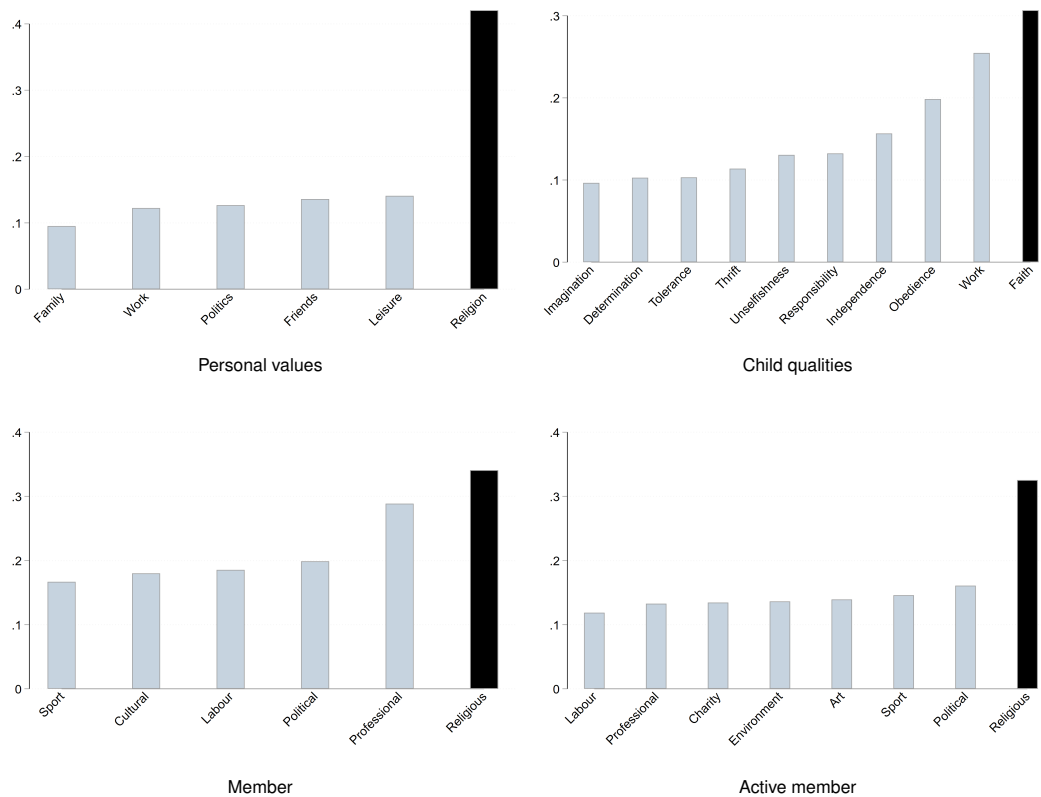
Fig. S4. CF_{st} across sub-national districts, not controlling for country fixed effects. Note: The samples used are the same as in Fig. 2. Code to reproduce the figure is provided in Harvard Dataverse. Result: Religious values continue to dominate global diversity when considering variation across sub-national districts.
