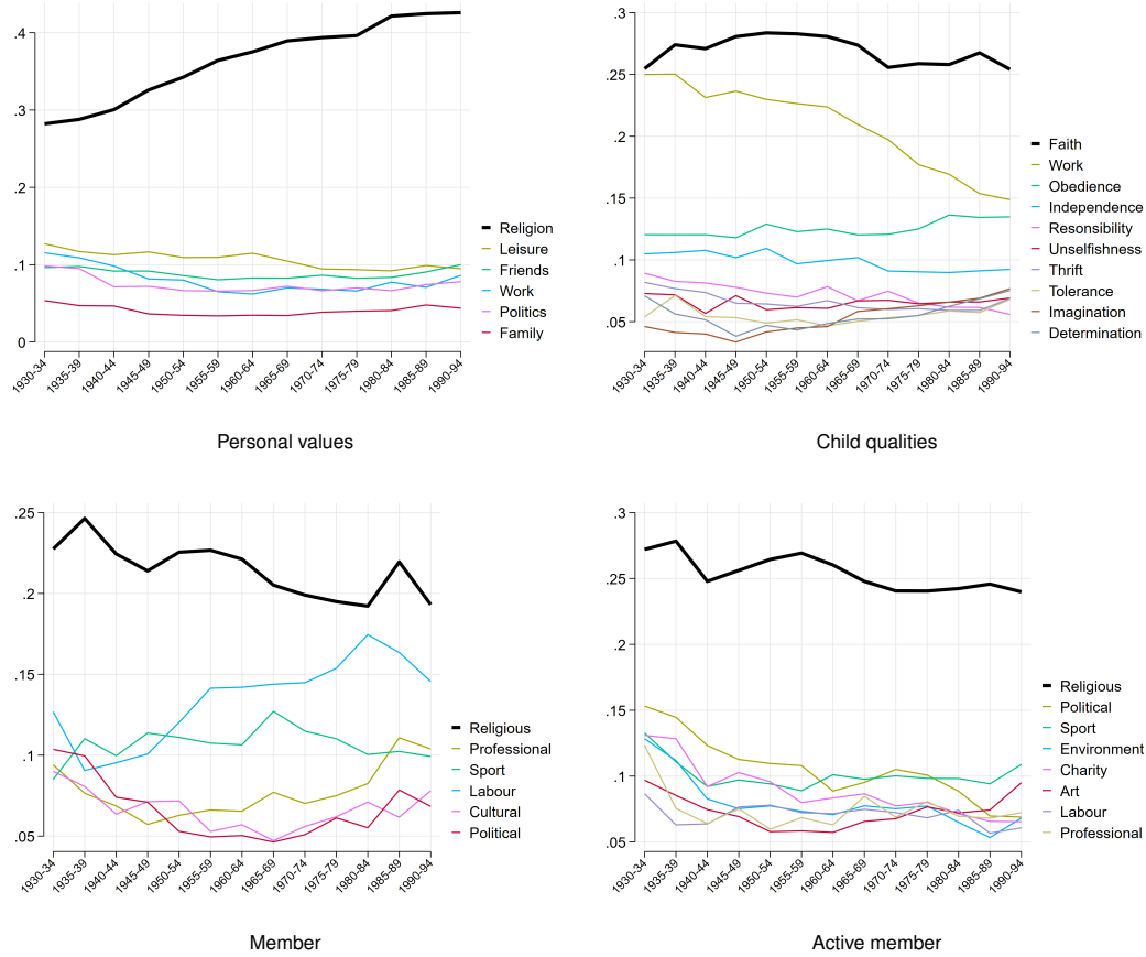
Fig. S5. CF_{st} over time, controlling for age and gender fixed effects. Note: The samples used are the same as in the right panels of Fig. 1. Code to reproduce the figure is provided in Harvard Dataverse.
