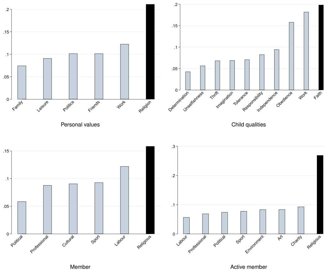
Fig. S14. CF_{st} across countries within denomination: Other religions. Note: CF_{st} is computed within the subsample of respondents who identify as Jewish, Hindu, Buddhist, or Other religion. Respondent counts are: 41,924 across 95 countries for Personal values , 46,579 across 96 countries for Child qualities , 17,399 across 74 countries for Membership , and 30,833 across 70 countries for Active membership . Code to reproduce the figure is provided in Harvard Dataverse. Result: Religiosity remains the most culturally diverse value dimension within this group of non-Christian and non-Muslim denominations.
