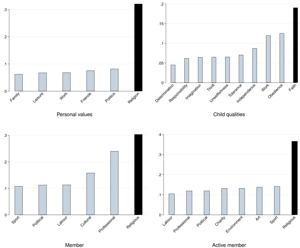
Fig. S13. CF_{st} across countries within denomination: Islam. Note: CF_{st} is computed within the subsample of respondents who identify as "Muslim". Respondent counts are: 109,990 across 82 countries for Personal values , 108,965 across 83 countries for Child qualities , 42,431 across 63 countries for Membership , and 68,541 across 67 countries for Active membership . Code to reproduce the figure is provided in Harvard Dataverse.
