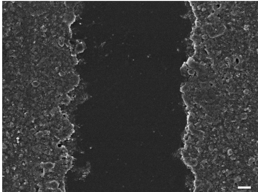
Supplementary Figure 1. SEM image of a device with a channel length of 77\mu\text{m} . The scale bar on the bottom right of the figure corresponds to a length of 10\mu\text{m} .
