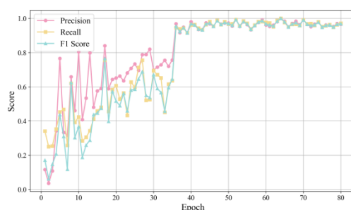
ResNet50-Validation
