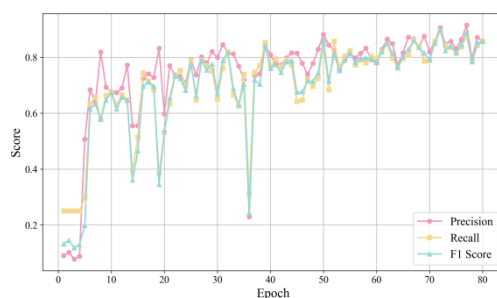
EfficientNet-Validation
