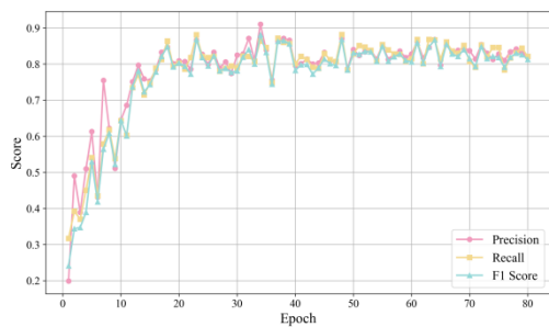
StartNet-Validation
