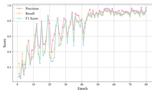
CoAtNet-Validation
