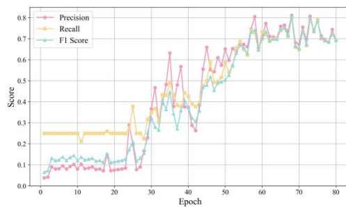
ResMLP-Validation
