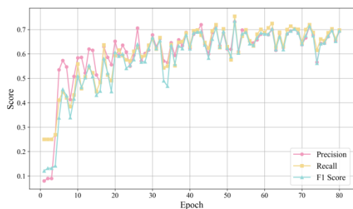
MobileNetV3-Validation
