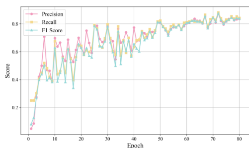
MobileNetV4-Validation
