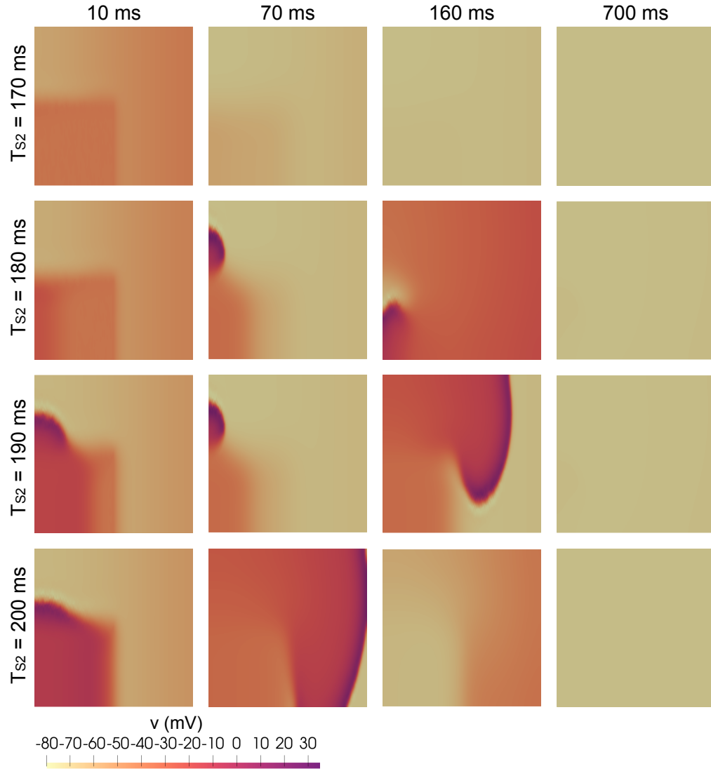
Supplementary Figure 1: Attempts to generate a spiral wave for the bidomain model by varying the timing of the S2 stimulation. Each figure row represents a specific timing of the S2 simulation, T_{S2} , after the S1 stimulation. This S2 timing is reported to the left of the snapshots. The time points displayed above the snapshots report the time when the snapshots are recorded after the S2 stimulation was applied. We observe that none of the considered S2 timings result in a reentrant spiral wave. Note that, as in Figure 2 in the paper, the x -axis of the snapshots has been adjusted to get a square shape.
