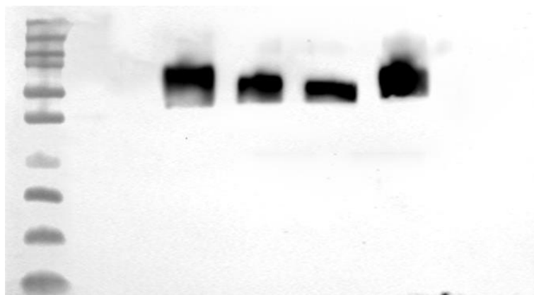
Supplementary Fig 2 The raw scan of western blot showing protein expression of mRNAs encoding different structural domains of RABV-G. The gel lanes from left to right are Protein Marker, Control, RABV-Full, RABV-TE, RABV-E and RABV-R333Q.
