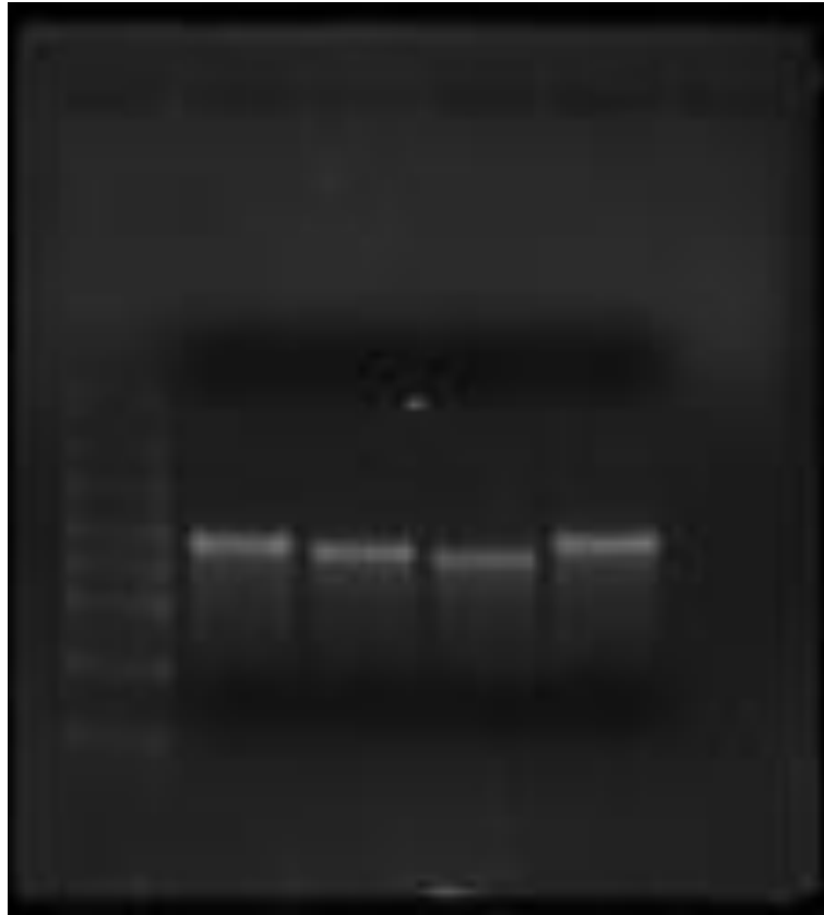
Supplementary Fig 1 The raw scan of agarose gel showing the lengths of mRNAs encoding different structural domains of RABV-G. The gel lanes from left to right are RNA Marker, RABV-Full, RABV-TE, RABV-E and RABV-R333Q.
