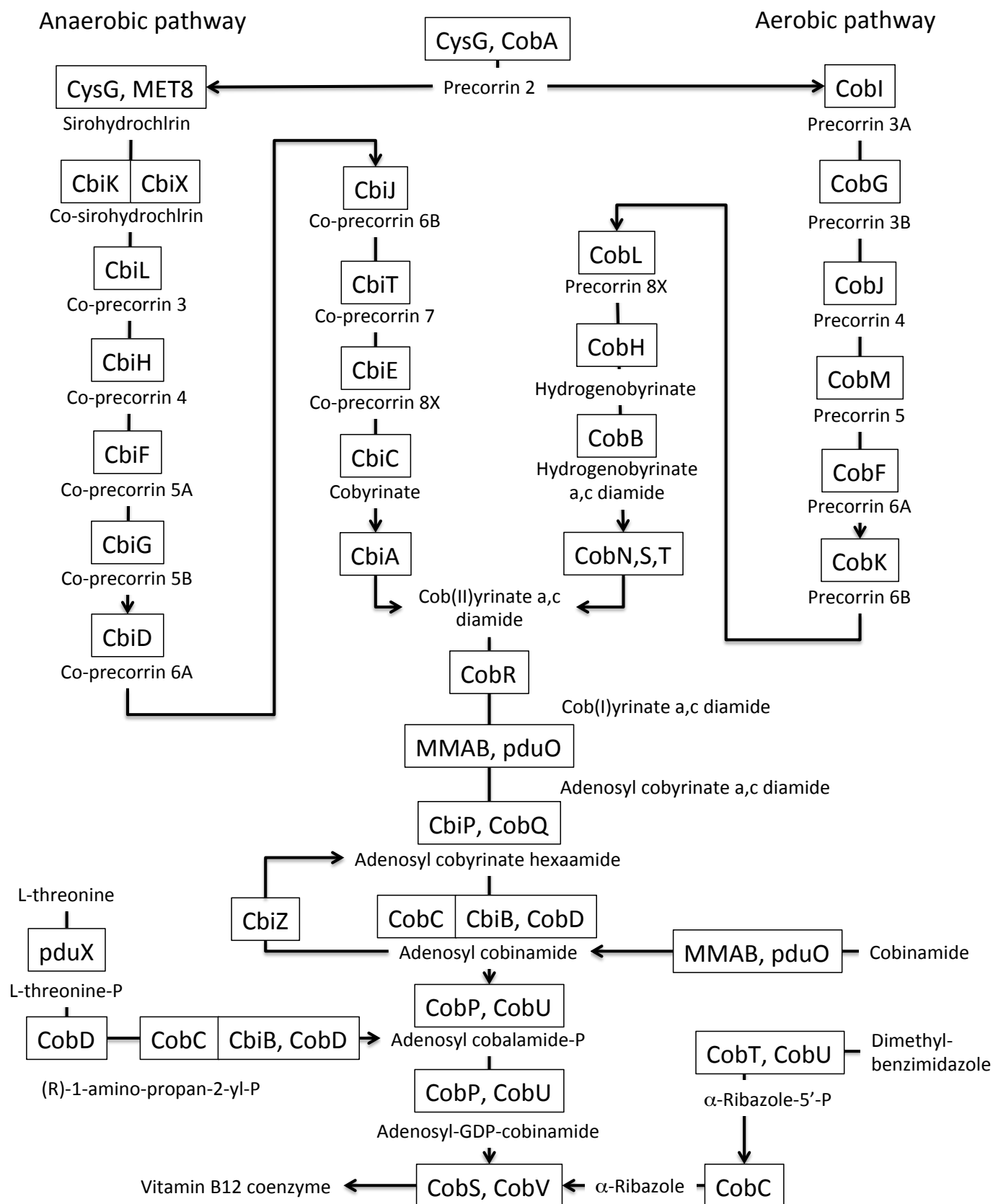
Figure S1. Cobalamin biosynthesis pathways using KEGG gene abbreviations. Both the anaerobic and aerobic pathways are shown
