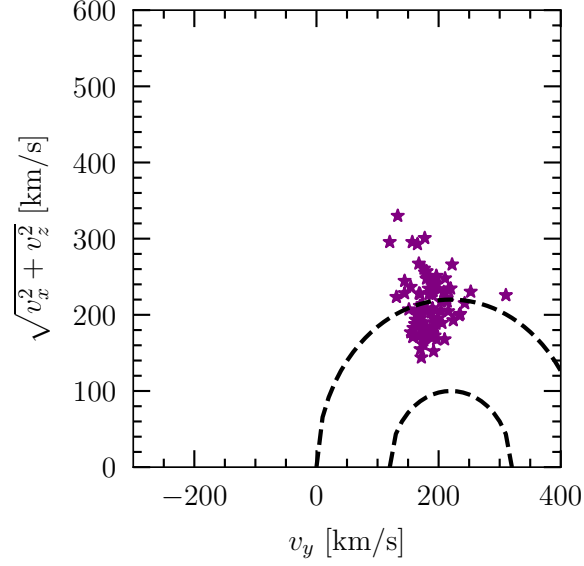
FIG. 1: Toomre diagram for Nyx stars. For reference, the black dashed lines correspond to velocity contours of 100 and 220 km/s in the local frame.
