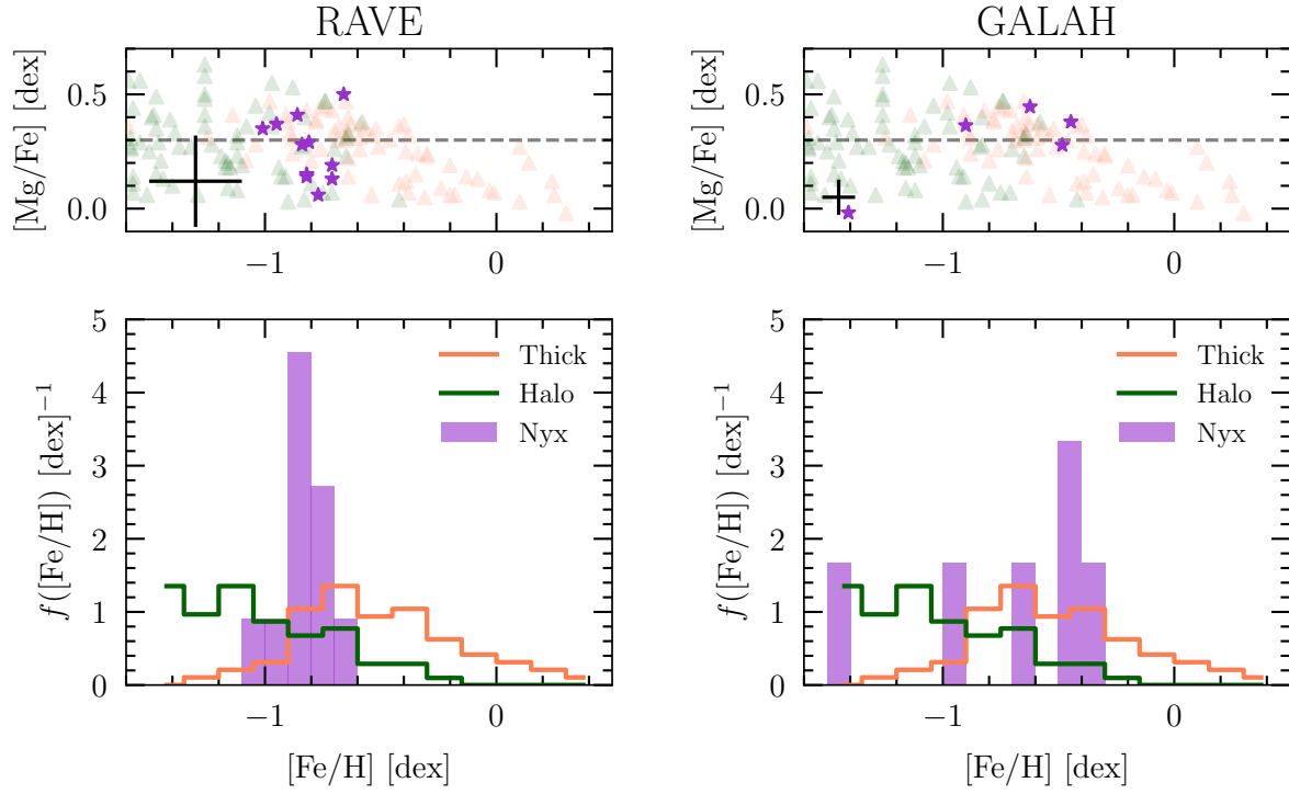
FIG. 5: Chemical abundance of the Nyx stars. This figure is similar to Fig. 2, but with abundances from RAVE [5] (left) and GALAH [6] (right), rather than RAVE-ON. The error bars are the 1-sigma uncertainties of the surveys.
