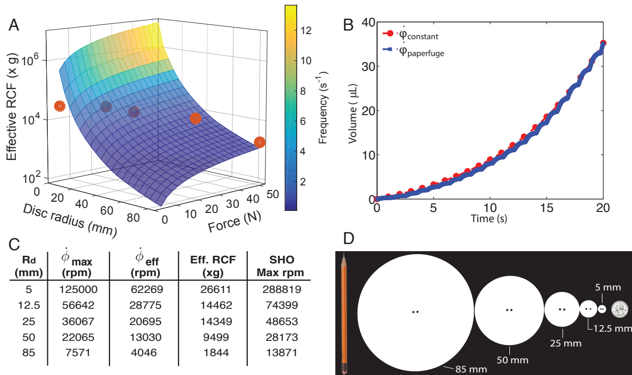
Figure 9: Scaling of RCF for paperfuge. A) Scaling curve of disc radius and input force for desirable effective RCF with experimental data in red. To generate this curve, the parameters used are: w_d = 0.3 mm, 4L = 0.661 m. The values for R_s were interpolated between 0.05 mm to 0.50 mm to correspond to experimental parameters (Table 3) B) Validation curve for effective RCF calculation. C) Maximum speed ( \dot{\phi}_{\text{max}} ), Effective speed ( \dot{\phi}_{\text{eff}} ), and Effective RCF attained experimentally from different paperfuges. \dot{\phi}_{\text{max}} attained from SHO approximation is also provided for comparison. D) Images of various sized paperfuges used in this study, with a pencil and a U.S. quarter shown for scale.
