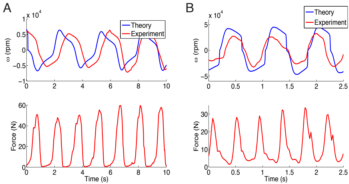
Figure 11: Validation data-sets for theory and experiment comparison Rotational speed from theoretical model and experimental data highlighting for A) R_d = 85 mm, and B) R_d = 25 mm. The experimental force profiles are shown below. The data-set is provided to highlight the ability of the theoretical model to match the measured dynamics of paperfuges of different disc sizes and parameters (see Table 3).
