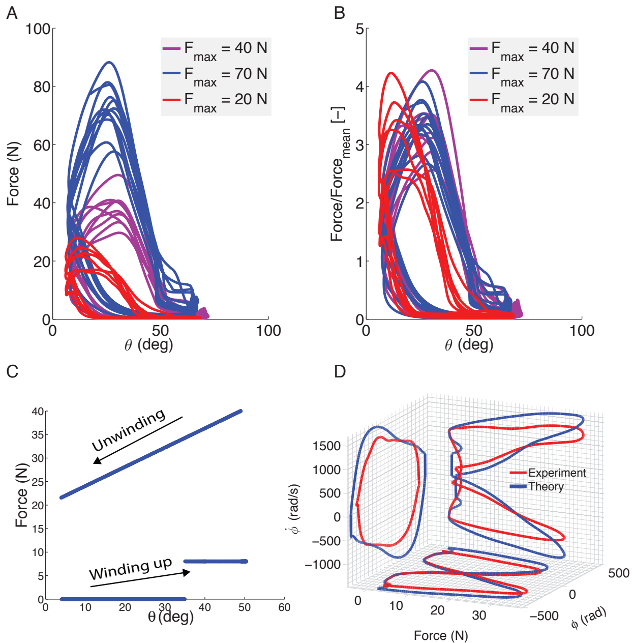
Figure 7: Theoretical Input Force. A) Experimental force vs. \theta at varying force-amplitudes ( F_{\max} = 20, 40 , and 70 N) for R_d = 50 mm. B) Normalized Experimental force vs. \theta space reveal that the force profiles collapse onto each other. C) Theoretical input force F_{th}(\theta) profile constructed from A and B. D) Phase space spanned by \dot{\phi} , F , and \phi , highlighting excellent agreement between theory and experiment.
