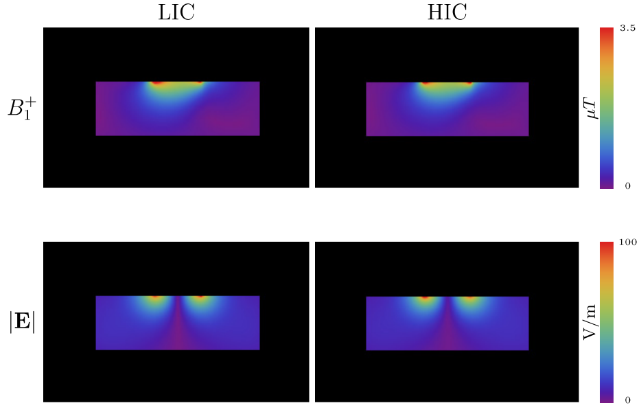
Supplemental Figure 13: Simulated \|E\| and B_1^+ fields in a large cuboid phantom (coronal slice through the center of the coil). The current distribution on the outside of the HIC (when the reversed pre-amplifier decoupling is deactivated) is almost identical to the traditional loop. Hence, both coils produce almost identical \mathbf{B} and \mathbf{E} fields. This observation is in agreement with the nearly identical single coil baseline SNR measured in our single LIC and HIC coil experiments (supplemental figure 15) and similar individual coil images in figure 2 of the main paper.
