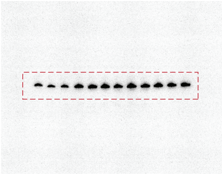
tRNA-Gly-CCC-2
