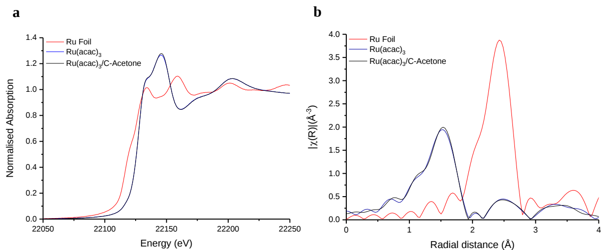
Supplementary Figure 6 – XAS characterisation of the freshly prepared 1wt.% Ru/C-Acetone catalyst. Ru K-edge a) XANES and b) FT-EXAFS of the freshly prepared 1wt.% Ru(acac) 3 /C-Acetone catalyst compared with the Ru foil and the Ru(acac) 3 standards.
