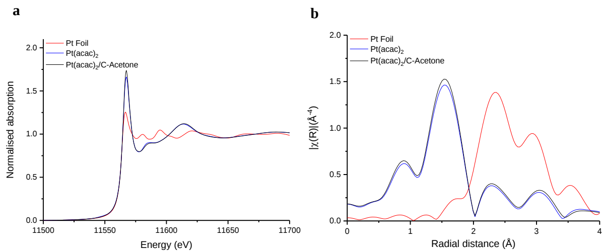
Supplementary Figure 5 – XAS characterisation of the freshly prepared 1wt.% Pt/C-Acetone catalyst. Pt L 3 -edge a) XANES and b) FT-EXAFS of the freshly prepared 1wt.% Pt(acac) 2 /C-Acetone catalyst compared with the Pt foil and the Pt(acac) 2 standards.
