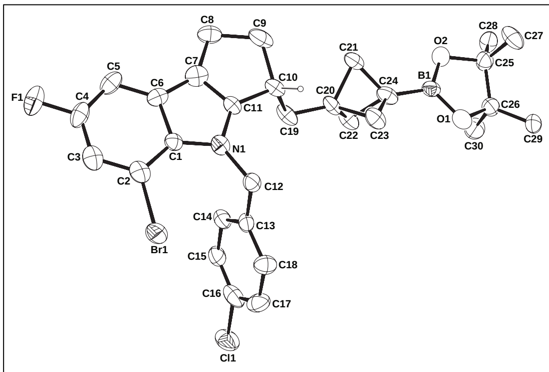
Figure S16. ORTEP drawing of molecule no. 1 with 50% thermal ellipsoids.
