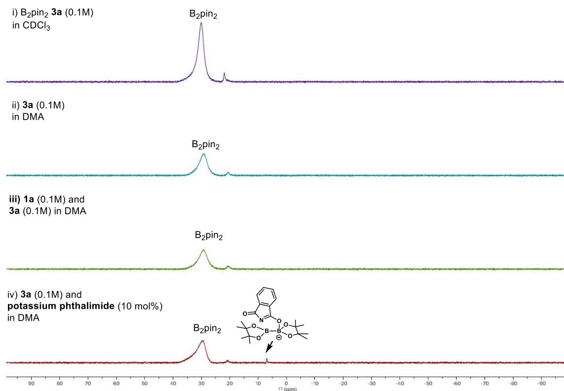
Figure S13. ^{11}\text{B} NMR data with RAE and \text{B}_2\text{pin}_2
