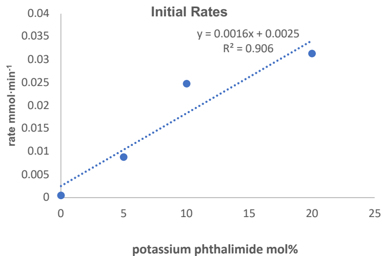
Figure S12. Plot of initial rates vs. the amount of potassium phthalimide indicates the participation of phthalimide in this multi-component borylation
