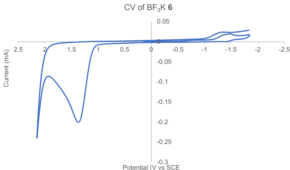
Figure S8. Cyclic voltammetry study on compound 6
