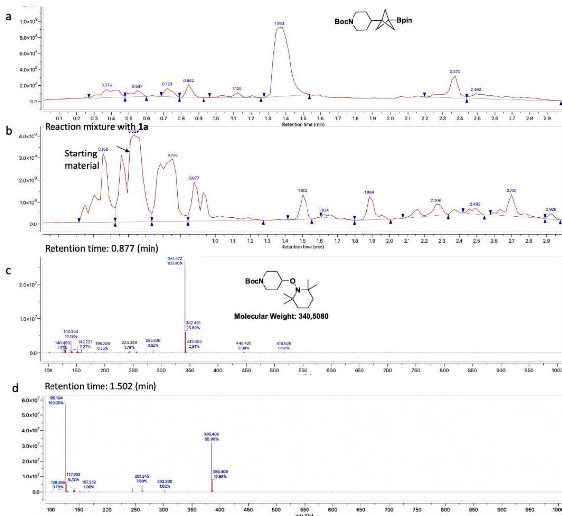
Figure S10. a) MS ES+ TIC spectra of 4k ; b) MS ES+ TIC spectra of the crude mixture with TEMPO showing no formation of product and remaining starting material; c) MS ES+ at 0.877 min, mass detected
