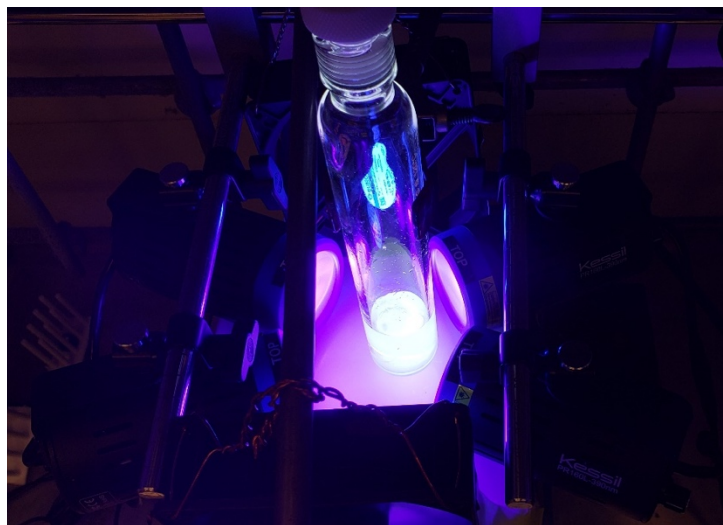
Figure S5. Gram-scale synthesis using 4 Kessil® LEDs at 50% power with 2 fans facing each other for cooling
