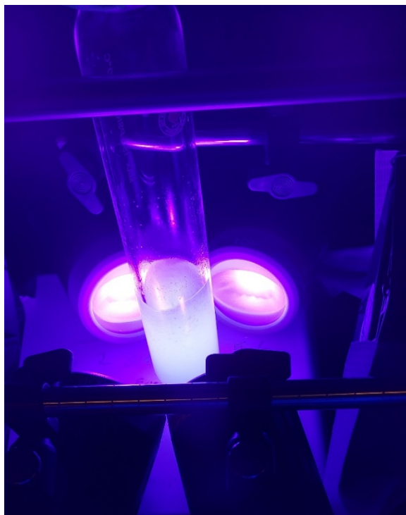
Figure S7. Gram-scale synthesis using 4 Kessil® LEDs at 100% power with 2 fans facing each other for cooling
