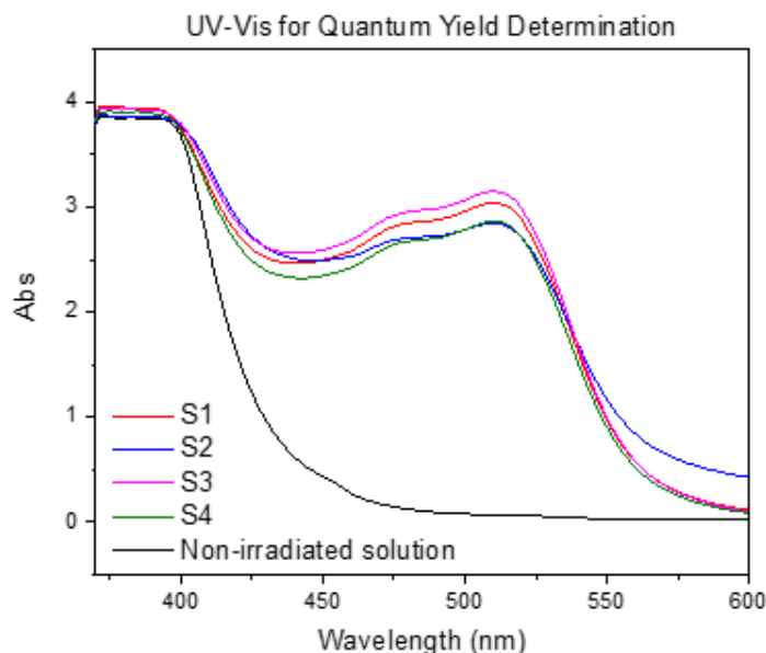
Figure S15. Absorbance curves of the 4 irradiated solution and of the non-irradiated solution
