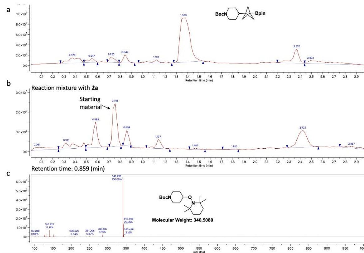
Figure S11. a) MS ES+ TIC spectra of 4j ; b) MS ES+ TIC spectra of the crude mixture with TEMPO showing no formation of product and remaining starting material; c) MS ES+ at 0.859 min, mass detected 341.496, [M+H]^+ calculated: 341.516
