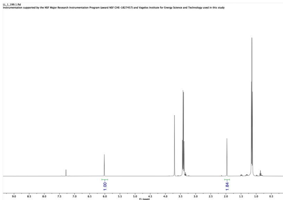
Figure S4. ^1\text{H} NMR spectrum for the propellane solution with 1,3,5-trimethoxybenzene in \text{CDCl}_3
