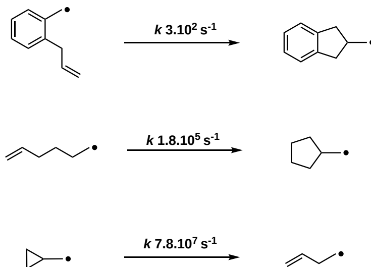
Scheme S1. Values for the radical clock used in our experiments 30
