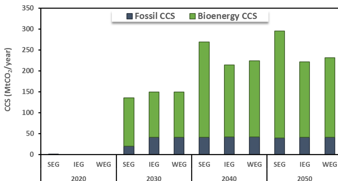
Figure S21 – CCS deployment across scenarios by type in Mt CO 2 /year
