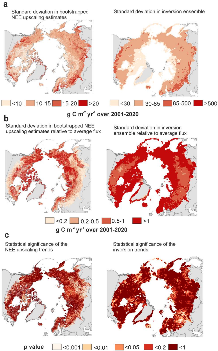
Supplementary Fig. 2. Uncertainties for the upscaled and inversion ensemble annual NEE. Standard deviations in upscaling were calculated from the outputs of 20 different bootstrapped models, and standard deviations in inversions were calculated across 5 inversion models; both thus represent the variability across different models (a) and the variability across the different models relative to the average flux (b). The p-values of the trends in c were determined using the Mann-Kendall test.
