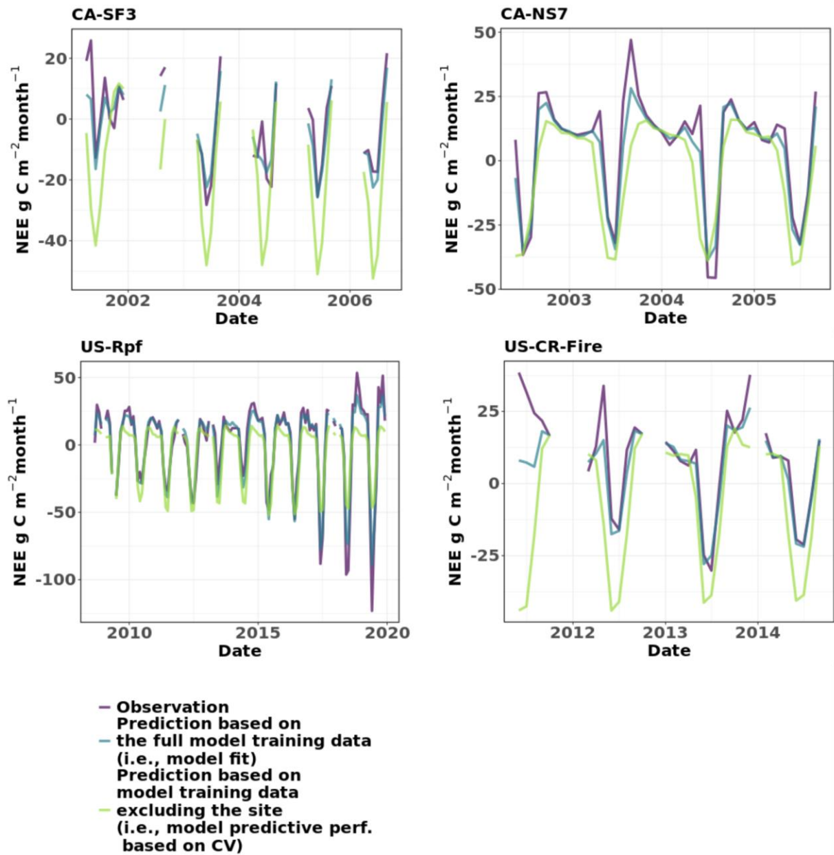
Supplementary Fig. 4. Time series of NEE from recently burned long-term (>3 years) sites and their agreement with model predictions. Model fit indicates how well the model trained with the entire model training data predicts to the same data, and model predictive performance shows how the models perform when a dataset excluding the specific site is used to train the model (i.e., leave-one-site-out cross validation).
