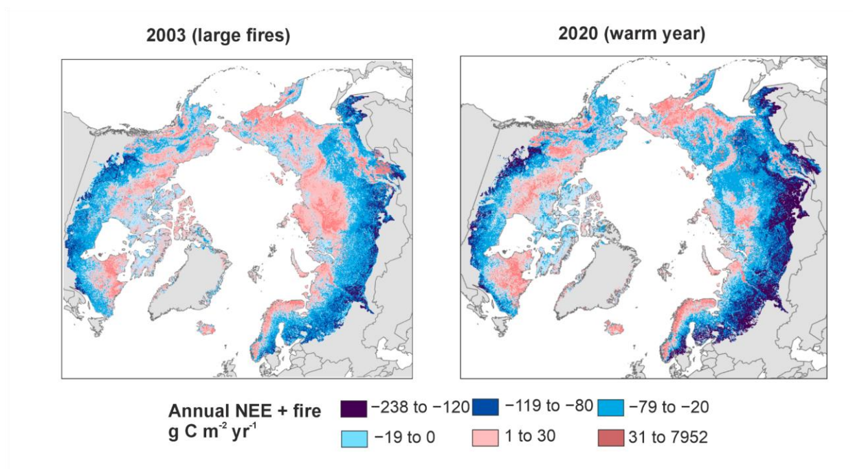
Supplementary Fig. 24. A visualization of how NEE + fire fluxes vary in 2003, when net CO 2 emission budget was the highest, and in 2020, when net CO 2 emission budget was the lowest.
