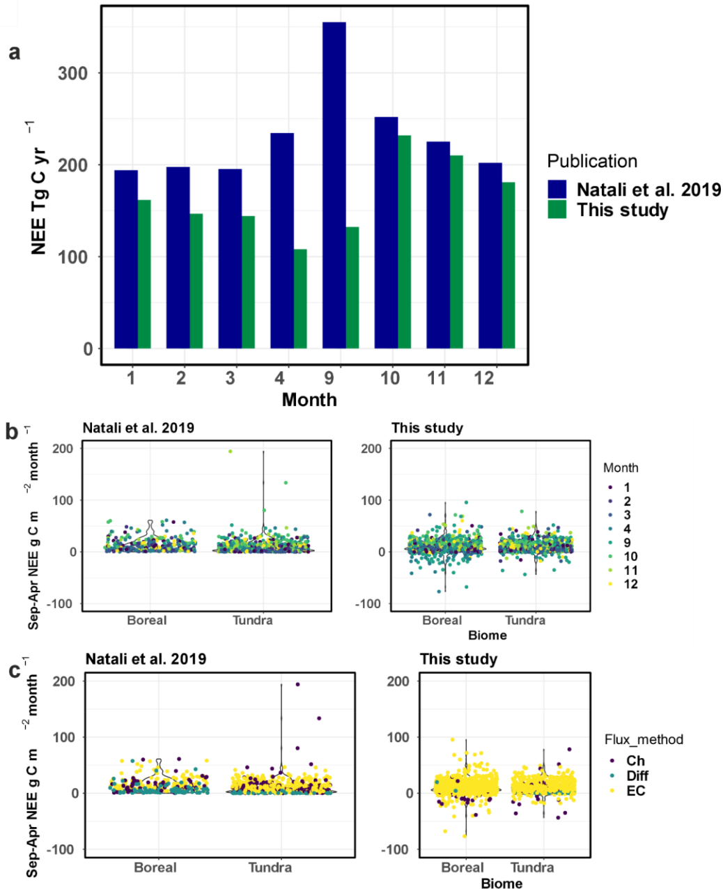
Supplementary Fig. 12. Comparison of the permafrost region non-growing season net ecosystem exchange (NEE) between Natali et al. (2019) and this study. The figure shows the comparison across monthly upscaled budgets (a), and in-situ monthly flux data visualized with months (b) and flux measurement methods (c). Natali et al. (2019) removed negative average monthly fluxes during the non-growing season to focus on net emissions, with a total number of site-months being 859 (in this study, site-months in the permafrost region totaled 1702). The October-April budget in this study was 1,181 Tg C yr -1 compared with 1,501 Tg C yr -1 in Natali et al. (2019) for the same period and domain; other studies have also shown that the non-growing season CO 2 budget in Natali et al. (2019) is higher compared to different data-driven bottom-up and top-down models 59–61 .
