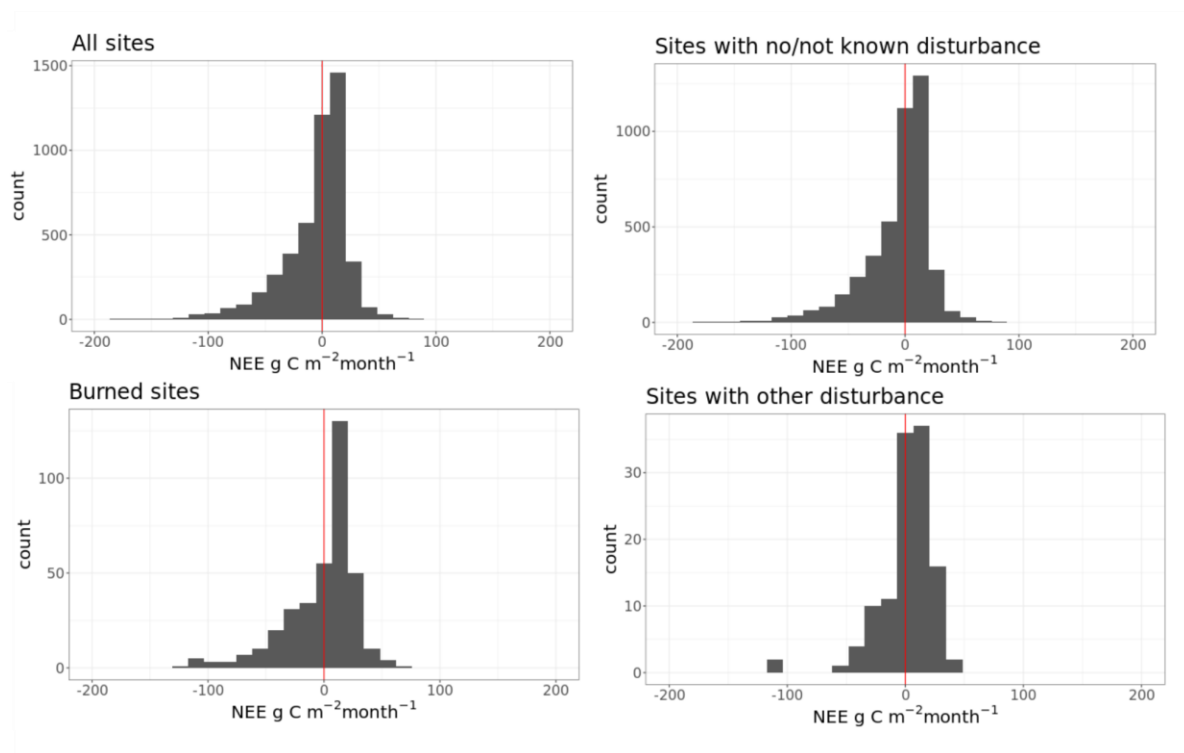
Supplementary Fig. 22. The distribution of monthly in-situ NEE data used to train the models. The red vertical line shows the zero flux.
