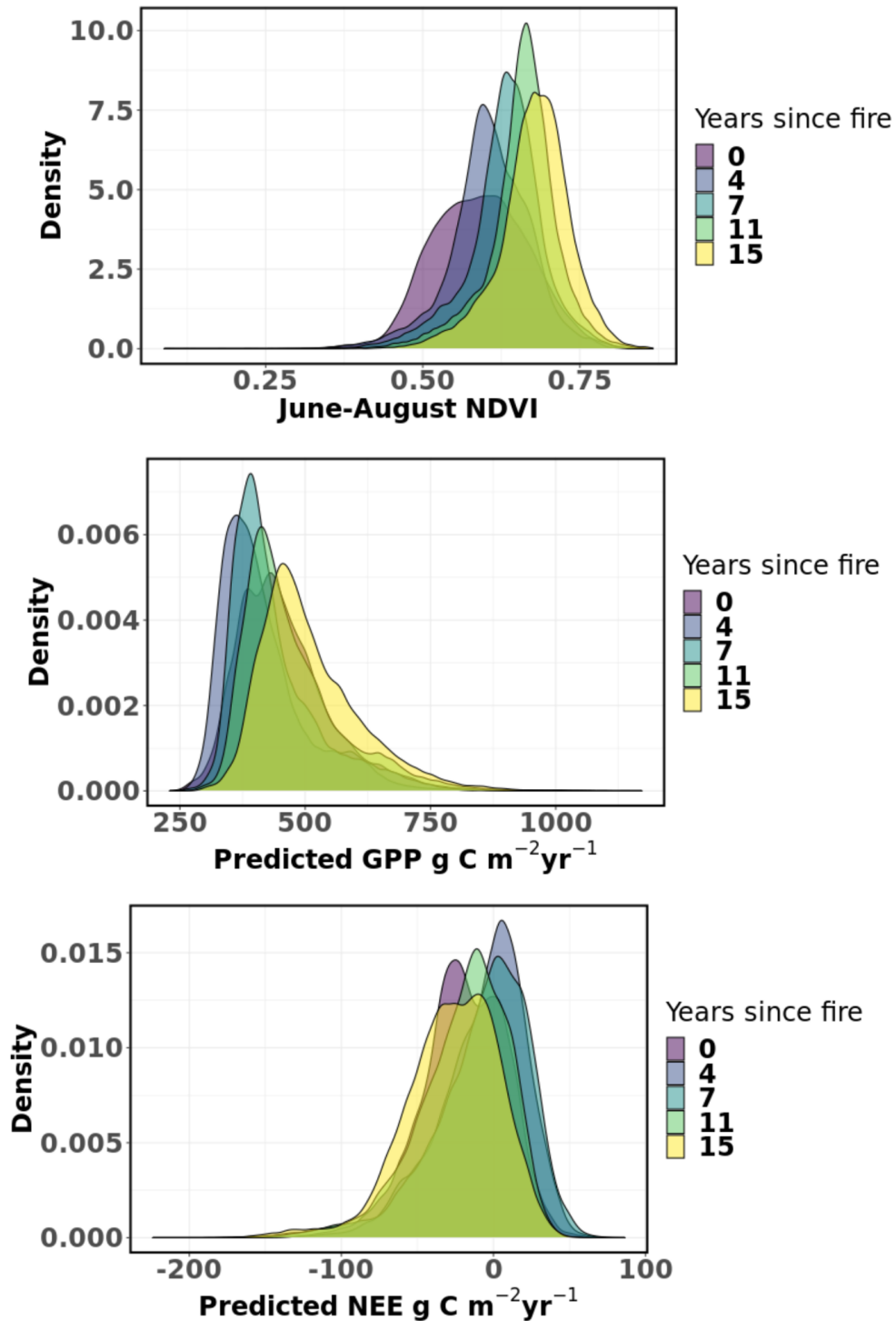
Supplementary Fig. 15. The Kernel density distribution of June-August NDVI, predicted annual GPP, and predicted annual NEE across pixels that were burned in 2004 from 0 to 15 years after the fire. Burned pixels were masked based on the pixels that had a direct fire emission of >200 \text{ g C m}^{-2} \text{ yr}^{-1} in the GFED-500m product and were located mainly in Alaska and northwestern Canada.
