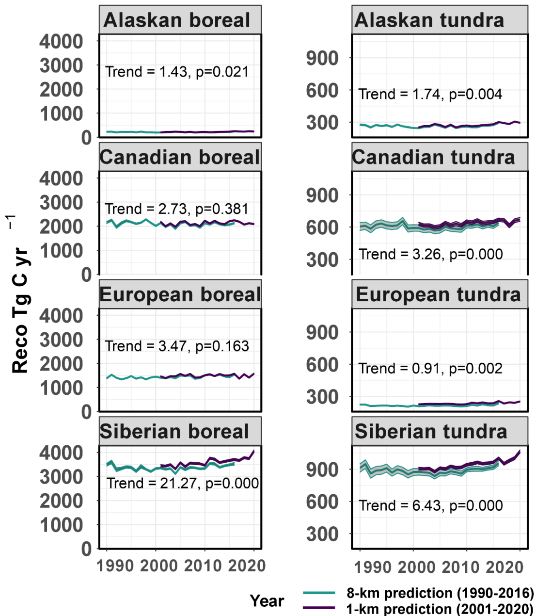
Supplementary Fig. 28. Time series of R_{eco} across the key regions. The central values (i.e., annual budgets) in figures a and b are derived from the outputs of the final model using the complete training dataset. The standard deviations (i.e., the error bars) are calculated from the outputs of 20 different models, each trained on a unique bootstrapped sample of the original training data. The magnitude of the trend was computed using the Theil-Sen approach, and the p-value determined using the Mann-Kendall test.
