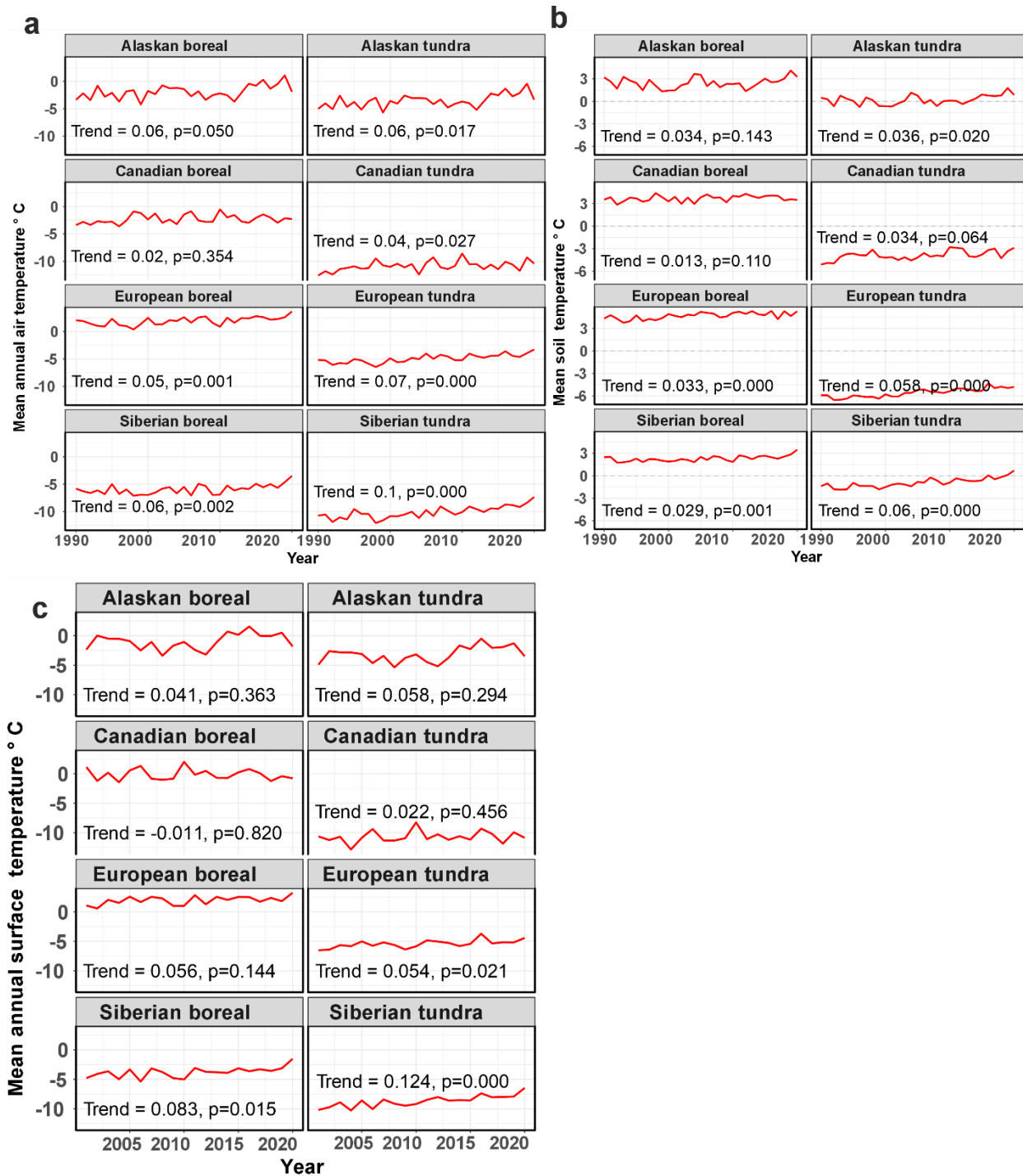
Supplementary Fig. 6. Trends (°C yr -1 ) for the air, land surface and soil temperature variables included in the models. Figures show that all regions are showing increases in air and soil temperatures. The Siberian tundra has the strongest air and soil temperature trends whereas the Canadian boreal has the weakest non-significant trends. The magnitude of the trend was computed using the Theil-Sen approach, and the p-value determined using the Mann-Kendall test.
