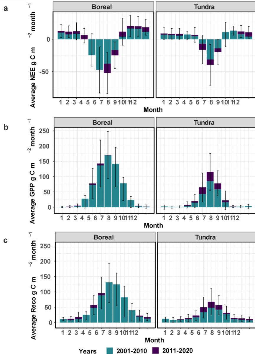
Supplementary Fig. 23. Average in-situ monthly NEE (n=4765), GPP (n=3869), and R_{eco} (n=3869) in boreal and tundra biomes during the past two decades. Error bars represent the standard deviation across averaged site-level months (i.e., they characterize spatial variability). Sample size for individual months were 288 (NEE) and 230 (GPP, R_{eco} ) for January, 289 (NEE) and 237 (GPP, R_{eco} ) for February, 329 (NEE) and 253 (GPP, R_{eco} ) for March, 377 (NEE), 275 (GPP) and 274 ( R_{eco} ) for April, 449 (NEE) and 363 (GPP, R_{eco} ) for May, 497 (NEE), 421 (GPP, R_{eco} ) for June, 527 (NEE) and 445 (GPP, R_{eco} ) for July, 522 (NEE) and 444 (GPP, R_{eco} ) for August, 475 (NEE) and 390 (GPP, R_{eco} ) for September, 386 (NEE), 314 (GPP) and 315 ( R_{eco} ) for October, 320 (NEE) and 257 (GPP, R_{eco} ) for November, and 306 (NEE) and 240 (GPP, R_{eco} ) for December. Note that this figure is highly uncertain as it does not account for the differences in the site distribution across the two decades. Fig. 3 in the main text shows the upscaled monthly fluxes that should better represent the average fluxes across the entire ABZ.
