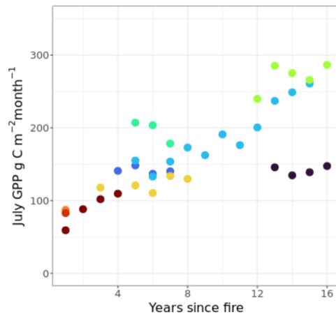
Supplementary Fig 13. Site-level remote sensing-based NDVI, and in-situ and upscaled flux data in recently burned sites. The figures show a clear increasing NDVI, GPP and net uptake signal after the fire. The upscaled fluxes show the actual predictions and not those based on cross validation.
