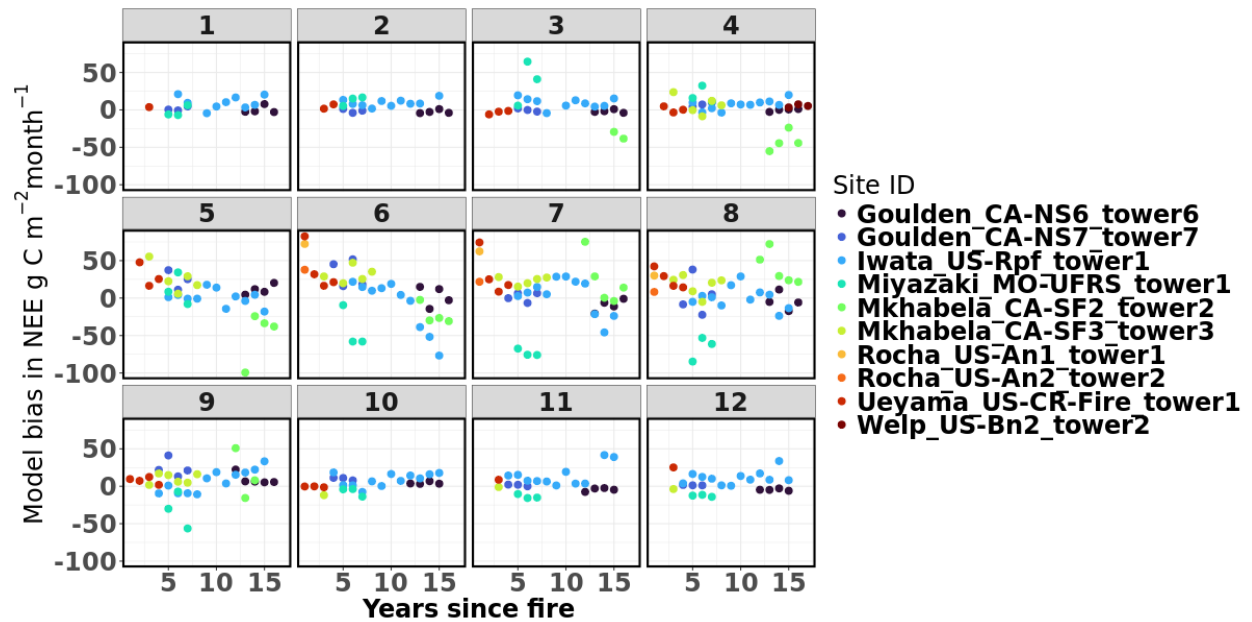
Supplementary Fig. 16. Bias in monthly NEE based on cross validation as a function of years since fire and separated by months. The only months with a statistically significant effect of years since fire were May (intercept: 39.0, p=0.001 ; slope: -3.8, p=0.02 ), June (intercept: 65.2, p=0.00 , slope: -8.5, p=0.006 ), and July (intercept: 34.1, p=0.03 ; slope: -3.7, p=0.008 ), based on linear mixed-effects model with the bias as a response and years since fire as a predictor.
