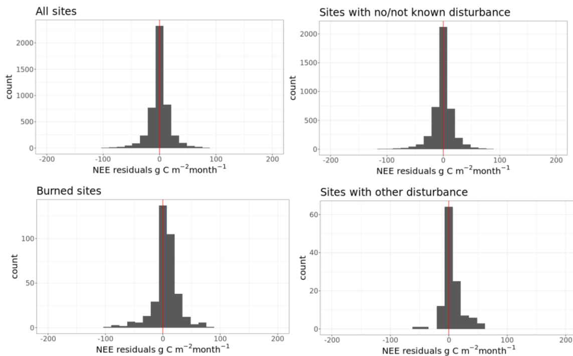
Supplementary Fig. 14. The distribution of monthly residuals of NEE. The red vertical line differentiates positive and negative residuals. A negative residual value represents the model overestimating NEE, i.e., underestimating net CO 2 sinks or overestimating net CO 2 sources.
