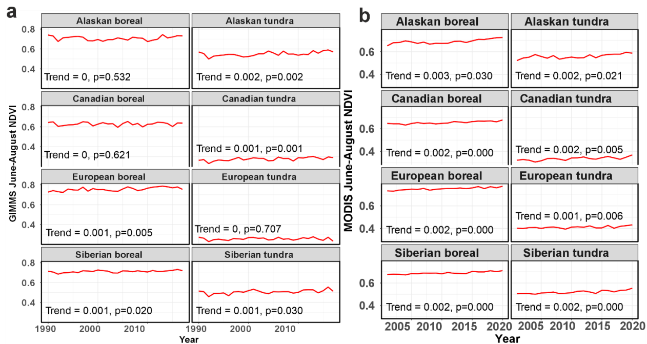
Supplementary Fig. 7. Trends for the NDVI variables for the June-August period. The GIMMS dataset used here covers a longer time period (1990-2016) but is limited to 8-km pixel resolution, whereas the MODIS NDVI time series goes from 2001 to 2020 and is at 1-km pixel resolution. Average greening trends are almost equally strong across the regions in the MODIS era but there is more variability in the GIMMS era. Weakest trends are found in European tundra across both the datasets; GIMMS shows strong trends particularly in Alaskan tundra. The magnitude of the trend was computed using the Theil-Sen approach, and the p-value determined using the Mann-Kendall test.
