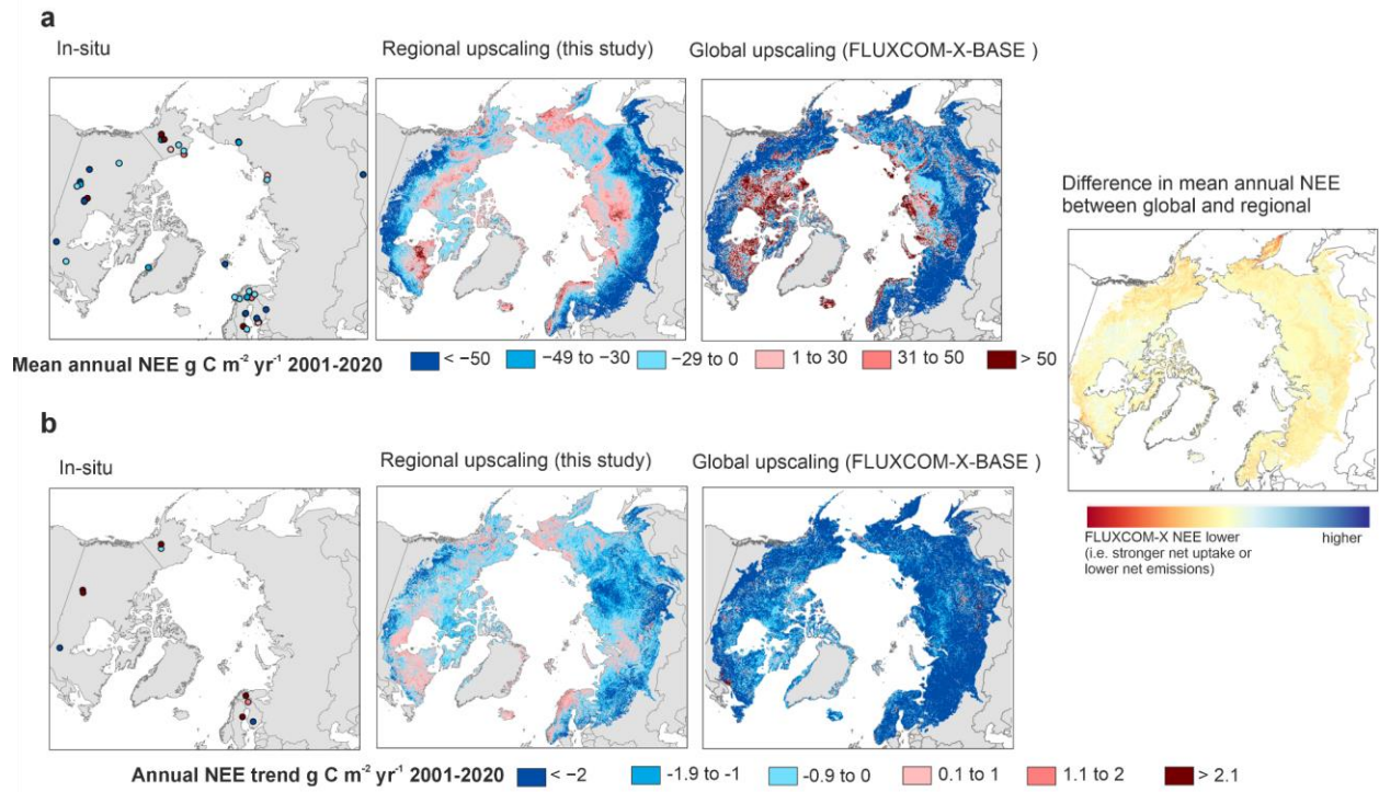
Supplementary Fig. 25. Maps showing the averages and trends in annual NEE in our upscaling and FLUXCOM-X-BASE, and the differences between those.
