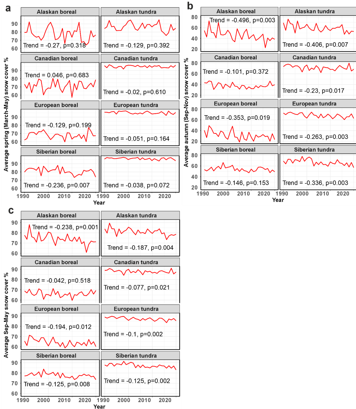
Supplementary Fig. 8. Trends (% yr -1 ) for the snow cover variable included in the models. The figures show that all regions experience declining snow cover in spring, autumn, and the entire non-summer (September-May) season. However, snow cover trends are stronger and statistically significant primarily in the autumn season, except for the Siberian boreal region that experiences a strong statistically significant declining trend in the spring. Declines in snow cover are the steepest in Alaskan boreal and tundra regions. The magnitude of the trend was
