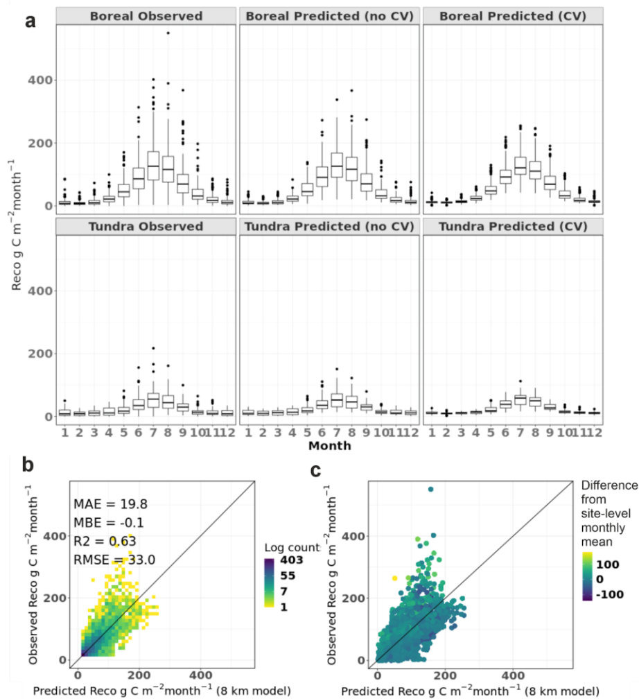
Supplementary Fig. 19. Predictive performance of the Reco model. The monthly Reco variability of observed fluxes, and predicted fluxes based on the same train and test dataset (no cross validation; no CV) and a leave-one-site-out CV (CV) approach (a). The model training dataset comprised a total of 3869 samples. Monthly sample sizes were distributed as follows: 230 in January; 237 in February; 253 in March; 274 in April; 363 in May; 421 in June; 445 in July; 444 in August; 390 in September; 315 in October; 257 in November; and 240 in December. The lower and upper hinges in the boxes correspond to the first and third quartiles (the 25th and 75th percentiles) and the line between the median. The whiskers extend from the quartiles to the furthest data points within 1.5 \times \text{IQR} , where IQR is the interquartile range; data beyond the end of the whisker are visualized with dots. Subplots b and c show the correlation between observed and predicted fluxes, colored by the density of observations (b) or the deviance from average site-level monthly flux (c). Subfigure c indicates that the model struggles the most when observations from individual sites have a large deviance from the mean. Coefficient of determination ( R^2 ) describes the strength of the linear relationship between the observed and predicted fluxes. Mean bias error (MBE) characterizes the average bias between prediction and observation, with negative values indicating the model to underestimate NEE (i.e., overestimate net \text{CO}_2 sinks or underestimate net \text{CO}_2 sources). Mean absolute error
