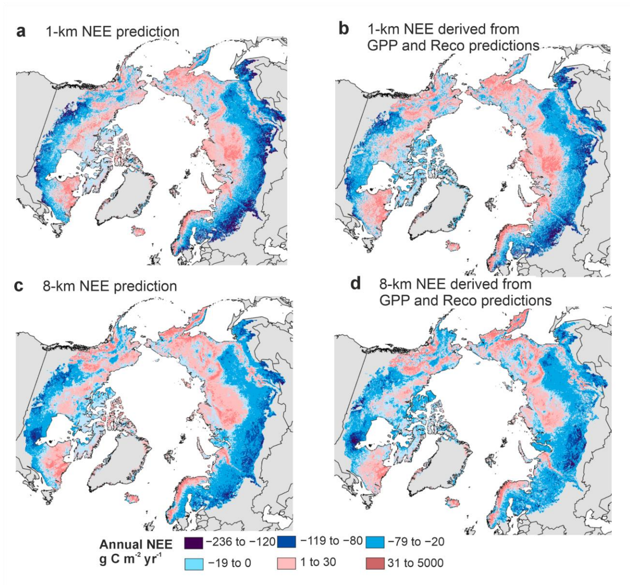
Supplementary Fig. 17. A comparison of upscaled NEE at 1 and 8-km predictions and from directly derived NEE or GPP- R_{\text{eco}} -derived NEE. In some areas, our upscaling showed higher than expected NEE values. For example, some sparsely vegetated or barren mountainous regions in northern Siberia (Kolyma mountains) or northern Europe (Scandes mountains) showed net emissions of 30-50 g C m -2 yr -1 , which appears elevated compared to the low vegetation carbon inputs and overall soil carbon pools.
