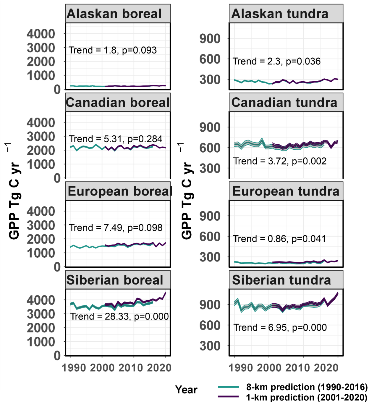
Supplementary Fig. 27. Time series of GPP across the key regions. The central values (i.e., annual budgets) in figures a and b are derived from the outputs of the final model using the complete training dataset. The standard deviations (i.e., the error bars) are calculated from the outputs of 20 different models, each trained on a unique bootstrapped sample of the original training data. The magnitude of the trend was computed using the Theil-Sen approach, and the p-value determined using the Mann-Kendall test.
