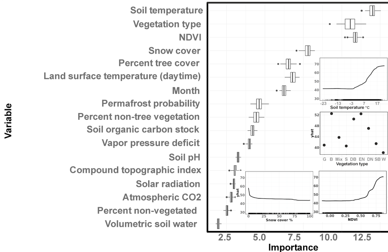
Supplementary Fig. 21. Variable importance plots and the partial dependence plots for the most important predictors of the R_{eco} model. The variable importance boxes show the scores from 100 simulations, with the lower and upper hinges corresponding to the first and third quartiles (the 25th and 75th percentiles) and the line between the median. The whiskers extend from the quartiles to the furthest data points within 1.5 \times IQR , where IQR is the interquartile range; data beyond the end of the whisker are visualized with dots. Vegetation types include G=graminoid, B=barren, Mix=mixed forest and mosaic vegetation type, S=shrub, DB=deciduous broadleaf forest, EN=evergreen needleleaf forest, DN=deciduous needleleaf forest, SB=sparse boreal vegetation, W=wetland. The values on the y axis of each partial dependence plot can be interpreted as followed: \hat{y} is conditional on other predictors in the model and their relationships with the predictor in the plot in question. Therefore, \hat{y} values should not be directly compared with observed or predicted values, rather the patterns in \hat{y} should be explored more generally. The x-axis represents the actual predictor values and can be used to infer, for example, conditions that lead to changes in \hat{y} (tipping points), and the strength and direction of the relationship.
