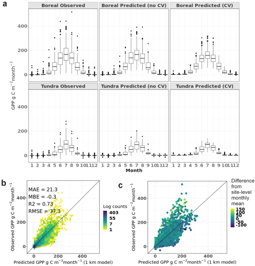
Supplementary Fig. 18. Predictive performance of the GPP model. The monthly GPP variability of observed fluxes, and predicted fluxes based on the same train and test dataset (no cross validation; no CV) and a leave-one-site-out CV (CV) approach (a). The model training dataset comprised a total of 3869 samples. Monthly sample sizes were distributed as follows: 230 in January; 237 in February; 253 in March; 275 in April; 363 in May; 421 in June; 445 in July; 444 in August; 390 in September; 314 in October; 257 in November; and 240 in December. The lower and upper hinges in the boxes correspond to the first and third quartiles (the 25th and 75th percentiles) and the line between the median. The whiskers extend from the quartiles to the furthest data points within 1.5 * IQR, where IQR is the interquartile range; data beyond the end of the whisker are visualized with dots. Subplots b and c show the correlation between observed and predicted fluxes, colored by the density of observations (b) or the deviance from average site-level monthly flux (c). Subfigure c indicates that the model struggles the most when observations from individual sites have a large deviance from the mean. Coefficient of determination ( R^2 ) describes the strength of the linear relationship between the observed and predicted fluxes. Mean bias error (MBE) characterizes the average bias between prediction and observation, with negative values indicating the model to underestimate NEE (i.e., overestimate net CO 2 sinks or underestimate net CO 2 sources). Mean absolute error (MAE) describes the absolute bias between prediction and observation, with larger values describing larger errors.
