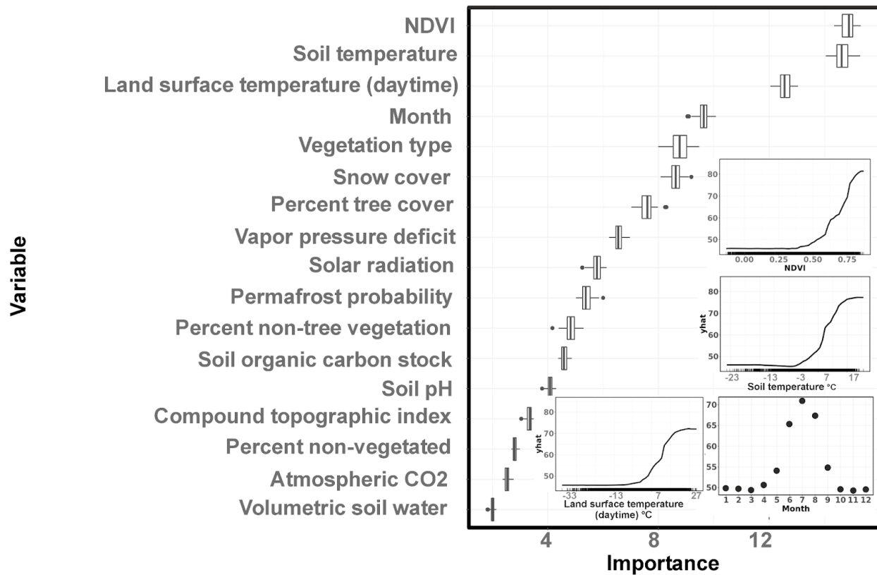
Supplementary Fig. 20. Variable importance plots and the partial dependence plots for the most important predictors of the GPP model. The variable importance boxes show the scores from 100 simulations, with the lower and upper hinges corresponding to the first and third quartiles (the 25th and 75th percentiles) and the line between the median. The whiskers extend from the quartiles to the furthest data points within 1.5 \times \text{IQR} , where IQR is the interquartile range; data beyond the end of the whisker are visualized with dots. The values on the y axis of each partial dependence plot can be interpreted as followed: yhat is conditional on other predictors in the model and their relationships with the predictor in the plot in question. Therefore, yhat values should not be directly compared with observed or predicted values, rather the patterns in yhat should be explored more generally. The x-axis represents the actual predictor values and can be used to infer, for example, conditions that lead to changes in yhat (tipping points), and the strength and direction of the relationship.
