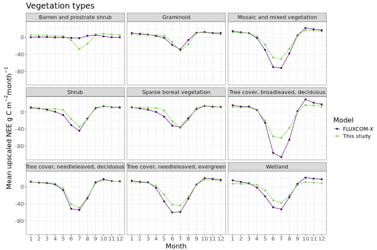
Supplementary Fig. 26. Mean upscaled monthly NEE fluxes in this study and FLUXCOM-X-BASE across key vegetation types.
