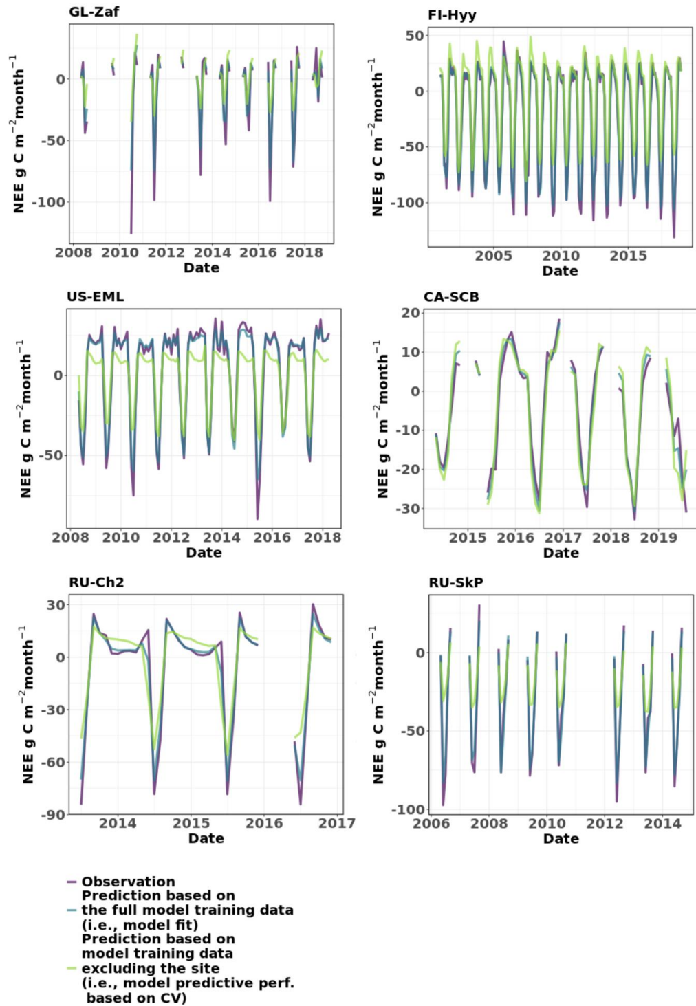
Supplementary Fig. 3. Time series of NEE from a subset of sites and their agreement with model predictions. Model fit indicates how well the model trained with the entire model training data predicts to the same data, and model predictive performance shows how the models perform when a dataset excluding the specific site is used to train the model (i.e., leave-one-site-out cross validation).
