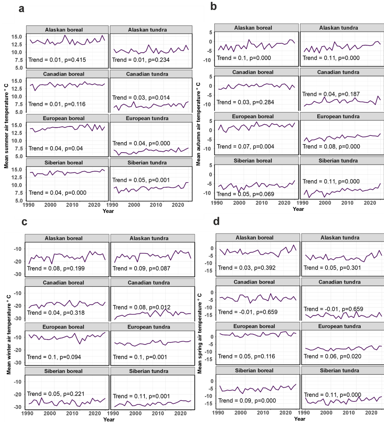
Supplementary Fig. 10. Trends (°C yr -1 ) for the air temperature variables in different climatological seasons. The magnitude of the trend was computed using the Theil-Sen approach, and the p-value determined using the Mann-Kendall test.
