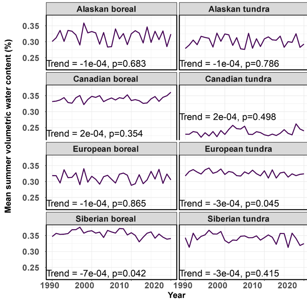
Supplementary Fig. 9. Trends (% yr -1 ) for June-August soil moisture. The magnitude of the trend was computed using the Theil-Sen approach, and the p-value determined using the Mann-Kendall test.
