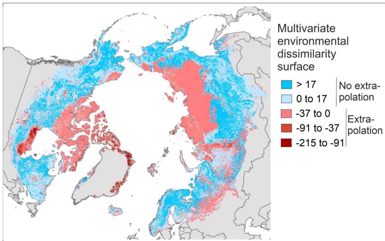
Supplementary Fig. 1. The area of extrapolation for NEE models based on sites that have data at least from one January (i.e., year-round sites).
