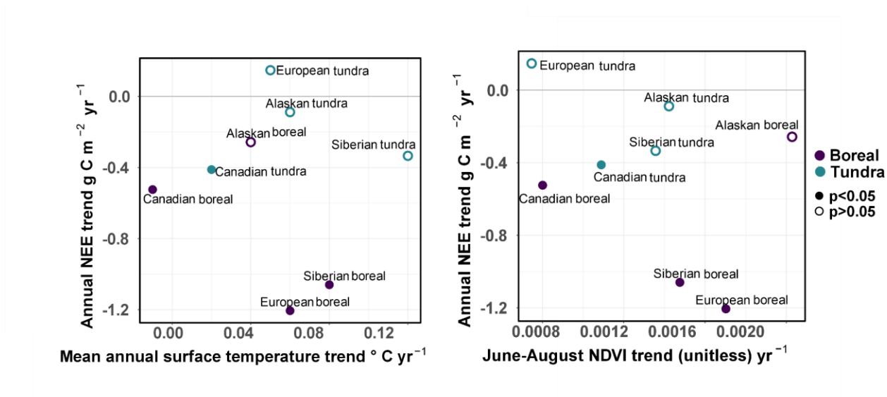
Supplementary Fig. 5. Correlation between average temperature and NDVI trends with upscaled average annual NEE trends over 2001-2020. The magnitude of the trend was computed using the Theil-Sen approach, and the p-value determined using the Mann-Kendall test. The statistical significance of the NEE trend is shown with full and empty circles.
