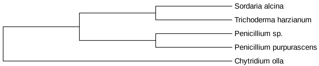
Maximum likelihood tree for study 120
