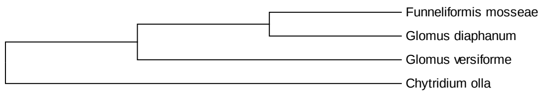
Maximum likelihood tree for study 533
