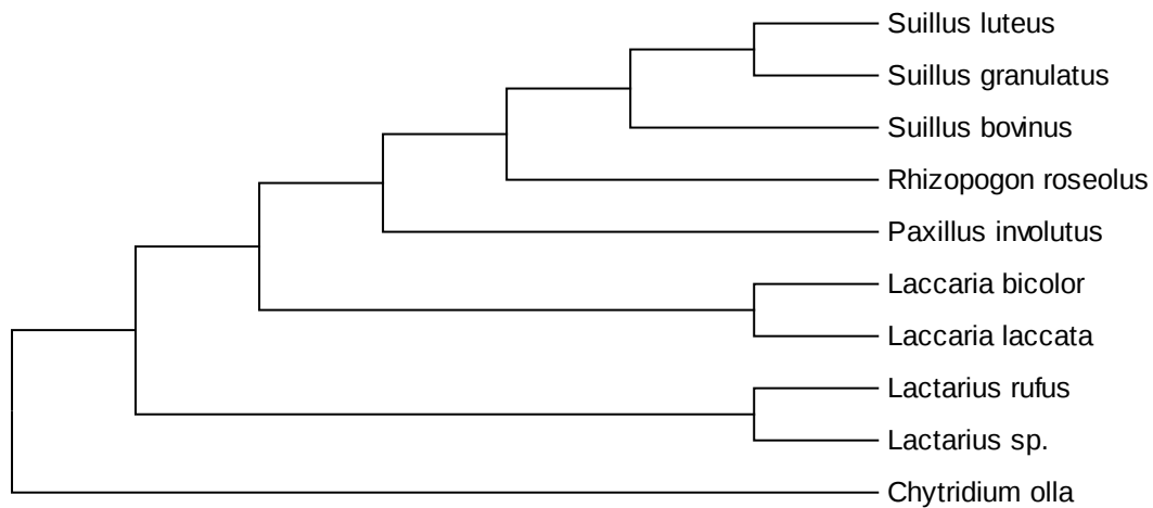
Maximum likelihood tree for study 680
