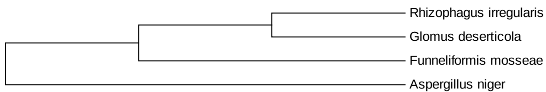
Maximum likelihood tree for study 98
