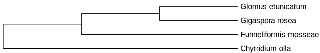
Maximum likelihood tree for study 689
