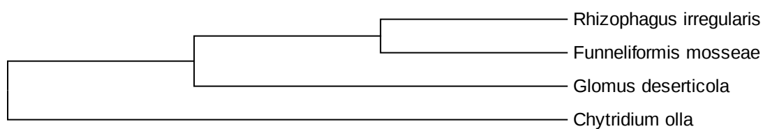
Maximum likelihood tree for study 107
