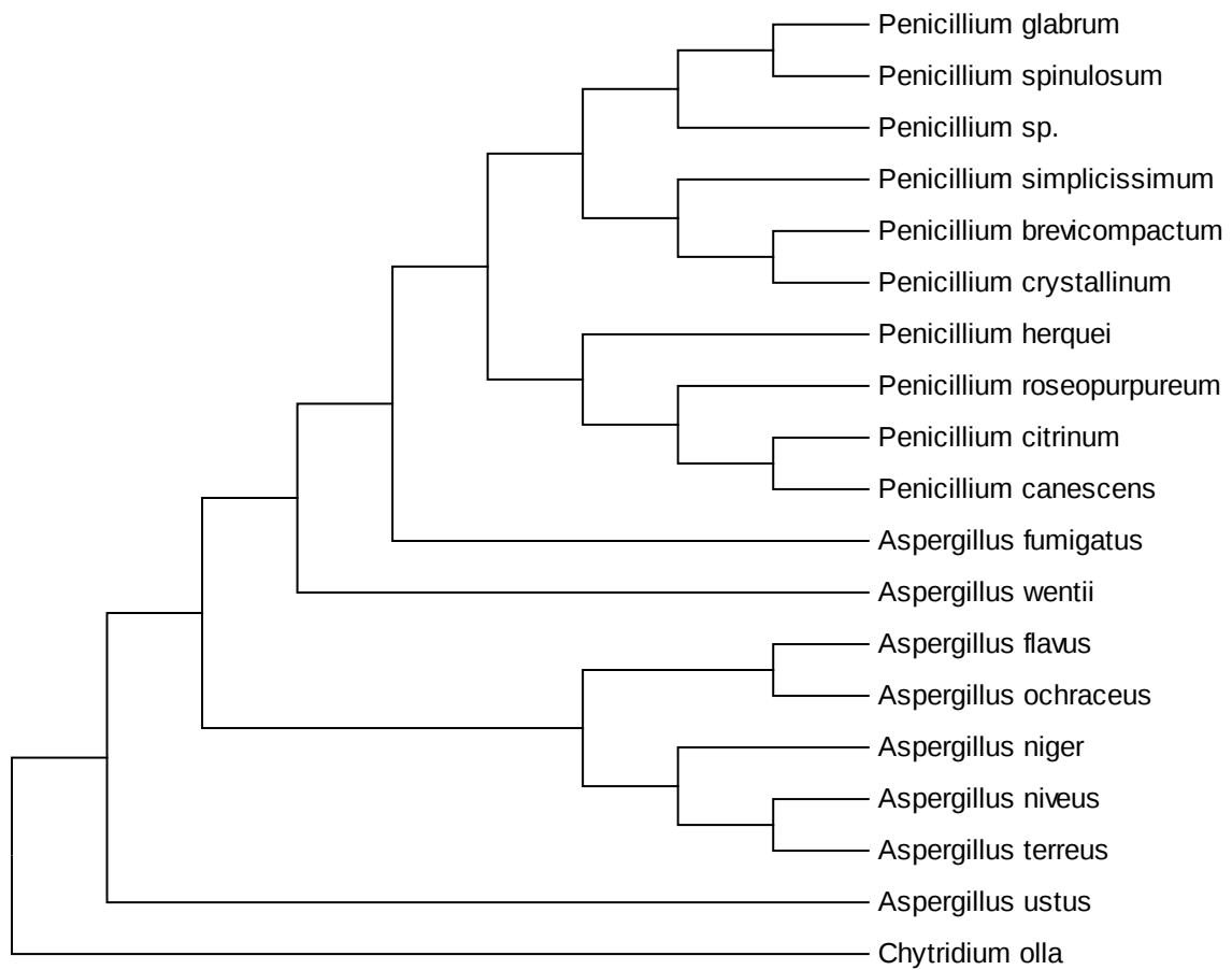
Maximum likelihood tree for study 154
