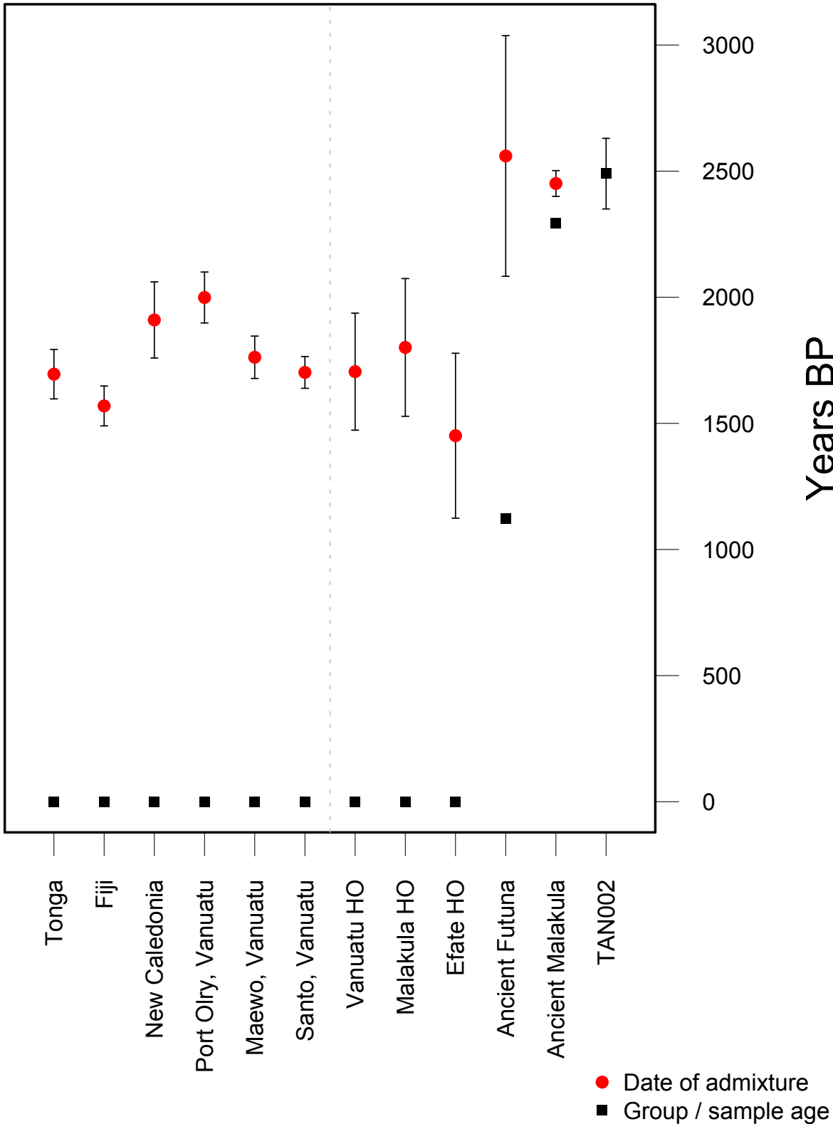
Supplementary figure 9. ALDER analyses estimating the date of Papuan and East Asian admixture, converted into years with a generation time of 28.1 years. Populations investigated derive from Parks et al. 32 (left of the dashed gray line), the newly HO genotyped Vanuatu individuals, either grouped together Vanuatu HO ( n=27 ) or divided as Malakula HO ( n=21 ) and Efate HO ( n=6 ), and ancient Futuna ( n=3 ) and Malakula ( n=3 ). Standard error bars are shown for date estimates, while sample ages for the two ancient groups (Futuna and Malakula) are averaged radiocarbon dating confidence interval (CI) midpoints. As the earliest ancient Vanuatu individual with unadmixed Near Oceanian ancestry, TAN002 is included for age comparison, with error bar indicating the 95.4% radiocarbon dating CI.
