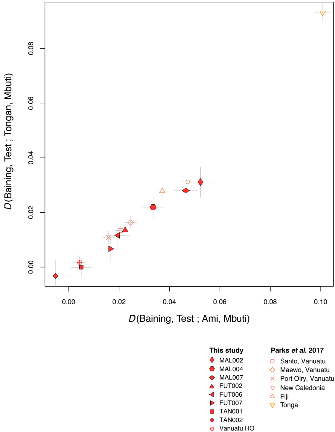
Supplementary figure 8. D -statistics in the form D(\text{Baining, Test} ; \text{Ami, Mbuti}) and D(\text{Baining, Test} ; \text{modern Tongan, Mbuti}) plotted against each other, where Test is Fiji, Tonga, Maewo (Vanuatu), Port Olry (Vanuatu), Santo (Vanuatu) and New Caledonia populations from Parks et al. 32 , modern-day Vanuatu HO individuals and ancient Malakula, Futuna and Tanna individuals from this study. Standard errors for each point are shown in both dimensions as gray lines.
