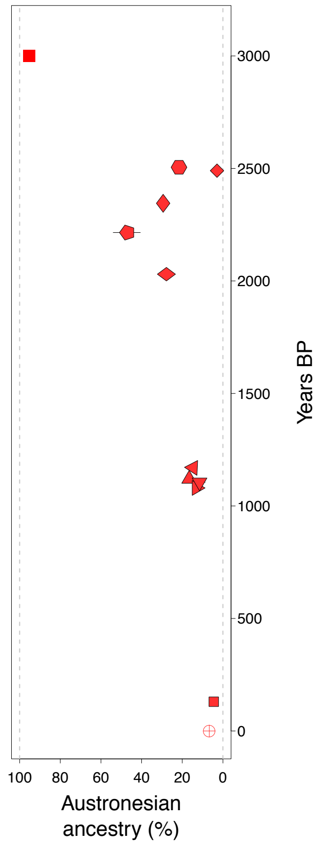
Supplementary figure 3. qpAdm analyses on the down-sampled SNPs of the HO dataset modeling the Austronesian ancestry proportion (represented by Ami population) in ancient individuals (filled symbols) and 27 present-day individuals grouped together (unfilled symbol) from Vanuatu. Standard errors are shown as black lines if larger than the sample symbol (legend in Fig. 1).
