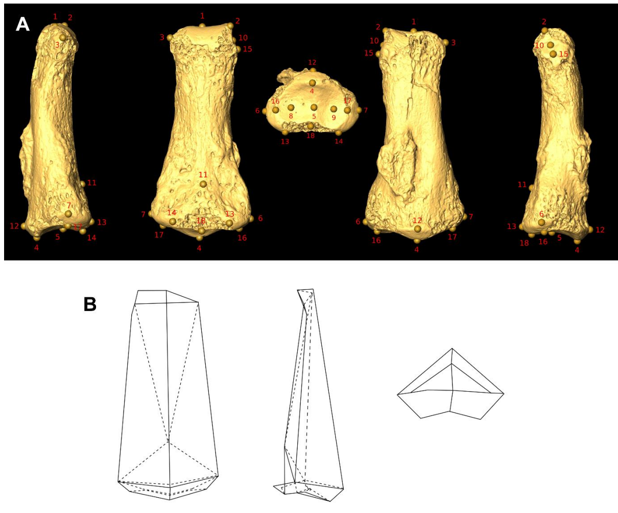
Supplementary Figure 2. Landmarks and wireframes used in geomorphometric analyses. A: Landmarks used to analyse phalanx shape using GMM. Landmarks numbered as in Supplementary Table 4 (AW-1 shown); B: Wireframes composed of straight lines connecting landmarks shown in A. Dorsal (left), lateral (middle) and proximal (right) views. Dotted lines connect landmarks not visible when bone is present, some lines omitted in proximal view for ease of visualisation.
