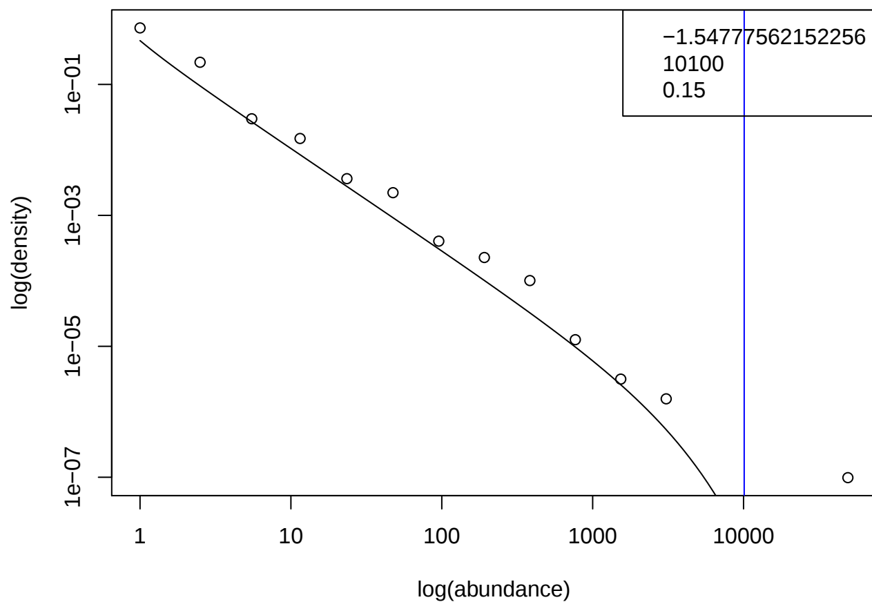
TARA_089.SUR.20.180.DNA
