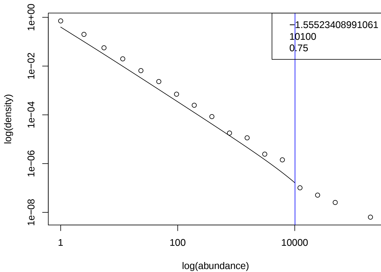
TARA_149.SUR.5.20.DNA
