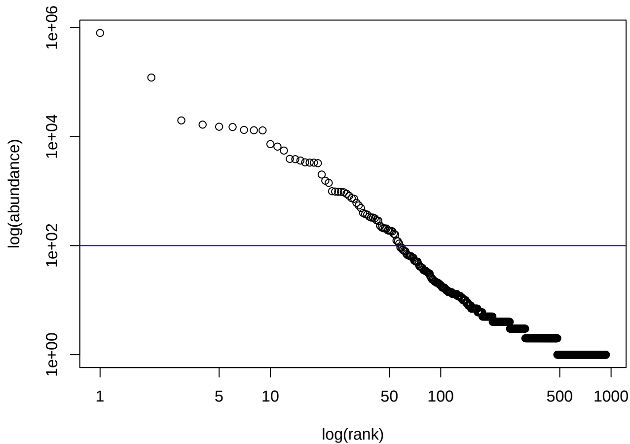
TARA_146.SUR.180.2000.DNA
