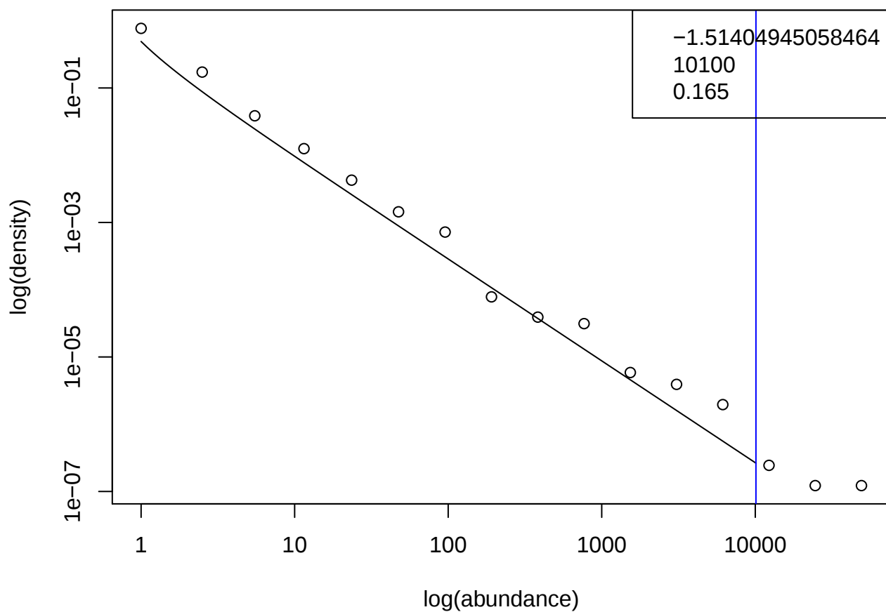
TARA_080.SUR.180.2000.DNA
