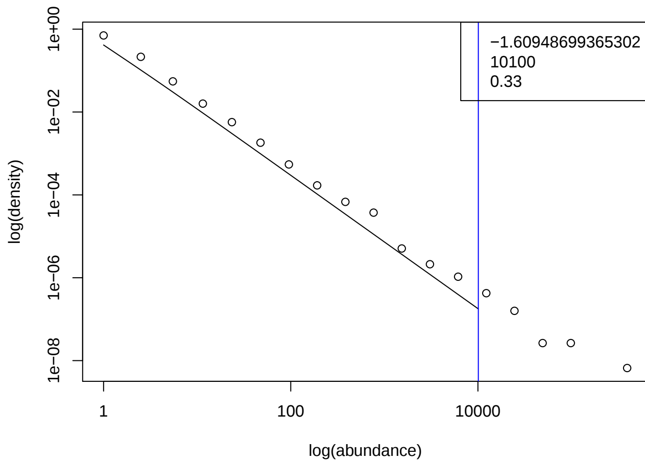
TARA_046.SUR.180.2000.DNA
