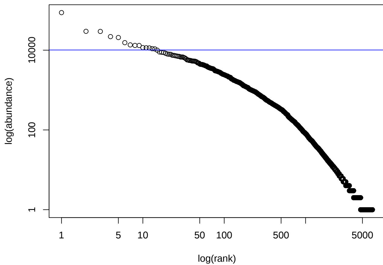
TARA_009.SUR.0.8.5.DNA
