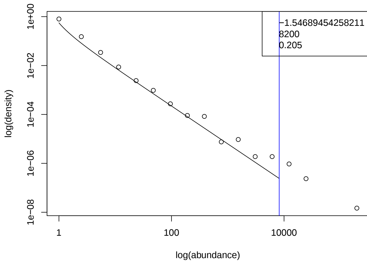
TARA_050.SUR.180.2000.DNA
