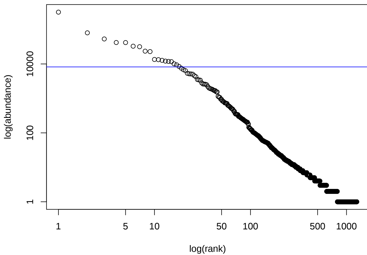
TARA_084.SUR.20.180.DNA
