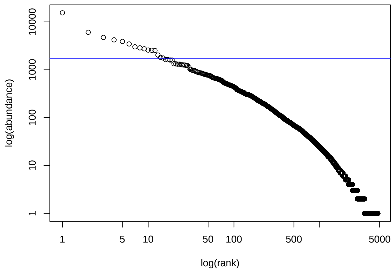
TARA_058.SUR.0.8.5.DNA
