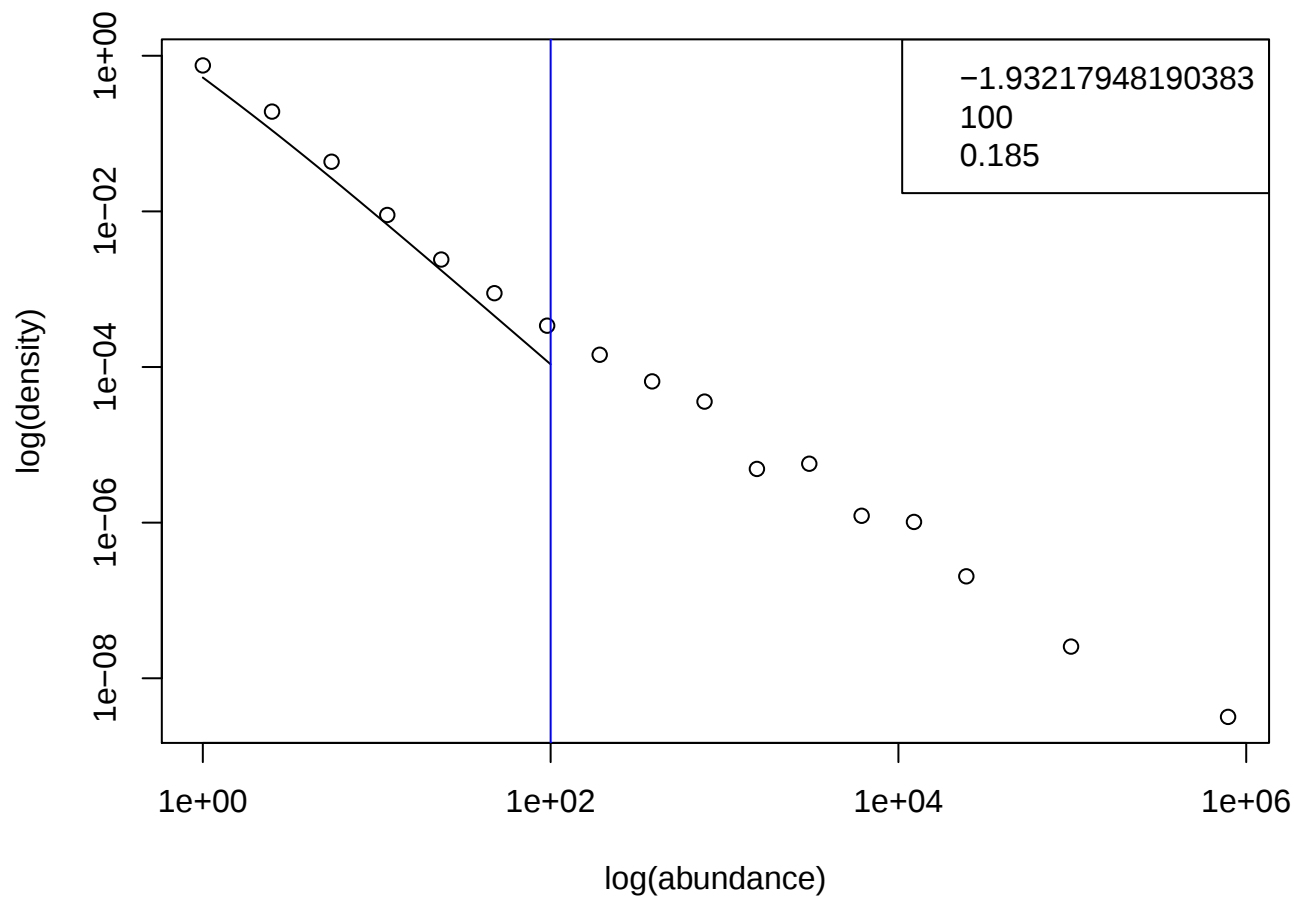
TARA_146.SUR.180.2000.DNA
