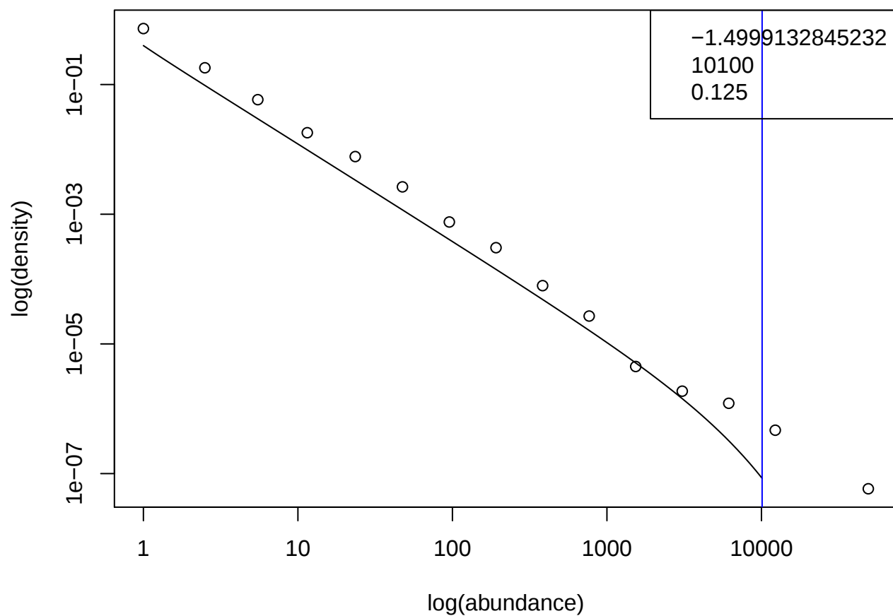
TARA_023.SUR.20.180.DNA
