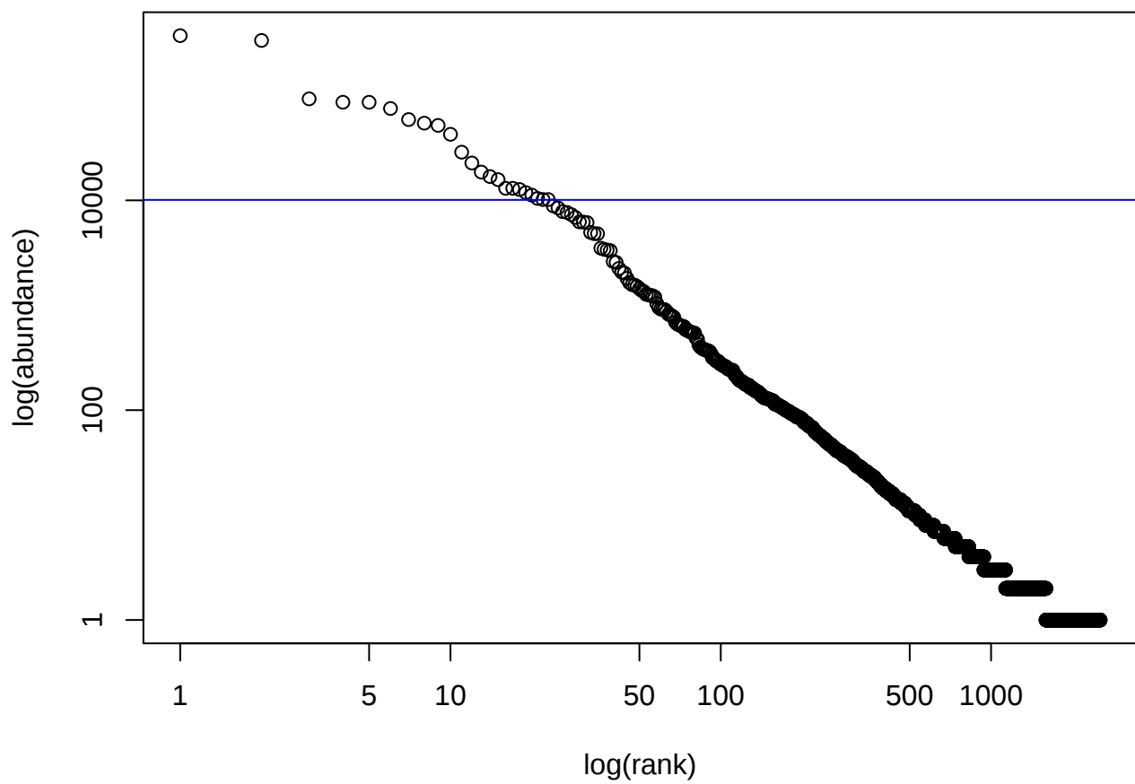
TARA_094.SUR.20.180.DNA
