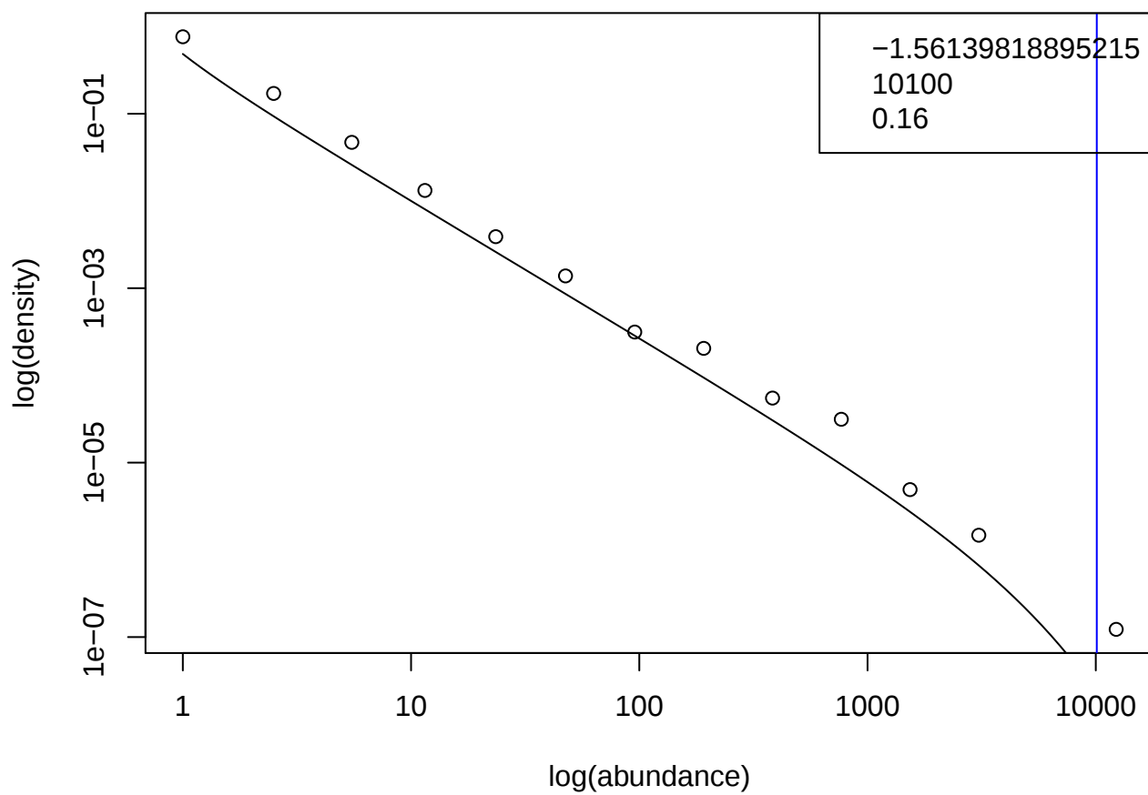
TARA_006.SUR.180.2000.DNA
