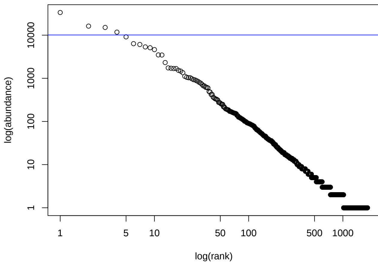
TARA_099.SUR.20.180.DNA
