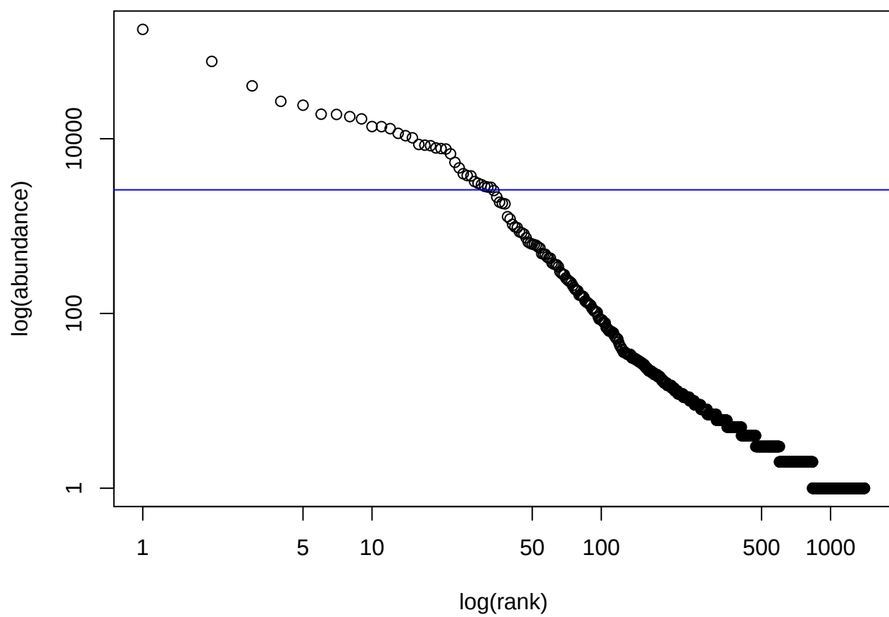
TARA_086.SUR.20.180.DNA
