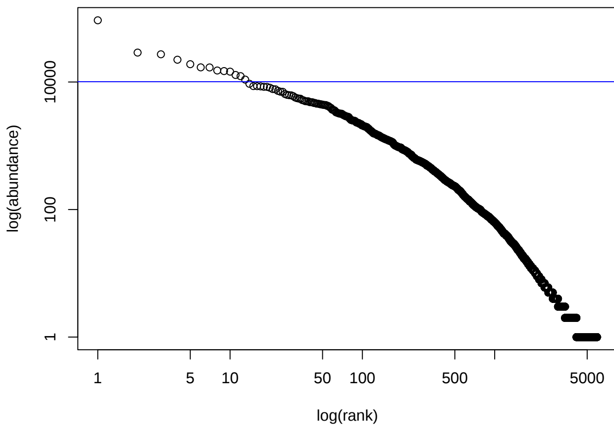
TARA_007.SUR.0.8.5.DNA
