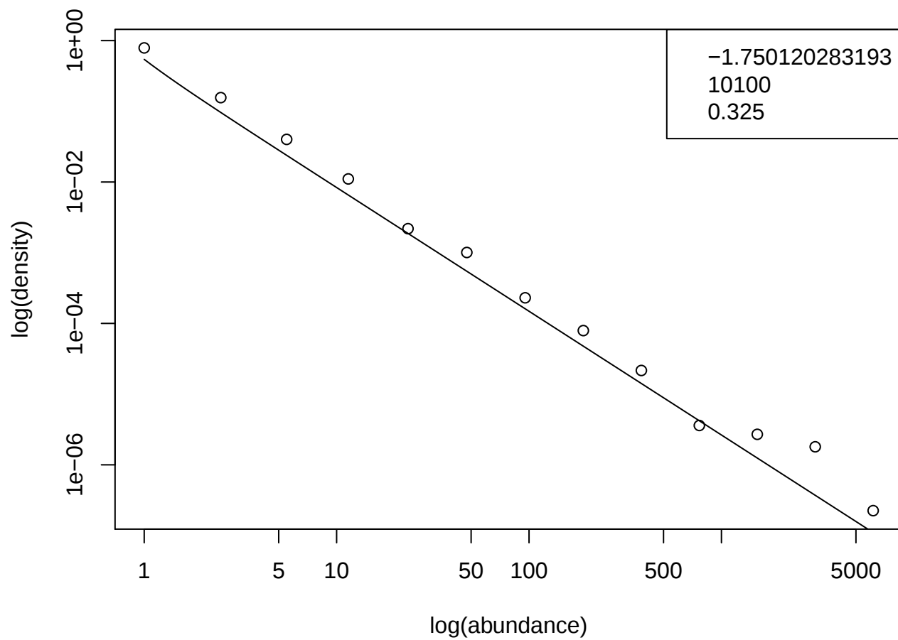
TARA_143.SUR.180.2000.DNA
