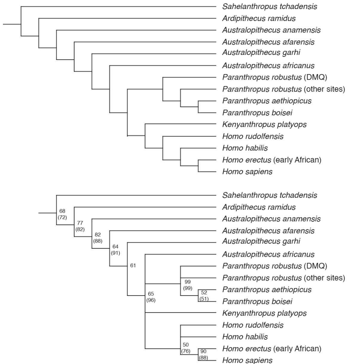
Supplementary Figure 6. Results of maximum parsimony analysis. a, Most parsimonious cladogram. b, 50% majority rule consensus tree derived from bootstrap analysis. Numbers at internal nodes indicate bootstrap support for the corresponding clade. Numbers in parentheses indicate bootstrap support for the clade when K. platyops and Au. garhi (both of which are missing data with respect to many characters) are excluded from the analysis.
