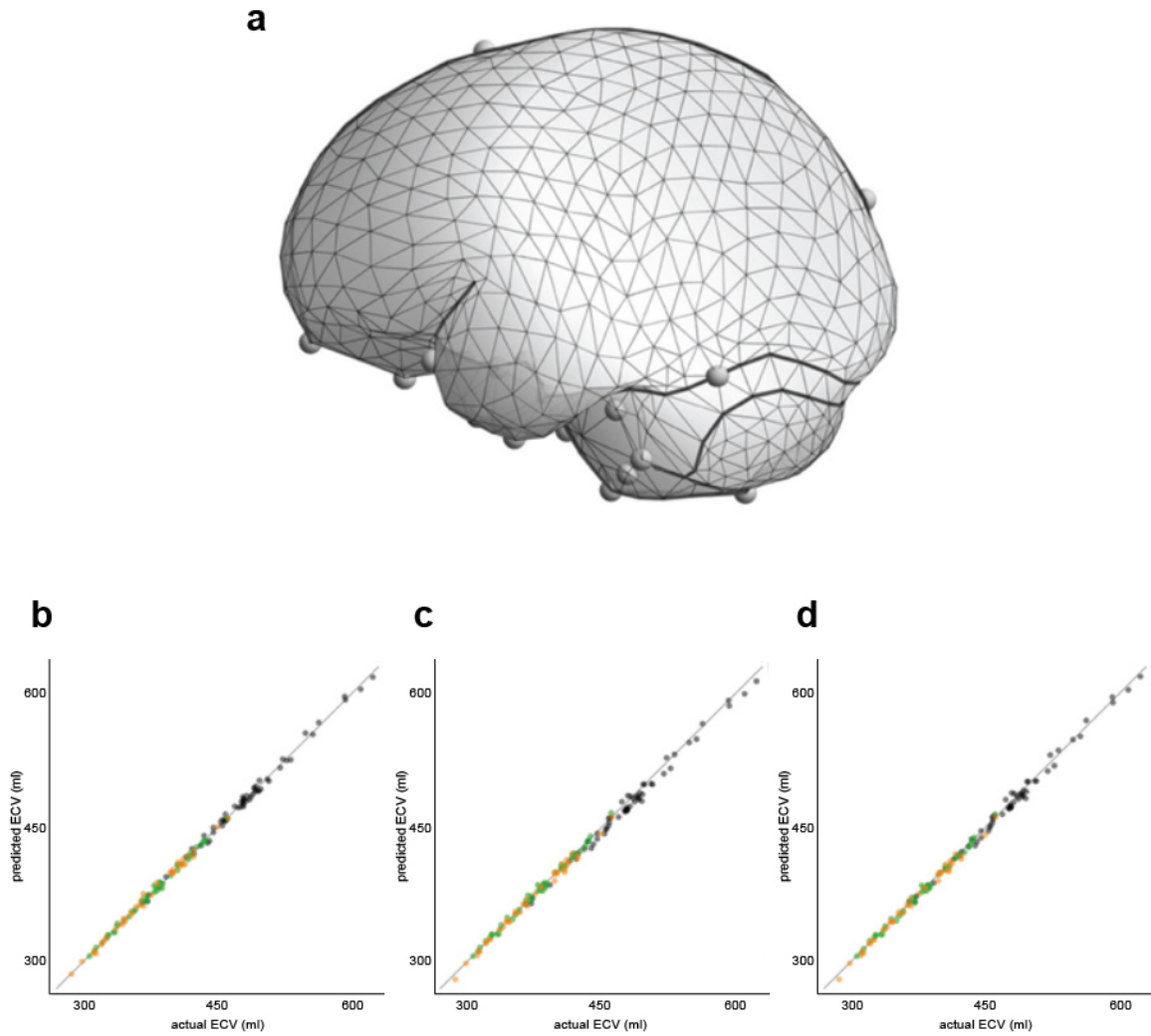
Supplementary Figure 5. Endocranial volume estimation of DNH 155. a , Endocranial landmark set used for ECV estimation. Each vertex of the surface is used as a landmark or semilandmark. Anatomical landmarks are shown as spheres, curve semilandmarks are connected as black lines. b – d , Simulations based on reference sample: measured versus predicted ECV [ b , regression-based, c , pooled TPS-based and d , species-specific TPS-based estimates] for gorillas (grey), orang-utans (orange), chimpanzees (green).
