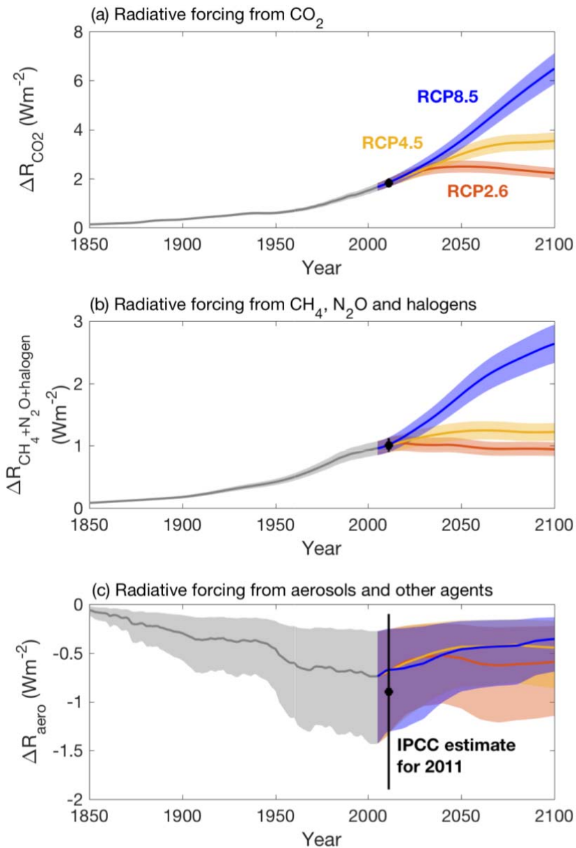
Supplementary Fig. 2. The radiative forcing for the observation-consistent ensemble over time and from observational estimates for 2011. The radiative forcing over time in the efficient Earth system model is drawn from the RCP scenarios 5 , but where each component is modified by an uncertainty which is retained over time (Supplementary Table 2). Included here are the median (line) and 95% range (shaded regions) for observation-consistent ensemble simulations over time and for the IPCC estimates for 2011 from Ref. 2.
