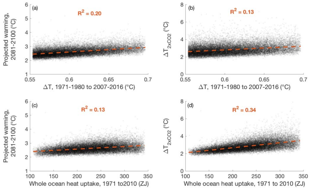
Supplementary Fig. 4: Simulated historical constraints against future projected warming and \Delta T_{2xCO_2} for RCP4.5. Scatterplots from the observationally-consistent ensemble: for the projected warming for year 2081 to 2100 versus (a) the surface temperature change \Delta T from decade 1971-1980 to 2007-2016 and (c) the global ocean heat content change (ZJ) from year 1971 to 2010; and the equilibrium climate sensitivity, \Delta T_{2xCO_2} (°C) versus (b) the surface temperature change \Delta T and (d) the global ocean heat content change [as in (a) and (b)]. The values of the correlation coefficient between the variables are included (Supplementary Table 8). Each point (grey dot) represents a single simulation in the observation-consistent ensemble, while the red dashed lines are the best fit.
