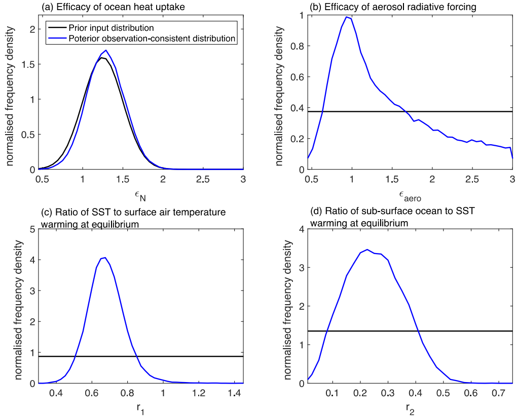
Supplementary Fig. 3: Prior and posterior distributions of efficacies and ratios in the standard experiment for RCP8.5. Normalised frequency distributions of model parameters in the initial prior 10^8 model simulations (black) and in the posterior distribution of the 3 \times 10^4 observation-consistent simulations (blue) (a) The distributions of the efficacy of heat uptake, \epsilon_N , (b) the distributions of efficacy of aerosol radiative forcing, \epsilon_{aero} , (c) the distributions of the ratio of warming in sea surface temperatures to surface air-temperatures at equilibrium, r_1 , and (d) the distributions of the ratio of warming in the sub-surface ocean to sea surface temperatures at equilibrium.
