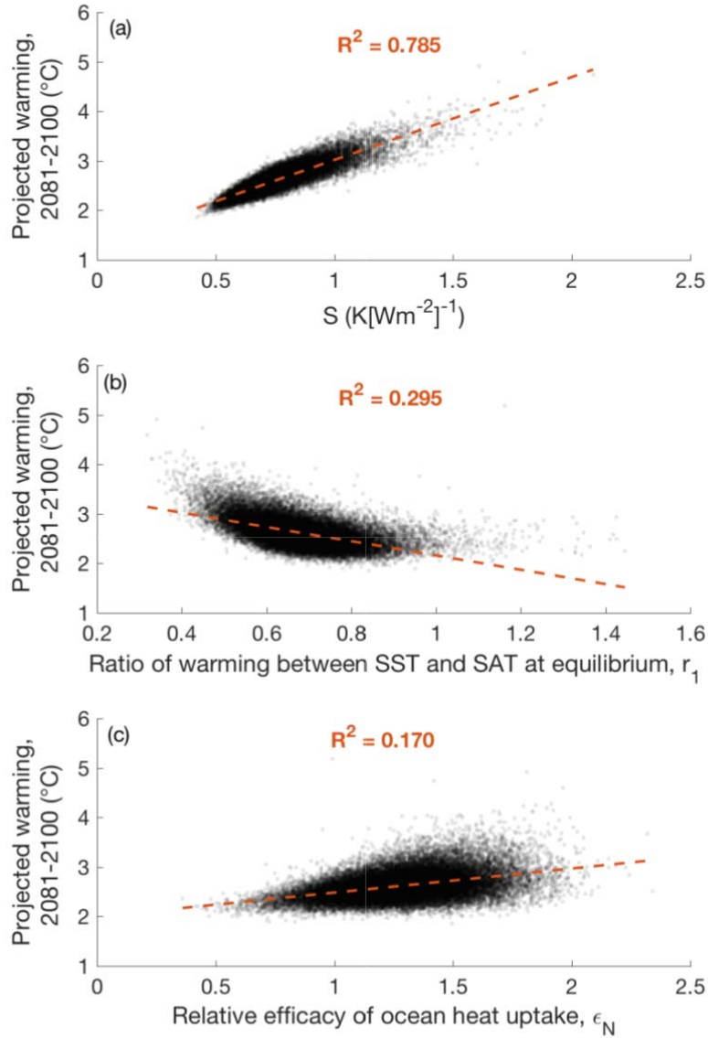
Supplementary Fig. 5: Model parameter input values against future projected warming for RCP4.5. Scatterplots from the observationally-consistent ensemble for the projected warming for year 2081 to 2100 versus (a) the climate sensitivity, S , (b) the ratio of warming at equilibrium for global sea surface temperatures compared to global surface air temperatures, r_1 and (c) the relative efficacy of ocean heat uptake, \epsilon_N . The values of the correlation coefficient between the variables are included (Supplementary Table 9). Each point (grey dot) represents a single simulation in the observation-consistent ensemble, while the red dashed lines are the best fit.
