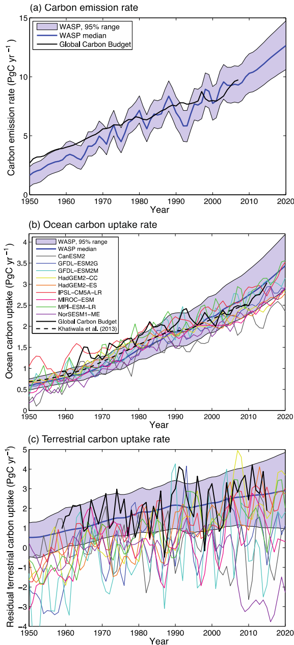
Supplementary Fig. 1. Carbon fluxes and upper ocean heat uptake from observations, Earth system AR5 models and our observation-consistent ensemble of conceptual Earth system model simulations (a) Compatible fossil fuel carbon emissions from observations and model re-analysis (black), the observation consistent ensemble of conceptual Earth system model (WASP) simulations (blue: thick blue line median, blue shading 95% range). The annual carbon fluxes into the (b) ocean and (c) terrestrial systems for observations, the observation consistent ensemble and nine Earth system models from Supplementary Table 1 (lines as legend on panel b). Carbon emission and flux observations in (a)-(c) from The Global Carbon Budget and Khatiwala et al. (Ref. 60) are as collated in Ref. (24), with additional original data therein also deriving from Refs. (58-59).
