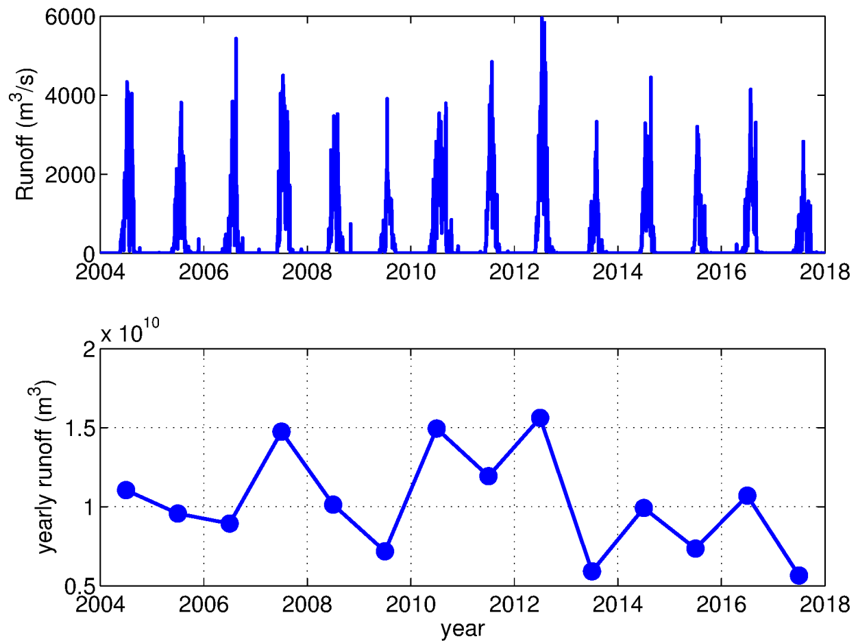
Supplementary Figure 16 | Subglacial discharge as estimated by RACMO2.3p2. Daily subglacial discharge (top panel) and the yearly-integrated values (bottom panel). Data are estimated using RACMO2.3p2 at 1 km resolution as discussed in the text. These were used as input for the plume model, in combination with temperature and salinity in Disko Bay as well as depth of the glacier at the calving front to compute the melting rate at the front.
