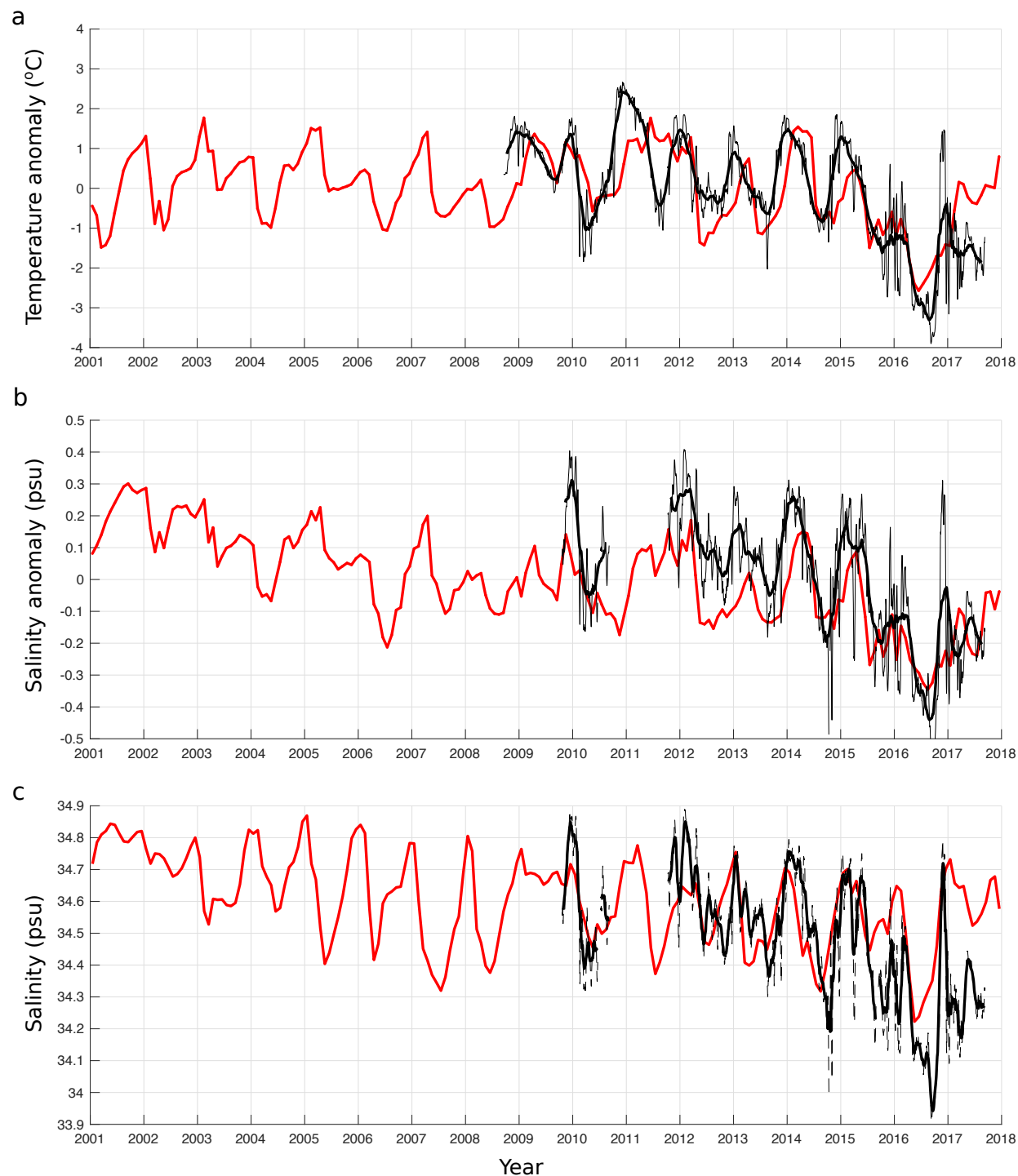
Supplementary Figure 12 | Temperature and salinity anomalies relative to 2009-2017 mean and the salinity at site of Davis Strait moorings. a, and b, Site is at point D in Supplementary Fig. 11. Red: ECCO state estimate; black: mooring data (heavy) 31-day boxcar averaged, (thin) 7-day boxcar averaged. We show the anomalies here because the ECCO state
