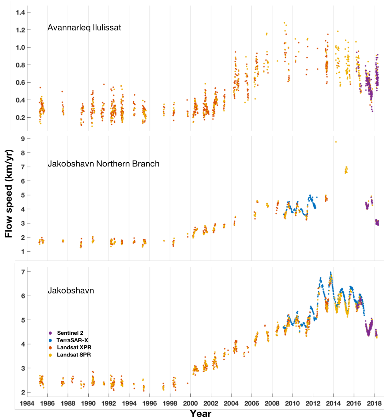
Supplementary Figure 6 | Flow speeds of the three main glaciers terminating in Ilulissat Icefjord. Glacier locations are shown in Supplementary Fig. 1. Time series extend from March 1985 to May 2018. Data are color coded by remote-sensing source and processing approach (XPR: Cross Path Row processing; SPR: Same Path Row processing).
