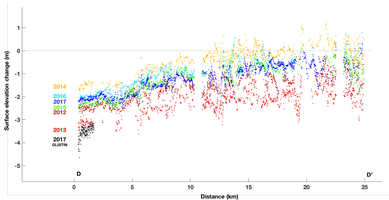
Supplementary Figure 5 | Surface elevation changes in a slow-moving ice area. Changes in elevation are along the path DD' (Supplementary Fig. 1), which traverses an area of slow-moving ice (slower than 200 m/yr). We use these measurements to constrain the contribution of surface processes such as precipitation and melting to observed surface elevation changes. Changes in elevation for each year shown are found relative to the preceding year. The uncertainty of the data is discussed in Methods.
