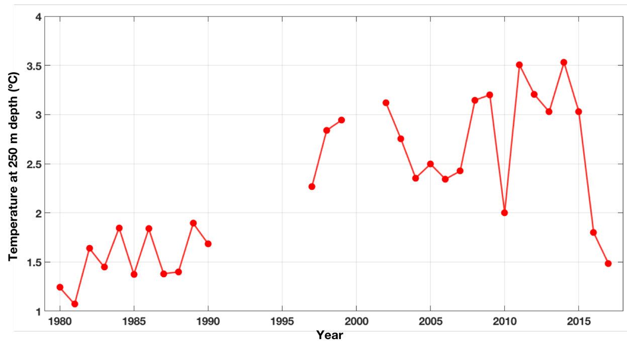
Supplementary Figure 8 | Temperatures in Disko Bay. As in Supplementary Fig. 7, but only for the depth at 250 m, which is the depth of the sill at the mouth of the fjord. Note that temperatures at 250-m depth have not been this cold since at least the early 1990s, and possibly since the late 1980s.
