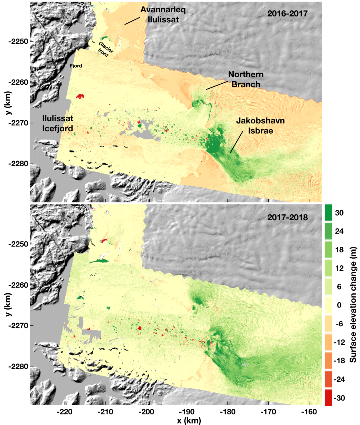
Supplementary Figure 4 | Surface elevation changes of Jakobshavn Isbrae, its Northern Branch and Avannarleq Ilulissat glacier. Changes in surface elevations for the periods 2016-2017 and 2017-2018 of the three main glaciers terminating in Ilulissat Icefjord. Measurements are by GLISTIN (Methods), and changes are obtained by subtracting the elevations of the earlier year from those of the latter. The color scale of elevation changes applies to both panels. The locations of the glaciers are shown in the inset of Supplementary Fig. 1.
