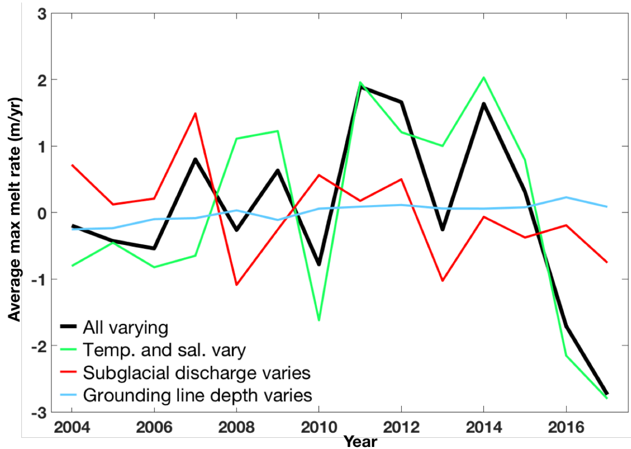
Supplementary Figure 17 | Sensitivity of plume model results to various inputs. Average of the maximum melt rate over a melt season for several different runs of the plume model. The time mean of each time series has been removed, since confidence in the model is highest for year-to-year variations. In the primary run, which was used for comparison with glacier response, temperature and salinity profiles at the glacier front, the depth below sea level of the glacier at the calving front or grounding line, and subglacial discharge were all allowed to vary from year to year. In the three other runs, two of these inputs were held constant at their mean values for each year and only one of these inputs was allowed to vary.
