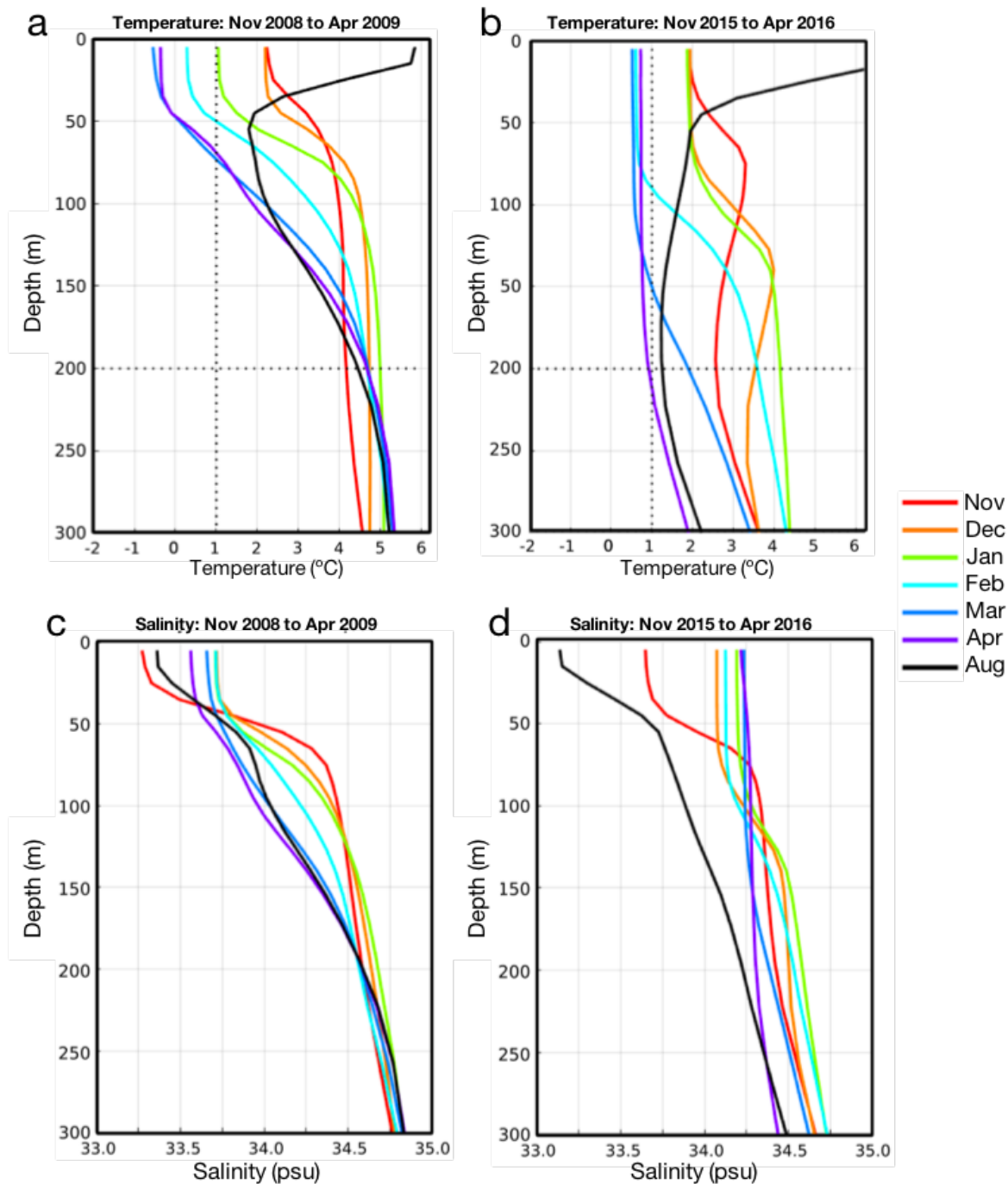
Supplementary Figure 15 | Evolution (Nov-Aug) of temperature (a-b) and salinity (c-d) at location C from the ECCO state estimate in two different years. The two years show distinct progression of mixed layer deepening and upper ocean cooling through winter (Nov-Mar). Winter 2009 (a, c) shows a mixed layer deepening to 50 m in Mar-Apr and cooling in upper 50 m by 2.5°C and little temperature change at 200 m (4.1°C in Nov). In contrast, the winter 2016 shows the evolution of a much deeper mixed layer (to ~220 m), and large cooling through the mixed layer of about 1.5°C. At 200-250 m, 2016 temperatures reach 1°C in Apr and remain close to 1°C in August. Relative to the 2001-2018 average, the 2015 initial upper ocean stratification (not shown) is weaker and temperatures in the upper 200 are colder.
