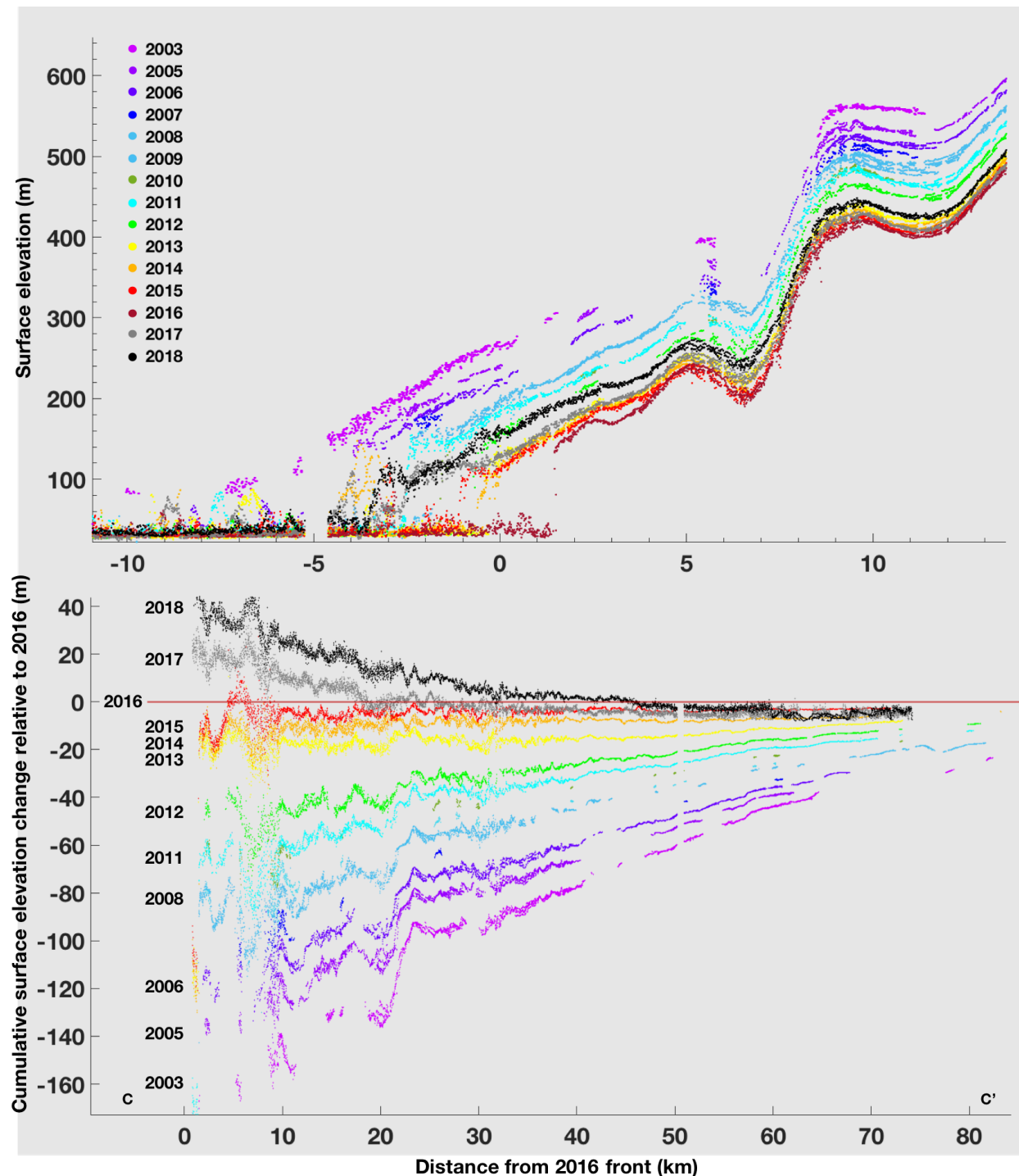
Supplementary Figure 2 | Jakobshavn Isbrae's surface elevation changes. Top panel shows elevations (relative to the WGS84 ellipsoid) of the lower reaches of the glacier during the period 2003-2018. The legend applies to both panels. Bottom panel depicts the cumulative changes in surface elevations. Change in elevation for each year is found relative to the year 2016, by subtracting the elevation of the earlier year from that of the latter. The path CC' (Supplementary Fig. 1) extends 80 km inland from the 2016 front. Data for the years 2003 to 2016 are from ATM observations, while the years 2017 and 2018 are from GLISTIN. During years missing from the time series the ATM track did not overlap with that of 2016. No smoothing is applied to the data. The uncertainty of the data is discussed in Methods.
