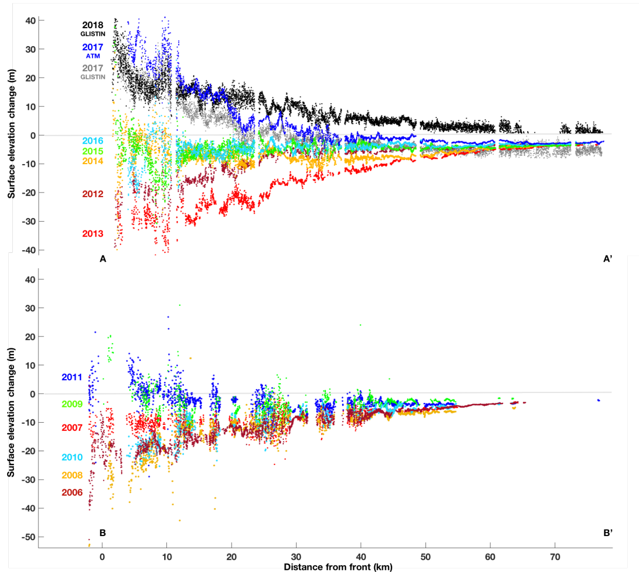
Supplementary Figure 3 | Surface elevation changes along the main trunk of Jakobshavn Isbrae. Changes in elevation for each year shown are found relative to the preceding year. The distance along path AA' is relative to the point where the 2017 ATM track intersects the 2017 front (Fig. 1; dates are given in Supplementary Table 1). Similarly, the distance along path BB' is relative to the point where the 2011 ATM track intersects the 2011 front (Fig. 1; dates are given in Supplementary Table 1). We interpolated the GLISTIN observations of elevation change (Fig. 1) along the 2017 ATM path, as shown in the top panel. The top panel is the same as in Fig. 2, except that no smoothing is applied here, and that we show the 2017 ATM data. The 2018 ATM data were not available at the time of writing. The uncertainty of the data is discussed in Methods.
