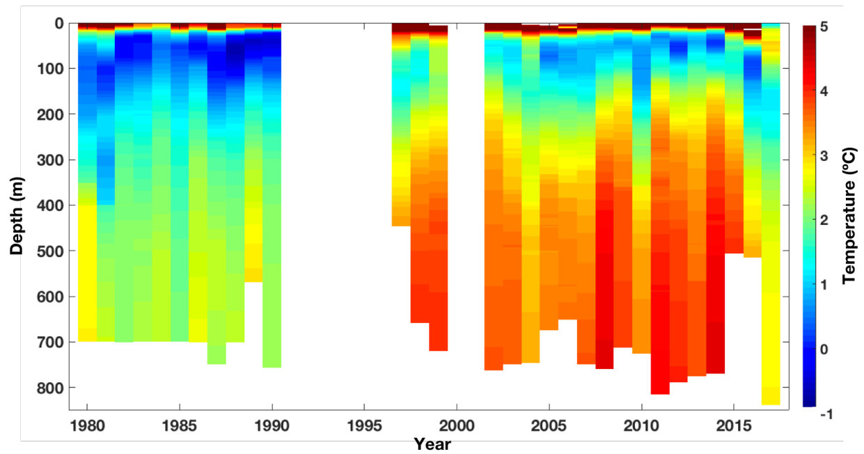
Supplementary Figure 7 | Temperatures in Disko Bay. Average temperatures in Disko Bay from CTD profiles collected in the locations indicated by the orange dots in Fig. 1b in the main text. Note the rapid cooling of the deep warm layer near the end of the time series.
