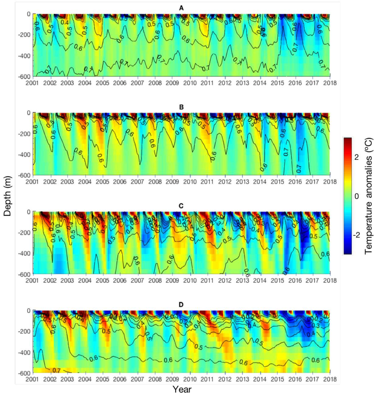
Supplementary Figure 14 | Depth-time evolution of temperature anomalies at the four sites A-D (shown in Supplementary Fig. 11) from the ECCO state estimate. Anomalies at each depth are relative to the mean over the period 2001 to 2017. Surface-referenced potential density contours, \rho_0 -1027 kg/m 3 , are overlaid. Large wintertime (DJFM) air-sea heat fluxes in 2015 across the entire subpolar gyre induce cold anomalies at all points. Temperatures at A partially recover but remain 0.6° cooler than average. Points B-D are downstream of A and also show significantly reduced temperature recovery through 2015. Total 2016 Wintertime cooling at C and D drive temperatures to the coldest temperatures seen over the 2001-2018 period. Importantly, between B-D temperatures below 100 m do not recover as normal between spring and fall in 2016.
