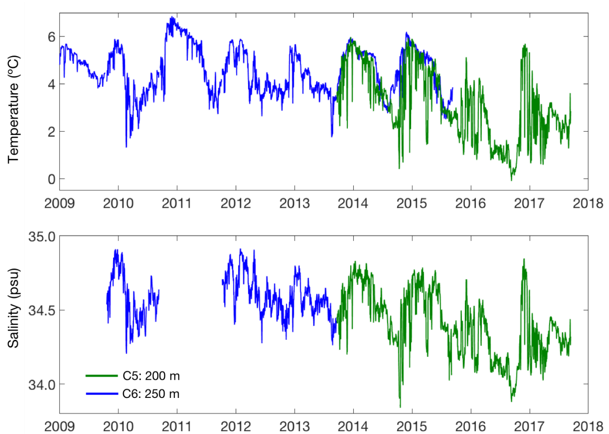
Supplementary Figure 10 | Temperature and Salinity in Davis Strait. Observations of daily-averaged temperature and salinity in Davis Strait at the location of two mooring (C5 and C6, shown as red dots in Fig. 3a of the main text). Although the C5 record is at 200 m depth and that of C6 is at 250 m depth, their variability is closely related and they are at the relevant depths to sample water at the correct density to make it over the sill and into Ilulissat Fjord (see ref. 8 , Figure 2).
