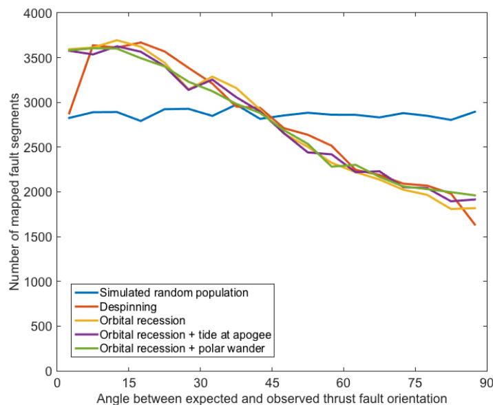
Figure S5. Comparison of observed and expected local thrust fault orientations for different stress models. An angle of 0^\circ indicates fault segments that are orthogonal to local direction of most compressive stress, and 90^\circ indicates fault segments that are parallel to most compressive stress.
