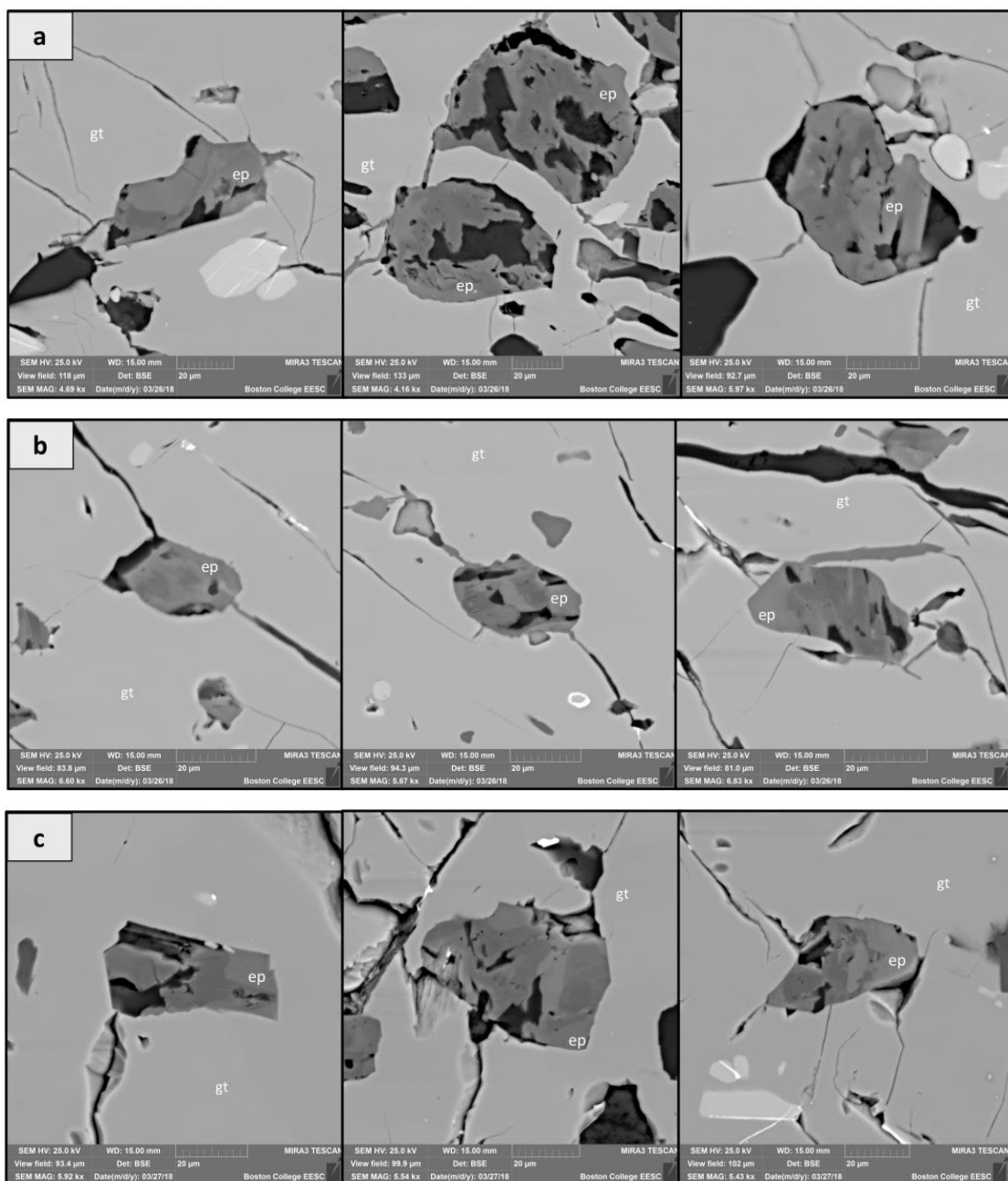
Supplementary Figure 5: BSE images of epidote inclusion in samples A) 09DSF-23E, B) 09DSF-54A, and C) 06MSF-6C so show epidote inclusions thought to be pseudomorphs after lawsonite. Epidote inclusions such as these display chemical zoning and are associated with albite or paragonite, products of lawsonite breakdown. As a result, these and all similar epidote inclusions were not used in oxygen barometry calculations. Abbreviations used include gt = garnet and ep = epidote.
