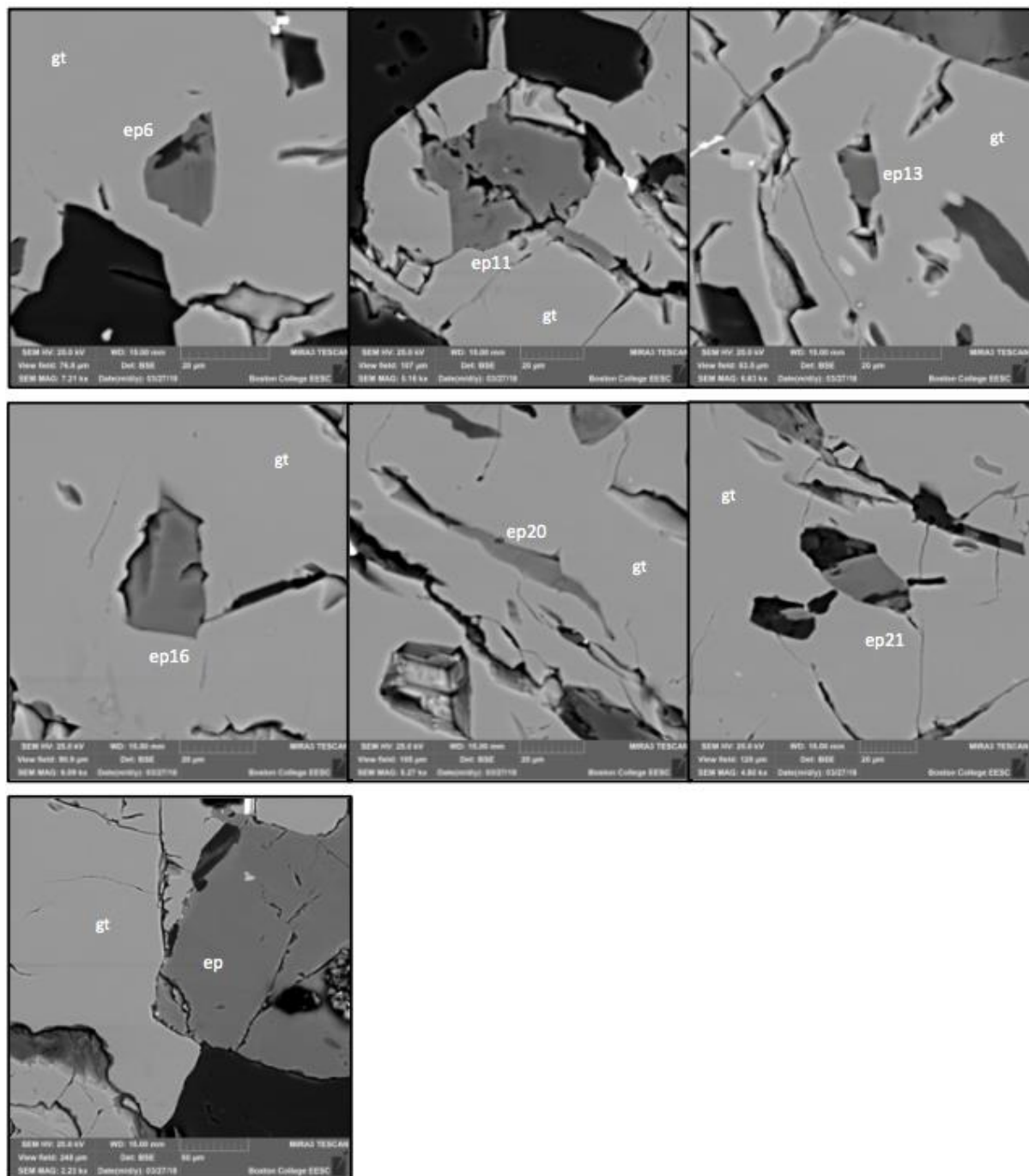
Supplementary Figure 4: BSE images of each epidote inclusion in sample 06MSF-6C used in oxygen barometry calculations.
