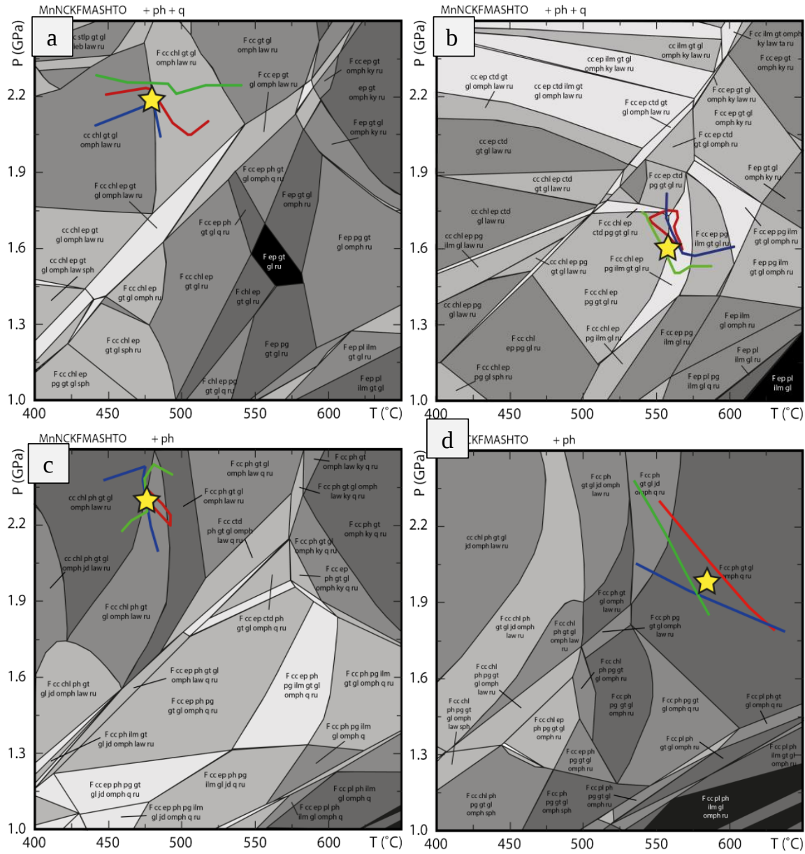
Supplementary Figure 7: Equilibrium phase diagram sections used for calculation of core and rim P - T conditions for samples 09DSF-23E and 09DSF-54A. Phase diagrams (A) and (C) use whole rock bulk compositions for calculation of P - T conditions corresponding to core growth for samples 09DSF-23E and 09DSF-54A respectively. Phase diagrams (B) and (D) were calculated using matrix bulk compositions to estimate the P - T conditions for growth of the garnet rims (Supplementary Table 3) for samples 09DSF-23E and 09DSF-54A respectively. Garnet chemical isopleths corresponding to observed garnet core and rim chemistry (Supplementary Table 4) are plotted (almandine=red, grossular=green, spessartine=blue). Intersection of garnet core isopleths constrains the P - T of garnet nucleation and intersection of garnet rim isopleths constrains the P - T of garnet rim growth. Mineral assemblages are labeled using the following abbreviations: gt = garnet; ep = epidote; law = lawsonite; chl = chlorite; ph = phengite; omph = omphacite; q = quartz; ru = rutile; jd = jadeite; gl = glaucophane; ilm = ilmenite; pl = plagioclase; cc = carbonate; F = fluid; sph = sphene; ctd = chloritoid; pg = paragonite; ky = kyanite.
