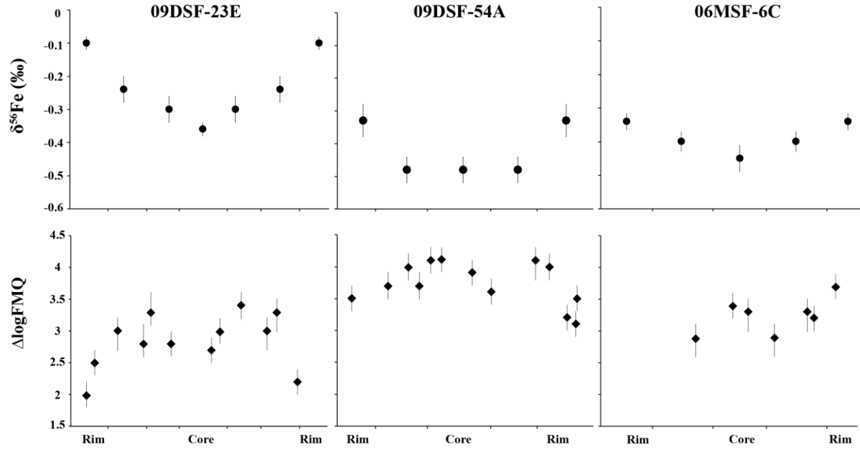
Supplementary Figure 1: \Delta\log\text{FMQ} and the \delta^{56}\text{Fe} values plotted from rim-core-rim in one garnet grain from samples 09DSF-54A, 09DSF-23E, 06MSF-6C. Error calculations for the \delta^{56}\text{Fe} data are the two-standard deviation of four isotopic analysis for each sample. Errors for the \Delta\log\text{FMQ} values are \pm 0.2 log units for the core and rim points, calculated using the \pm 1\text{kbar} and \pm 40^\circ\text{C} errors associated with P - T estimates from thermodynamic modeling 30 . The errors for the \Delta\log\text{FMQ} of the intermediate zones are calculated accounting for the slightly larger uncertainty in the P - T conditions and were calculated using upper and lower bounds for the possible P - T conditions (see further discussion in methods section and calculations in Supplementary Table 5).
