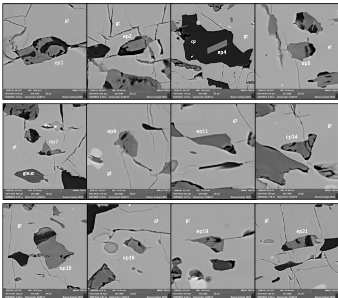
Supplementary Figure 2: BSE images of each epidote inclusion in sample 09DSF-23E used in oxygen barometry calculations.
