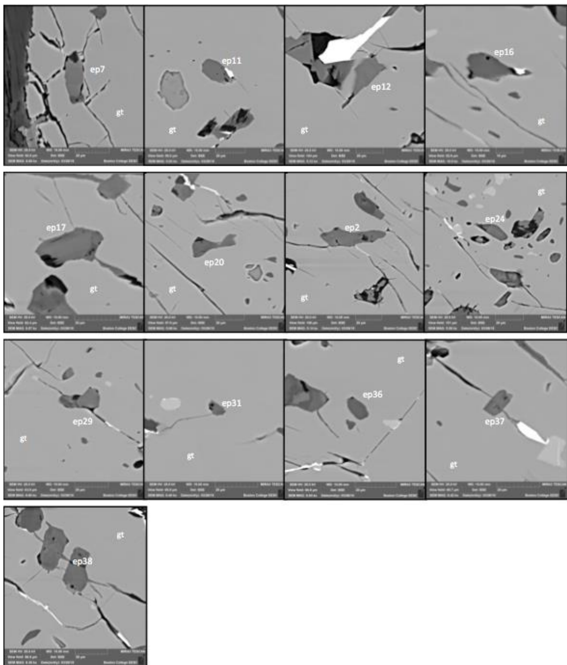
Supplementary Figure 3: BSE images of each epidote inclusion in sample 09DSF-54A used in oxygen barometry calculations.
