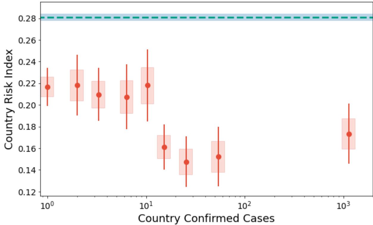
Supplementary Fig. 6: A second aggregated view of the evolution of the risk index for increasing numbers of confirmed cases. Differently from Fig. 4, here we compute the average risk index for a single day in each country (instead of the cumulative value). We first compute the average value for days with no confirmed cases, which is 0.28 (blue line in figure). We then aggregate all days with confirmed cases in homogeneous bins and compute the average values (red points). We observe that reporting of the first case is associated with a drop in the risk index, followed by a second significant drop in correspondence of 10 confirmed cases, supporting what was observed in Fig. 4. All shaded areas represent the s.e.m of the average risk index, error bars encode the 95% confidence intervals.
