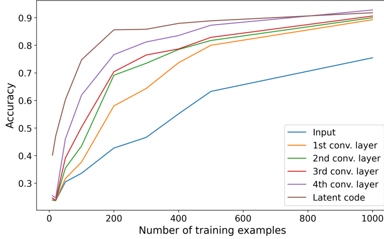
Figure 2: Latent representations support few-shot category learning. The accuracy of an object shape classifier on a held-out test set is shown for different amounts of training data, with different layers of the VAE as input features. The classifier is a simple support vector machine as in Figure 2a.
