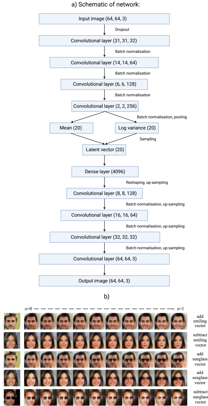
Figure 3: Additional model details. a) Variational autoencoder architecture. Trainable layers (plus the input, output, and sampled latent vector) are shown in boxes, along with the dimensions of their outputs, and non-trainable operations such as activation functions, batch normalisation, and upsampling are shown as annotations. See the SI for more details. b) Figure adapted from Hou et al. 4 with permission, showing the effect of adding and subtracting a proportion \alpha of various different vectors in the latent space of their VAE. (Diagrams were created using BioRender.com.)
