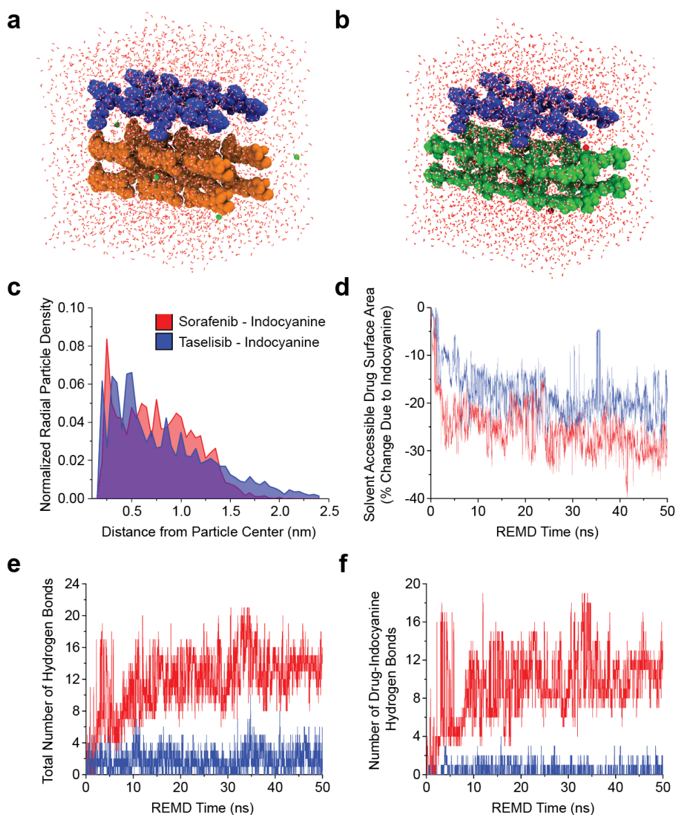
Supplementary Figure 12. Molecular dynamics simulations of indocyanine nanoparticles.
