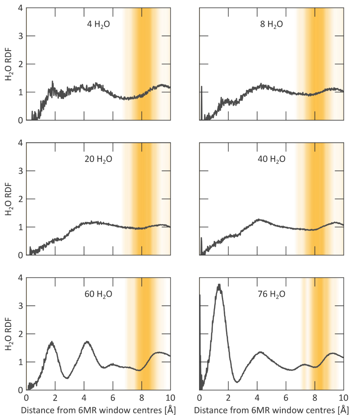
Supplementary Figure 43 | Radial distribution functions at various water loadings at 300 K and 50 MPa. RDFs between (i) the centres of the 6MR apertures and the oxygens of the water molecules (grey trace) and (ii) the centres of the 6MR apertures (orange shade).
