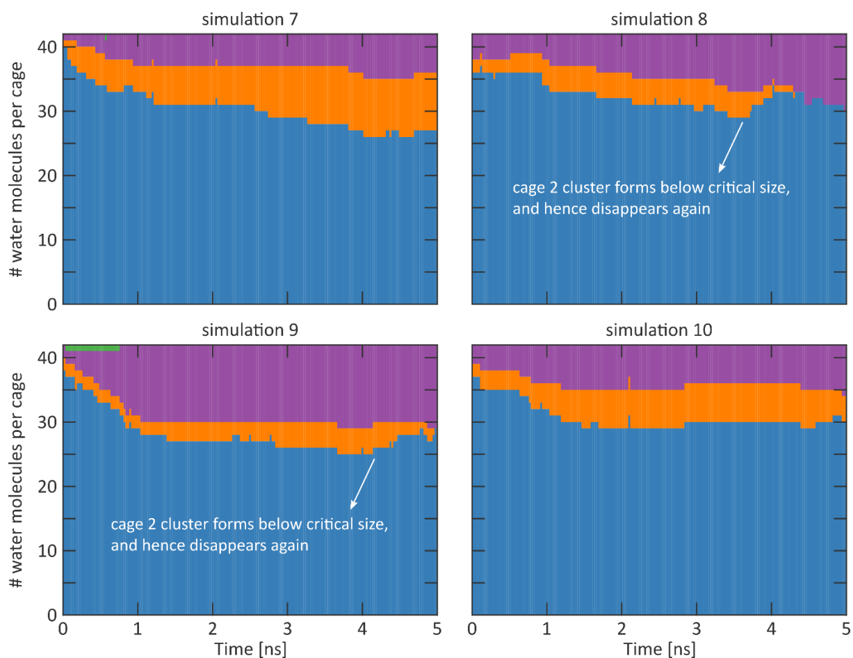
Supplementary Figure 64 | Evolution of the number of water molecules per cage during a 5 ns MD simulation at 300 K and 0 MPa of a 1\times 1\times 2 ZIF-8 supercell with an inhomogeneous water distribution. All simulations initially contained 42 water molecules in cage 1 while all other cages were initially empty. These simulations were initialised with different initial velocities for the water molecules, which were drawn randomly from a Maxwell-Boltzmann distribution at 300 K. The cage indexing is identical to Figure 4a of the main text. Figure continued from Supplementary Figure 63.
