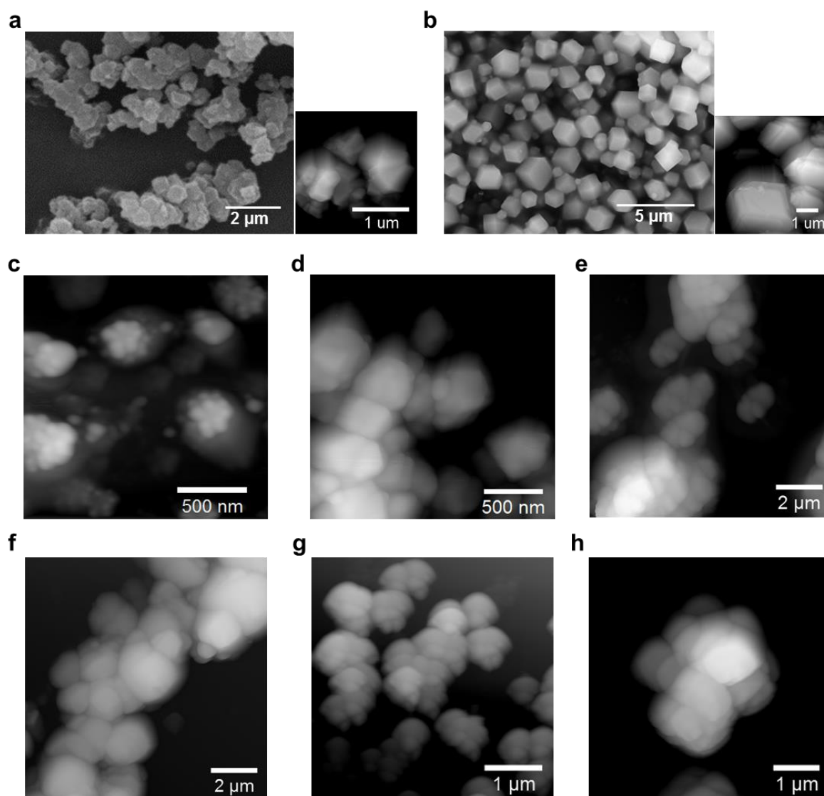
Supplementary Figure 3 | AFM and SEM images of the ZIFs before water intrusion. a, ZIF-8 (left: SEM, right: AFM), b, ZIF-71 (left: SEM, right: AFM), c, ZIF-7, d, ZIF-9, e, ZIF-67. f, ZSM-5, g, zeolite- \beta , h, mordenite. ZIF-7 and ZIF-9 are the guest-free phase II samples, 4 and the three zeolite samples are after the heating treatment at 1,000 ^{\circ}\text{C} .
