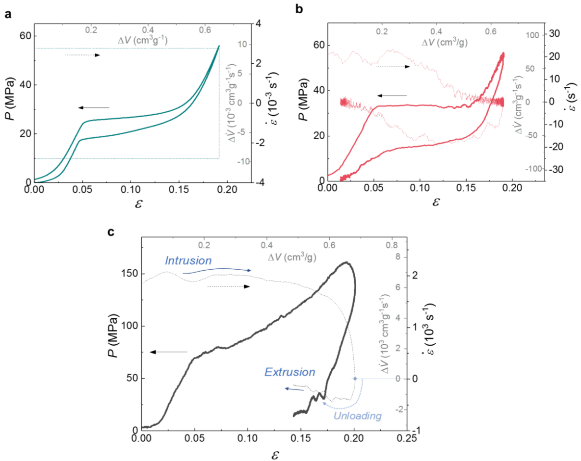
Supplementary Figure 12 | Water intrusion and extrusion of ZIF-8. a , Low-rate, b , medium-rate, and c , high-rate conditions, corresponding to the result of Figure 2b-c in the main text. Solid lines represent the pressure; dashed lines represent the corresponding strain rate.
