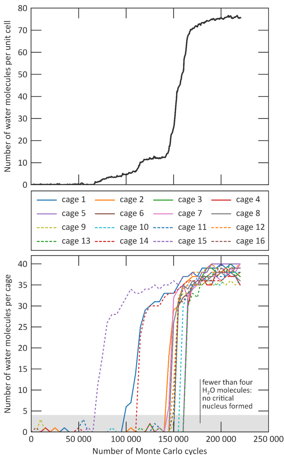
Supplementary Figure 82 | Filling of the ZIF-8 cages during a grand canonical Monte Carlo simulation: (top) averaged over a 2×2×2 supercell, (bottom) for each of the 16 cages separately. Results obtained at a water pressure of 6 kPa and a temperature of 298 K. The top figure corresponds with Supplementary Figure 23.
