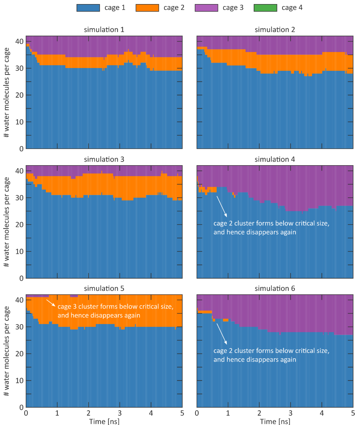
Supplementary Figure 63 | Evolution of the number of water molecules per cage during a 5 ns MD simulation at 300 K and 0 MPa of a 1\times 1\times 2 ZIF-8 supercell with an inhomogeneous water distribution. All simulations initially contained 42 water molecules in cage 1 while all other cages were initially empty. These simulations were initialised with different initial velocities for the water molecules, which were drawn randomly from a Maxwell-Boltzmann distribution at 300 K. The cage indexing is identical to Figure 4a of the main text. Figure continued in Supplementary Figure 64.
