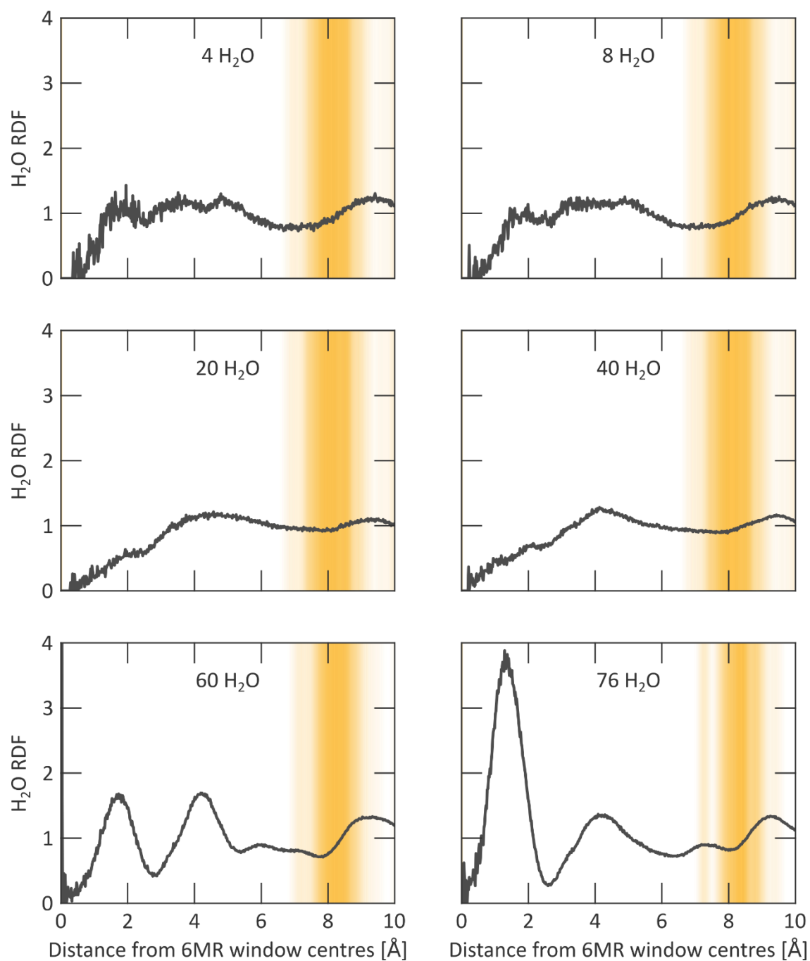
Supplementary Figure 44 | Radial distribution functions at various water loadings at 300 K and 60 MPa. RDFs between (i) the centres of the 6MR apertures and the oxygens of the water molecules (grey trace) and (ii) the centres of the 6MR apertures (orange shade).
