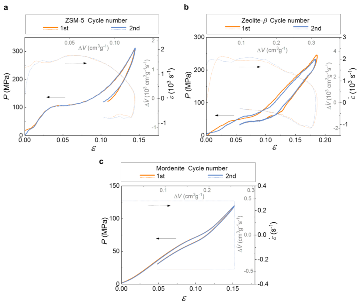
Supplementary Figure 91 | Cyclic water intrusion and extrusion of the channel-containing zeolites.
