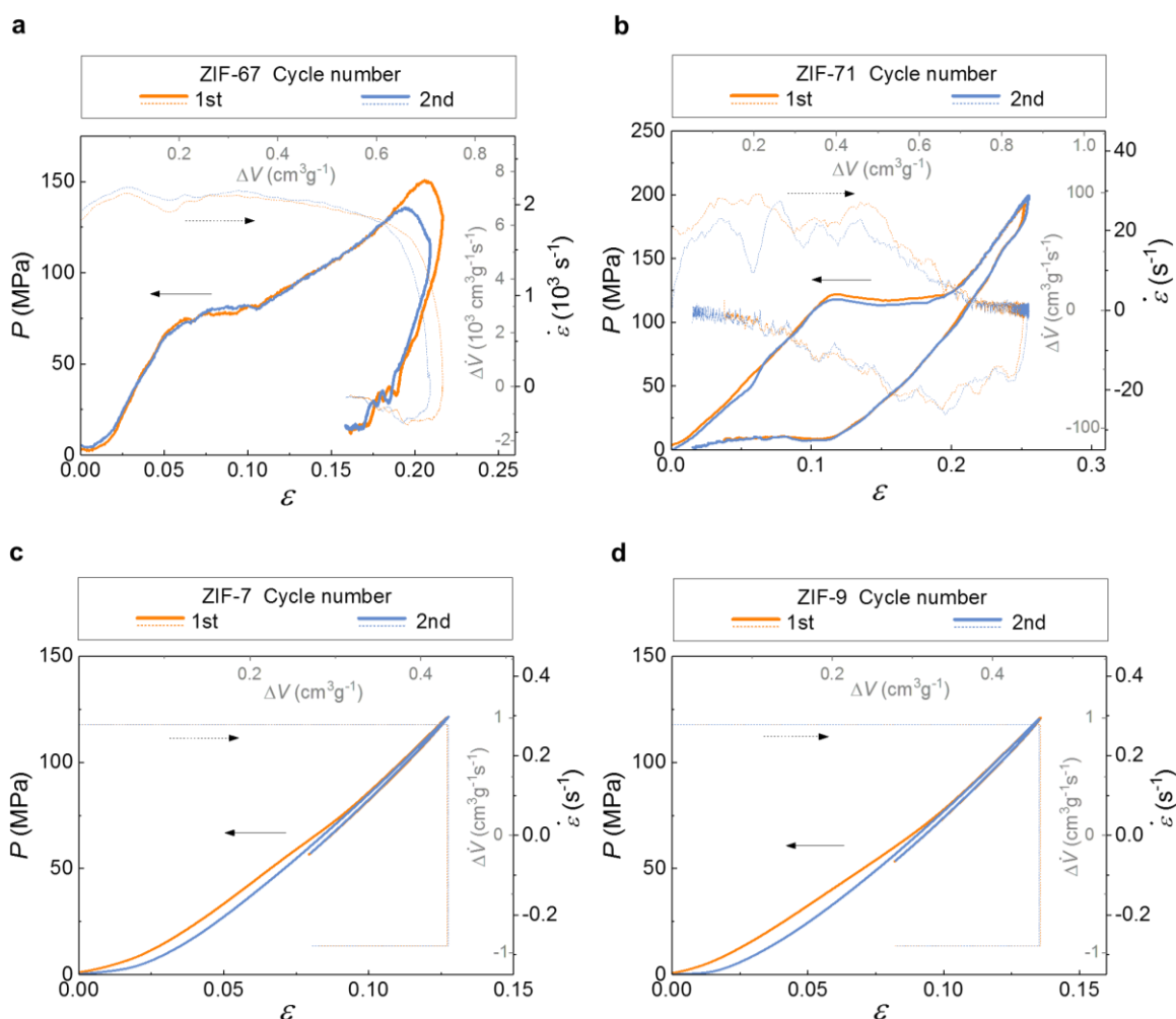
Supplementary Figure 16 | Cyclic water intrusion and extrusion of different ZIF materials. a, ZIF-67 at high strain rate, b, ZIF-71 at medium strain rate, c, ZIF-7 at 0.3 s -1 , and d, ZIF-9 at 0.3 s -1 .
