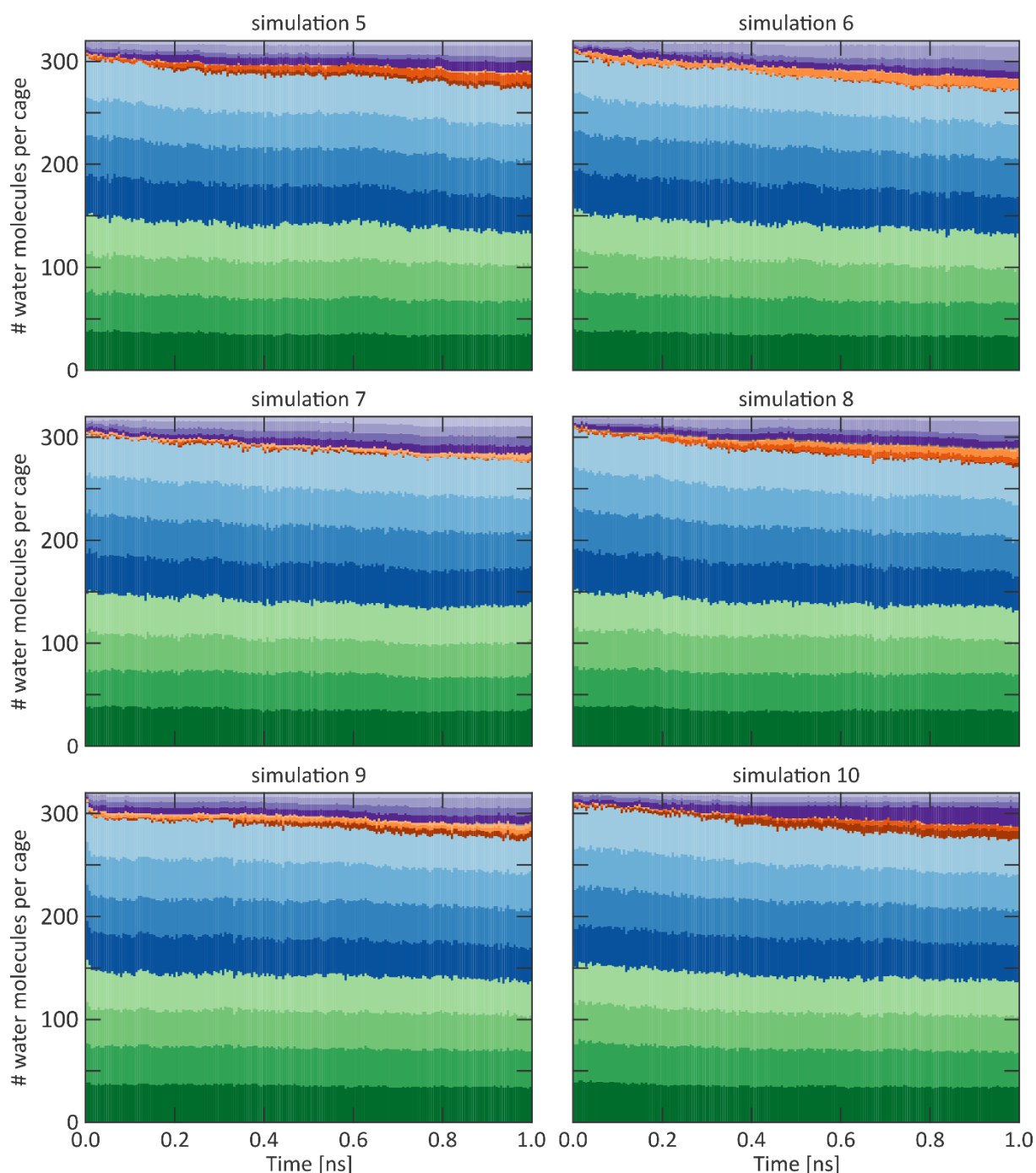
Supplementary Figure 74 | Evolution of the number of water molecules per cage during a 1 ns MD simulation at 300 K and 0 MPa of a 2 \times 2 \times 12 ZIF-8 supercell with an inhomogeneous water distribution in which two layers, corresponding to a 2 \times 2 \times 1 ZIF-8 supercell, were initially filled. All filled layers initially contained 40 water molecules per cage, while all other cages were initially empty, leading to a total of 320 water molecules in the system. These simulations were initialised with different initial velocities for the water molecules, which were drawn randomly from a Maxwell-Boltzmann distribution at 300 K. The cage indexing and colouring follows the scheme outlined in Supplementary Figure 66. Figure continued from Supplementary Figure 73.
