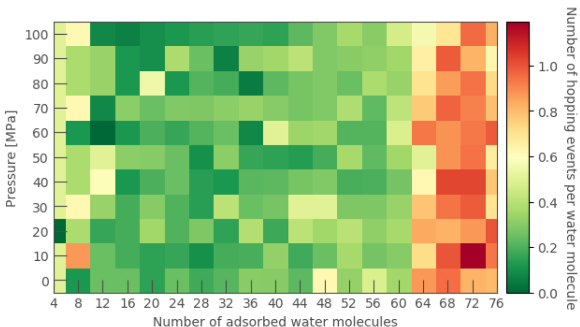
Supplementary Figure 50 | Relative water hopping frequency. Number of water hopping events counted between the two cages in the conventional ZIF-8 unit cell during a 5 ns ( N, P, \sigma_a = \mathbf{0}, T ) simulation as a function of the mechanical pressure and the water loading, normalised on the amount of water molecules present in the unit cell.
