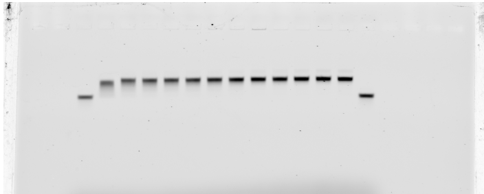
Octahedron 20 mM
