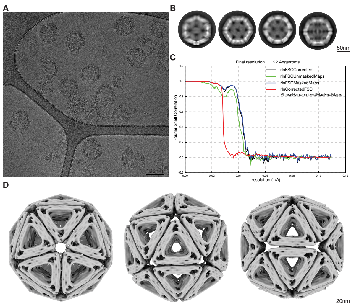
Supplementary Figure 14 | Cryo-EM reconstruction of the T=1 shell at 25 mM \text{MgCl}_2 . (A) Cryo-EM micrograph of T=1 shells on a lacey carbon grid with carbon support. (B) Two-dimensional class averages showing different orientations. (C) Graph showing different FSC curves which were used for resolution estimation. (D) Electron density map shown from the 5-fold, 3-fold and 2-fold symmetry axis (left to right, respectively).
