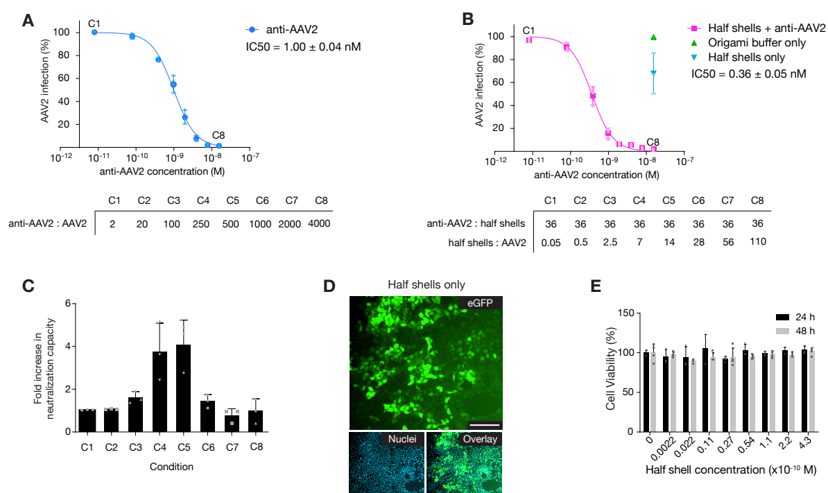
Supplementary Figure 35 | Dose-response characterization of neutralization capacity and cell viability. Complete IC 50 curves for both free antibody (anti-AAV2, A ) and origami half shells + anti-AAV2 ( B ). Concentration of half shells + anti-AAV2 in ( B ) is normalized to the concentration of anti-AAV2. Origami buffer only and half shell only conditions do not contain anti-AAV2, but the respective data points are positioned for easy visualization. Concentration of the half shells only is identical to that used in the highest half shell + anti-AAV2 condition. Below each graph is the approximate number of anti-AAV2 antibodies, and number of half shells, per AAV2 virus particle. All ratios are based on the total number of virus particles. Data in ( A ) and ( B ) is presented as mean ± s.d., n = 3 biologically independent experiments. Individual data points are overlaid. ( C ) Fold-increase in neutralization capacity that is achieved by conjugation of the anti-AAV2 antibody to the origami half shells, for each of the concentrations in the IC 50 curves ( A ) and ( B ), denoted as C1–C8. Data is presented as mean ± s.d., n = 3 biologically independent experiments. Individual data points are overlaid. ( D ) Representative epifluorescent images demonstrating expression of eGFP by infected cells for origami half shells without conjugated anti-AAV2. Images are representative from one of n = 3 biologically independent experiments, with similar results each time, scale bars represent 100 μm. ( E ) Viability of HEK293T cells exposed to half shell origami structures for 24 h and 48 h. Half shell concentrations are identical to those used in the IC 50 characterization ( B ). Exposure of HEK293T cells to the DNA origami half shells did not result in dose-dependent toxicity. Data is presented as mean ± s.d., n = 3 and 4 biologically independent experiments, for 24 h and 48 h respectively. Individual data points are overlaid.
