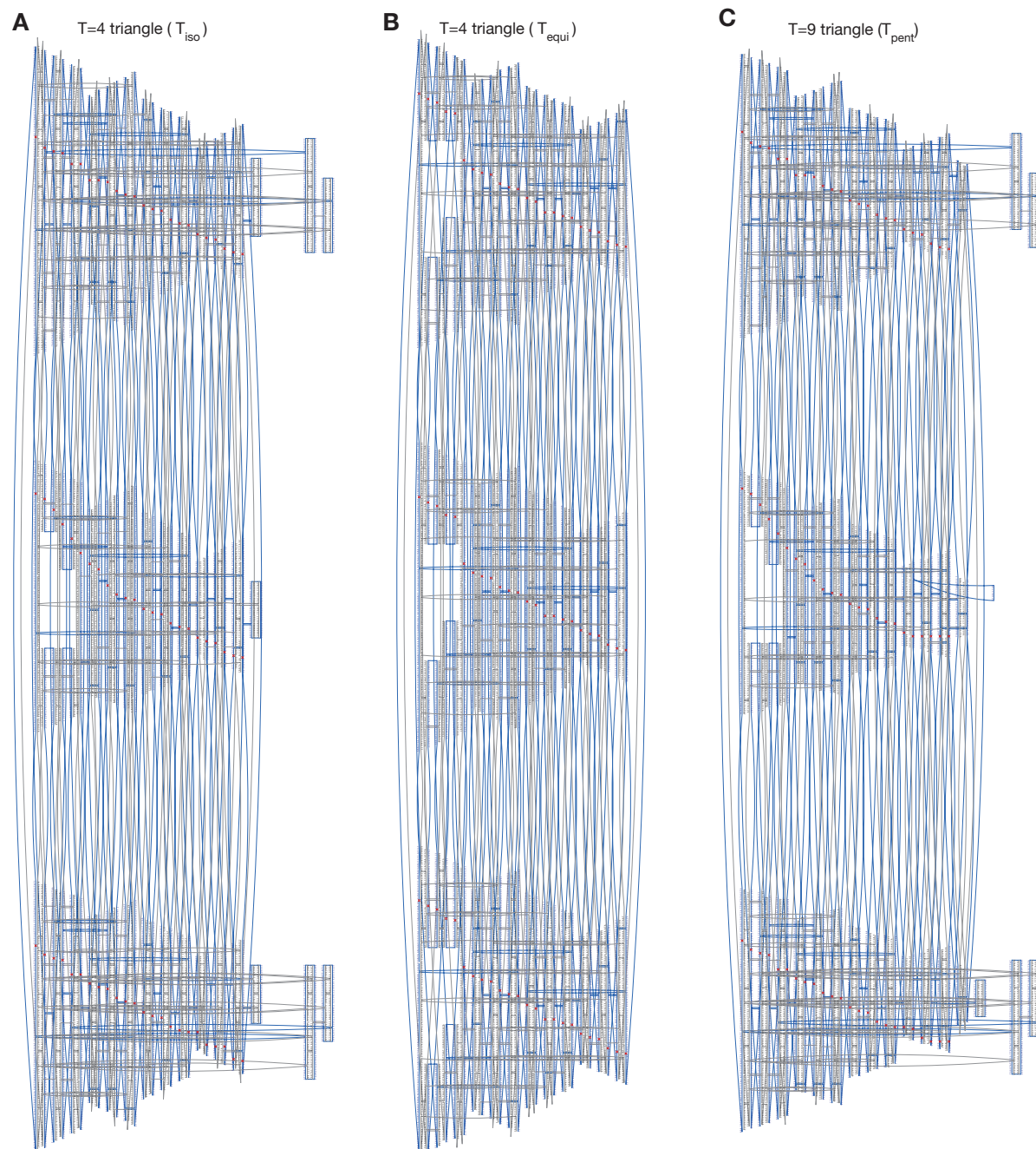
Supplementary Figure 39 | Design diagram of T=4 triangles and T_{pent} prepared with caDNAno v0.1. Oligonucleotides that connect two different sides have five additional single-stranded thymidines at the corner.
