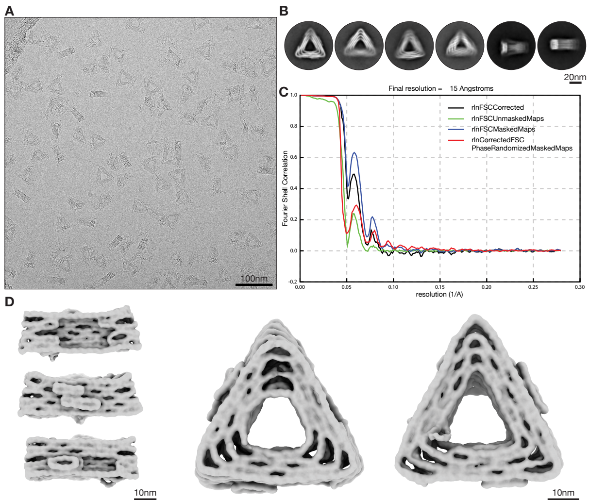
Supplementary Figure 10 | Cryo-EM reconstruction of the T=9 triangle T_{\text{hex}2} . (A) Cryo-EM micrograph of the T_{\text{hex}2} triangle in free-standing ice. (B) Two-dimensional class averages showing different orientations. (C) Graph showing different FSC curves which were used for resolution estimation. (D) Electron density map shown from different viewing angles.
