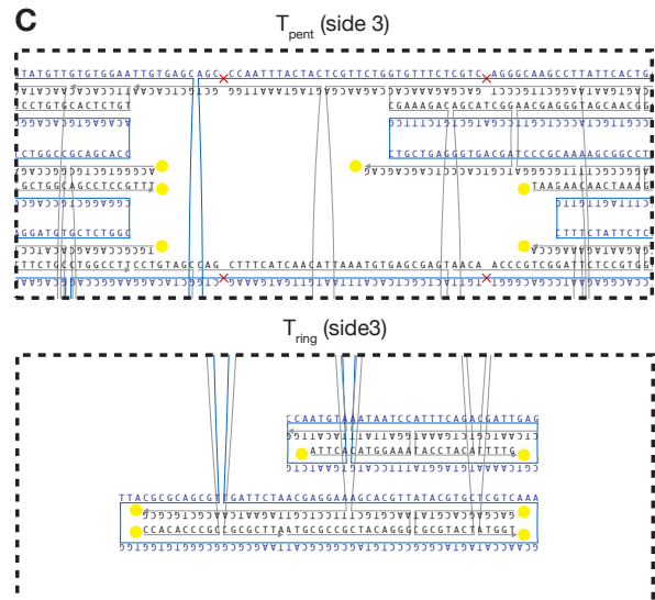
Supplementary Figure 45 | Design diagrams UV-welding at stacking contacts prepared with caDNAno v0.1. Protrusions and recesses have sticky overhangs and one optional, additional thymine base (yellow circle) for UV-welding in order to stabilize the partial shells in cell medium. (A) Protrusion and recess of the half octahedron (see Supplementary Fig. 42A). (B)+(C) Protrusion and recess of the half T=1 shell triangles T pent and T ring (see Supplementary Fig. 41C,D). Side 1 binds to side 2 (B) and side 3 of T pent to side 3 of T ring (C).
