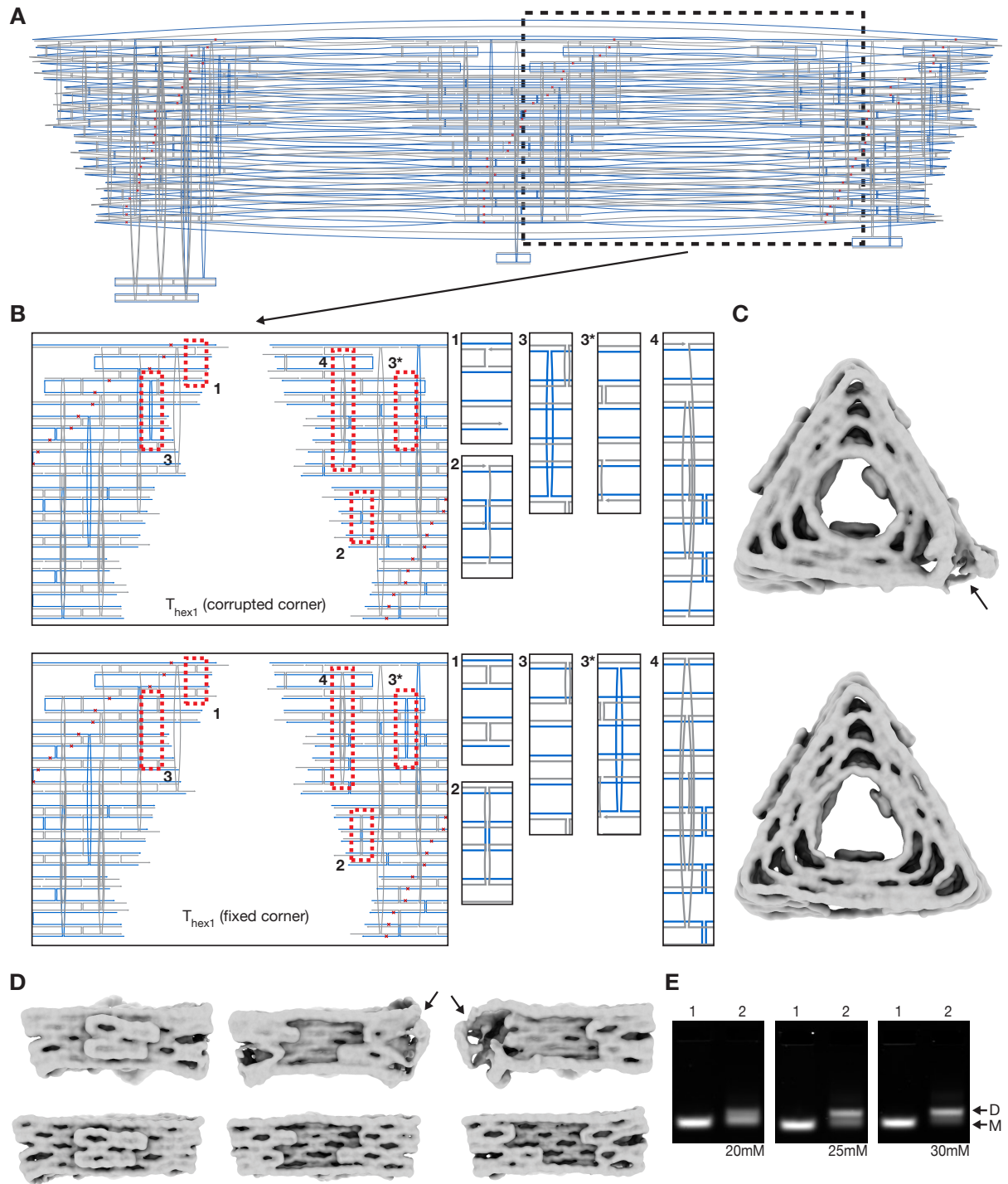
Supplementary Figure 11 | Correction for folding defects in T_{\text{hex1}} . (A) Design diagram of the T_{\text{hex1}} triangle with fixed corner. (B) Zoom-in on the location of the corrupted corner showing the differences between the two versions in the design diagram. (C and D) Cryo-EM map of the two T_{\text{hex1}} triangle versions. The arrows indicate the location of the corrupted corner. (E) 1.5% agarose gels with different \text{MgCl}_2 concentrations showing the dimerization of T_{\text{pent}} and T_{\text{hex1}} triangles. All sides not involved in the binding of the two triangles were passivated with polyT extensions at the stacking contacts. While the corrupted corner prevents the two triangles to bind to each other because of missing stacking contacts, the triangle with fixed corners binds to T_{\text{pent}} and assembles into dimers. Lane 1: T_{\text{pent}} + T_{\text{hex1}} (corrupted corner), Lane 2: T_{\text{pent}} + T_{\text{hex1}} (fixed corner). D: dimer, M: monomer.
