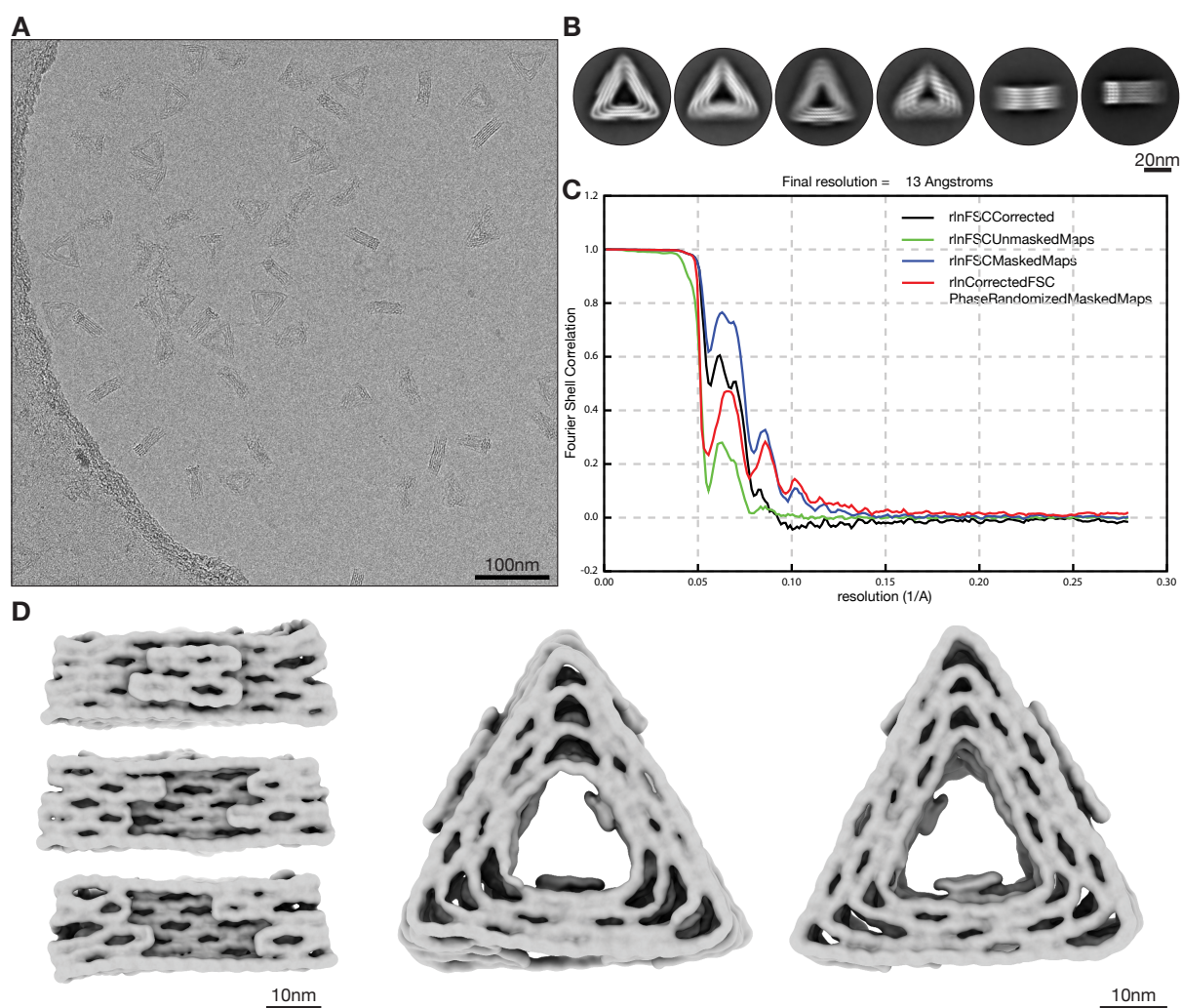
Supplementary Figure 9 | Cryo-EM reconstruction of the T=9 triangle T_{\text{hex1}} . (A) Cryo-EM micrograph of the T_{\text{hex1}} triangle in free-standing ice. (B) Two-dimensional class averages showing different orientations. (C) Graph showing different FSC curves which were used for resolution estimation. (D) Electron density map shown from different viewing angles.
