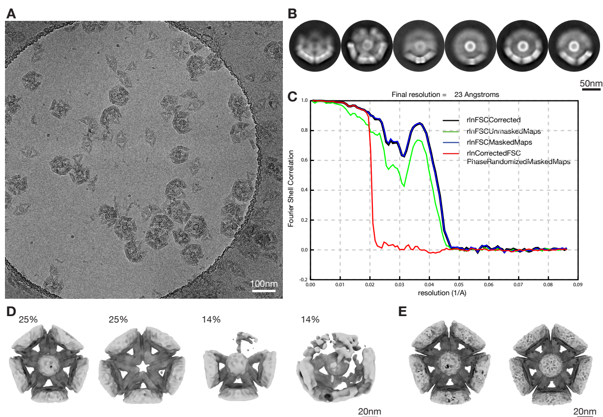
Supplementary Figure 33 | Cryo-EM reconstruction of the half T=1 shell with a trapped HBV core particle. (A) Cryo-EM micrograph of the half T=1 shell with a trapped HBV core particle in free-standing ice. (B) Two-dimensional class averages showing different orientations. (C) Graph showing different FSC curves which were used for resolution estimation. (D) Classes after 3d classification in relion3. (E) Refinement without (left) and with (right) using C5 symmetry.
