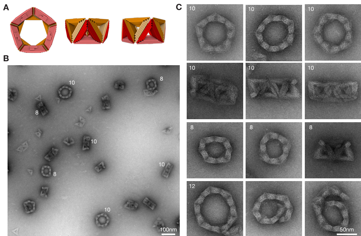
Supplementary Figure 29 | Negative stain TEM images of T_{\text{ring1}} and T_{\text{ring2}} . (A) Cylindrical model of the DNA-origami ring containing 10 triangles. (B) Negative stain images of rings formed by T_{\text{ring1}} and T_{\text{ring2}} assembled for 1d at 40°C ( c_{\text{triangle}}=10\text{nM} , c_{\text{MgCl}_2}=25\text{mM} ). The white numbers show the number of triangles within a ring. (C) Exemplary particles showing rings with 8, 10 or 12 triangles as well as not fully closed rings.
