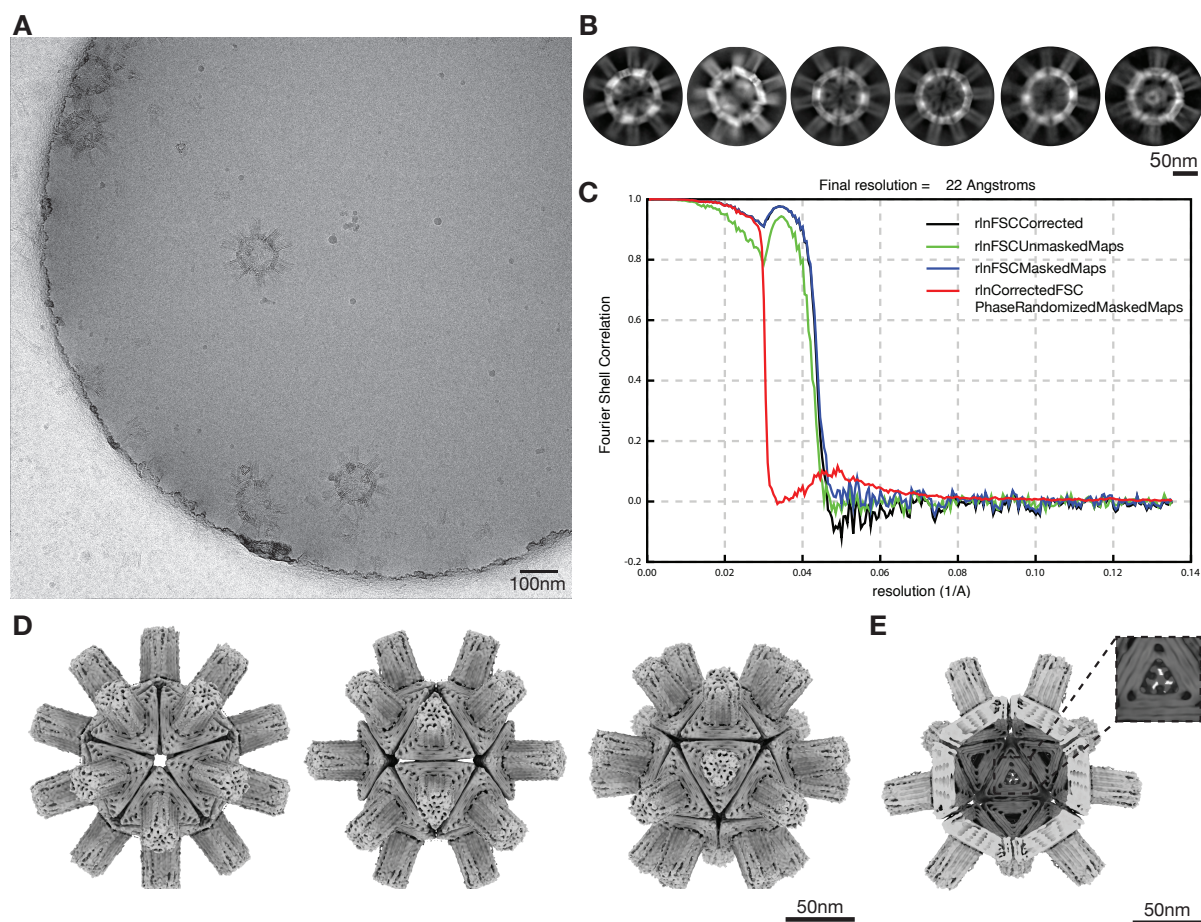
Supplementary Figure 21 | Cryo-EM reconstruction of the spiky shell at 22.5 mM MgCl 2 .
