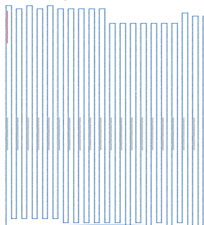
Supplementary Figure 43 | Design diagrams for modified T=1 shells prepared with caDNAno v0.1. (A) T=1 triangle with protruding oligonucleotides. (B) Triangular brick structure with connections sites. (C) Single-stranded scaffold with 20 handles for triangle (grey) and one handle for Cy5 (red) attachment.
