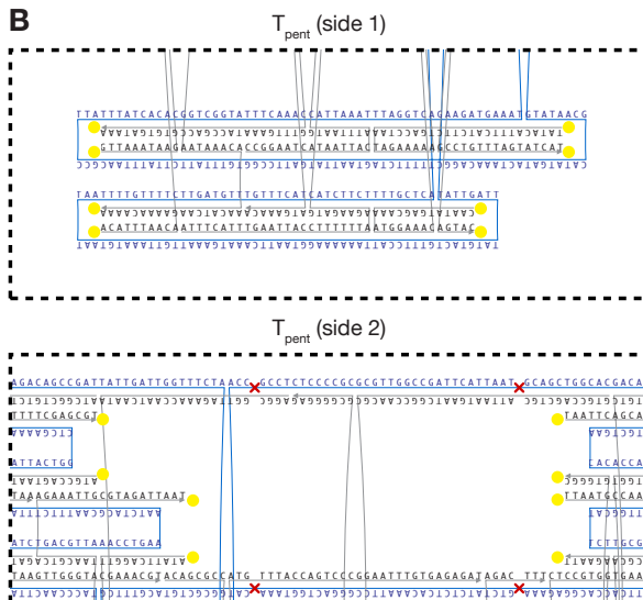
Supplementary Figure 45 | Design diagrams UV-welding at stacking contacts prepared with caDNAno v0.1. Protrusions and recesses have sticky overhangs and one optional, additional thymine base (yellow circle) for UV-welding in order to stabilize the partial shells in cell medium. (A) Protrusion and recess of the half octahedron (see Supplementary Fig. 42A). (B)+(C) Protrusion and recess of the half T=1 shell triangles T pent and T ring (see Supplementary Fig. 41C,D). Side 1 binds to side 2 (B) and side 3 of T pent to side 3 of T ring (C).
