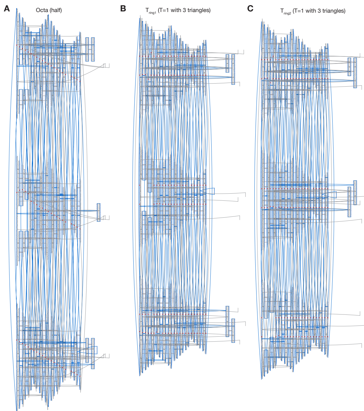
Supplementary Figure 42 | Design diagram of Octa and T=1 half-shell triangles prepared with caDNAno v0.1. Oligonucleotides that connect two different sides have five additional single-stranded thymidines at the corner. Every side is equipped with three handles for attaching the antibodies (seq.: GCAGTAGAGTAGGTAGAGATTAGGCA-oligo). The T ring1 and T ring2 triangles can assemble T=1 shells missing a pentagon vertex together with T pent triangles (Supplementary Fig. 25C, Supplementary Fig. 41A).
