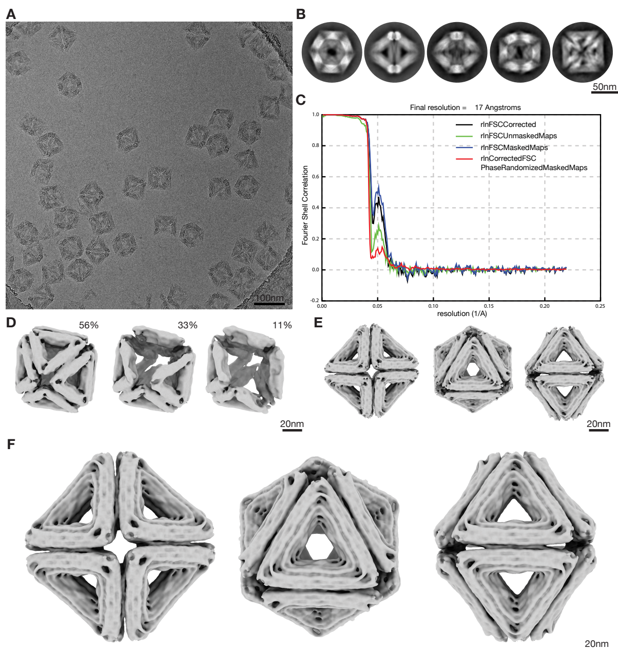
Supplementary Figure 12 | Cryo-EM reconstruction of the assembled octahedron at 17.5 mM \text{MgCl}_2 . (A) Cryo-EM micrograph of the octahedron in free-standing ice at 17.5 mM \text{MgCl}_2 . (B) Two-dimensional class averages showing different orientations. (C) Graph showing different FSC curves which were used for resolution estimation. (D) Classes after 3d classification in relion3. (E) Refinement without using any symmetry (C1). (F) Electron density map shown from the 4-fold, 3-fold and 2-fold symmetry axis (left to right).
