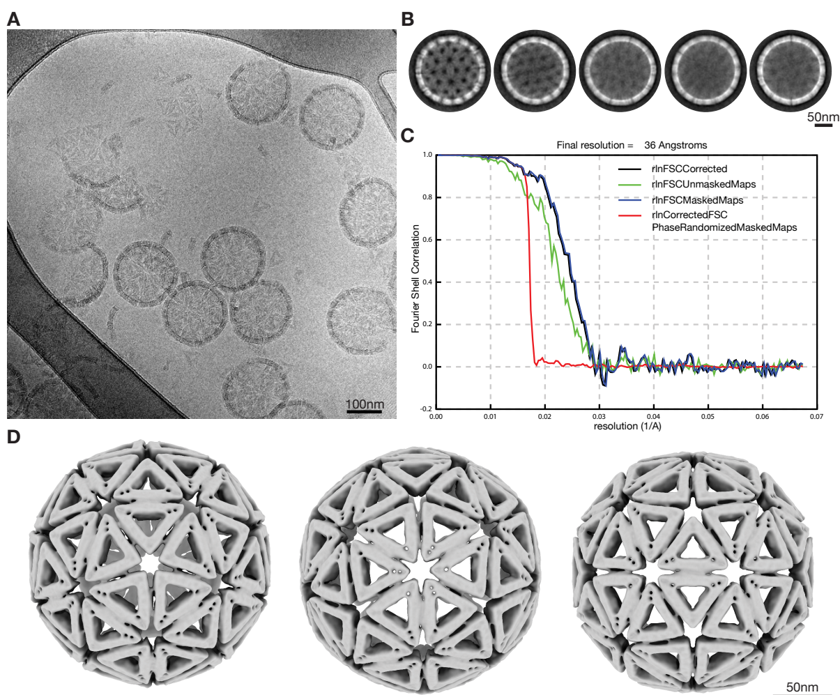
Supplementary Figure 15 | Cryo-EM reconstruction of the T=3 shell at 20 mM \text{MgCl}_2 . (A) Cryo-EM micrograph of T=3 shells on a lacey carbon grid with carbon support. (B) Two-dimensional class averages showing different orientations. (C) Graph showing different FSC curves which were used for resolution estimation. (D) Electron density map shown from the 5-fold, 3-fold and 2-fold symmetry axis (left to right).
