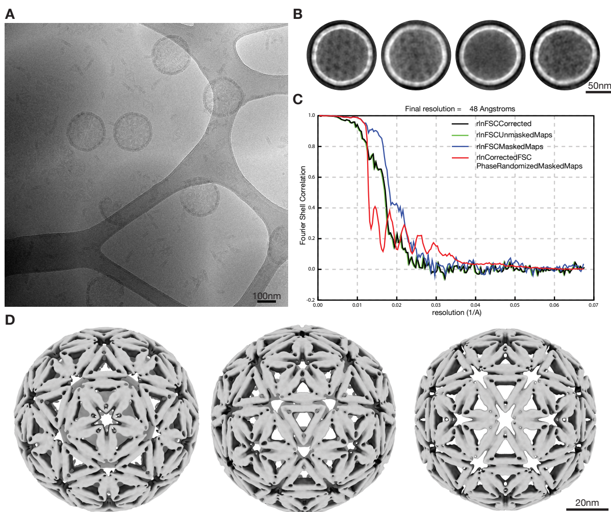
Supplementary Figure 16 | Cryo-EM reconstruction of the T=4 shell at 25 mM \text{MgCl}_2 . (A) Cryo-EM micrograph of T=4 shells on a lacey carbon grid with carbon support. (B) Two-dimensional class averages showing different orientations. (C) Graph showing different FSC curves which were used for resolution estimation. (D) Electron density map shown from the 5-fold, 3-fold and 2-fold symmetry axis (left to right).
