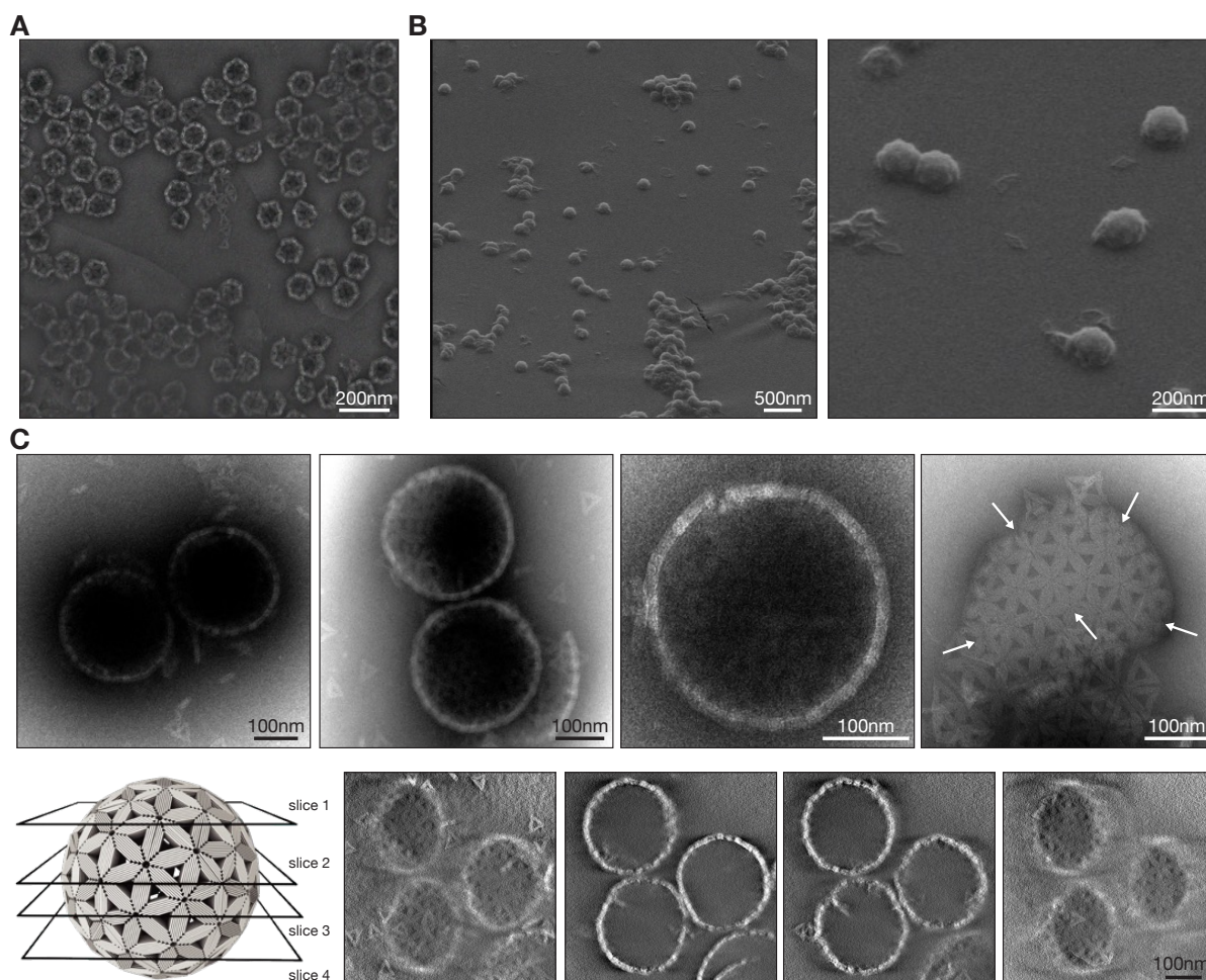
Supplementary Figure 17 | TEM and HIM data of T=1, T=3 and T=9 shells. (A) Negative stain TEM image of assembled T=1 triangles assembled at 25 mM \text{MgCl}_2 . (B) HIM images of T=3 shells coated with a 5 nm layer of AuPd. (C) Negative stain TEM images of assembled T=9 shells. Top: exemplary images of fully or partially assembled shells. The white arrows indicate the right locations of pentamers within the assembly. Bottom: Four slices of a tomogram showing three fully assembled T=9 shells.
