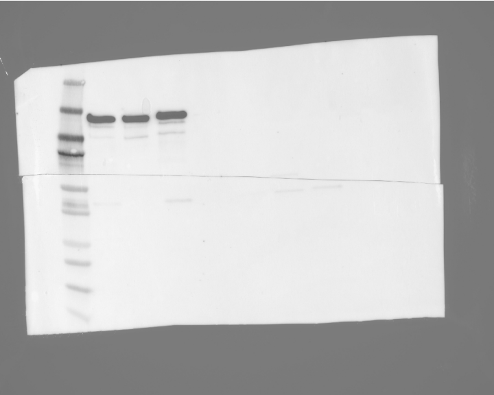
Unprocessed western blot of Fig. 4 c
