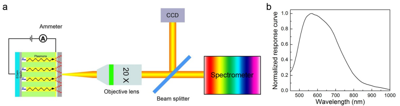
Figure S3 | Optical characterization of electrically driven plasmonic nanorod metamaterials. a , Schematic diagram of the optical characterization setup. b , Normalized spectral response of the detection system, which includes the transmission through the objective lens, beam splitter, optical fibre, reflectivity of grating in the spectrometer, and the quantum efficiency of the CCD in the spectrometer.
