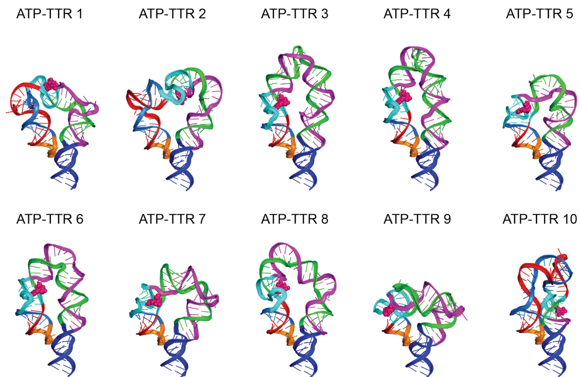
Supplementary Figure 6: Models of 10 ATP-TTRs designed by RNAMake to ‘lock’ the ATP aptamer through a bracing tertiary contact.
