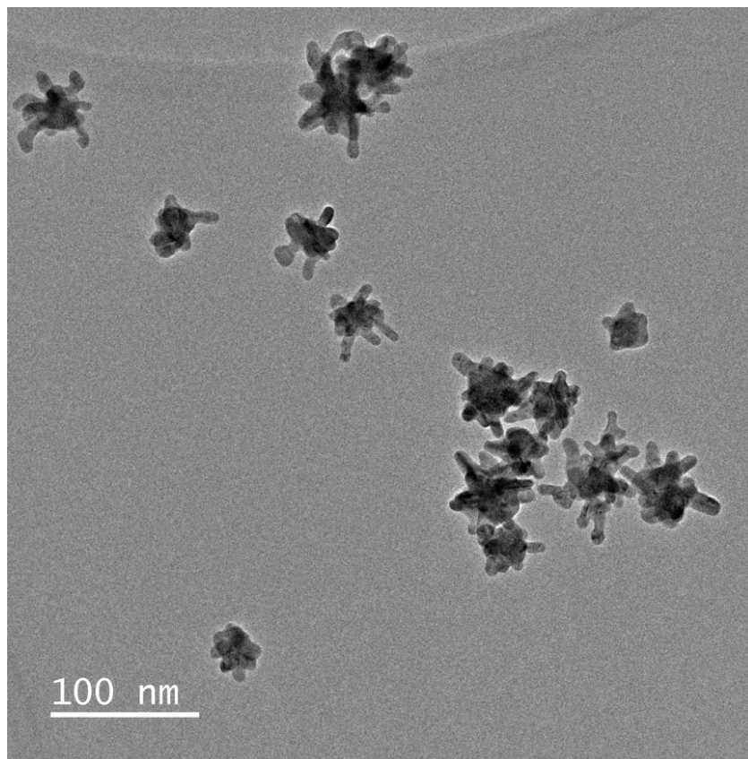
Fig. S8. Nanostars stability after long-term irradiation. TEM image of the nanostars after irradiation with a 940-nm LED at high power level ( \sim 4 dBm) for 15 min/day over a period of 15 days. Nanostars also retained their photothermal efficacy during this period, as verified by thermal imaging of the nanoparticles under long-term pulsed irradiation.
