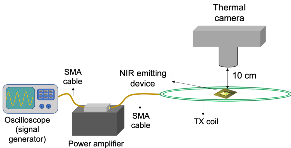
Fig. S31. Thermal imaging of the devices. Setup used for quantitative imaging of temperature variations on the wirelessly-powered NIR-emitting devices before their implantation. Results are shown in Fig. 1D and Supplementary Fig. 32.
