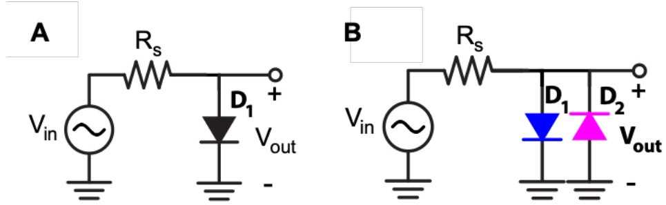
Fig. S16. Two possible device designs which use the rectifying capability of the LED as a diode. (A) Single and (B) back-to-back LED topologies.
