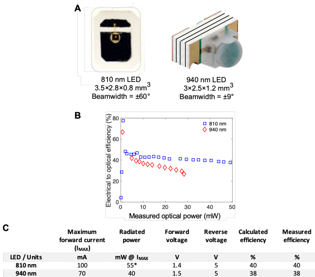
Fig. S12. Characterization of the LEDs used for wireless photothermal therapy. (A) Photographs showing the 810-nm and 940-nm LEDs used in this study, along with their dimensions (L×W×H) and half beam width. (B) Measured efficiency of the 810- and 940-nm LEDs for generating NIR beams with different optical powers. (C) Electrical parameters of the LEDs from the datasheet. The ideal efficiency of each LED was calculated using the data provided by the manufacturers, by assuming a linear scaling of optical power with forward current. The calculated results were in agreement with the measured data. 810-nm and 940-nm LEDs had different I max rating, which limited their maximum allowable electrical power and therefore, their maximum optical power. * Estimated based on similar LEDs from the vendors and our measurements.
