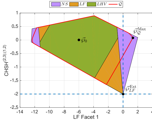
Fig.S.1. Detailed version of Fig. 3 from the main text. The 2-dimensional slice of the space of correlations is the same as in Fig. 3. This slice is spanned by the three points \vec{\wp}_0 , \vec{\wp}_{LF}^{\text{Ext}} , and \vec{\wp}_Q^{\text{Max}} , defined in Eqs. (S.1), (S.2), and (S.3), respectively. The horizontal axis labels the left-hand side of Eq. (13) whereas the vertical axis denoted by \text{CHSH}^{(2,3);(1,2)} is a short hand for the Bell expression appearing in a Semi-Brukner inequality -\langle A_2 B_1 \rangle - \langle A_2 B_2 \rangle - \langle A_3 B_1 \rangle + \langle A_3 B_2 \rangle . Accordingly, the blue dashed lines demarcate the intersection of the boundary of these facets (each representing a half space) with this 2-dimensional slice. In other words, the LF polytope (even beyond this 2-dimensional slice) has to lie above the horizontal dashed line and to the left of the vertical dashed line.
