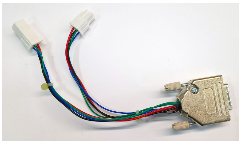
Figure S4. A connector for connecting the syringe pumps to RS232 port.
