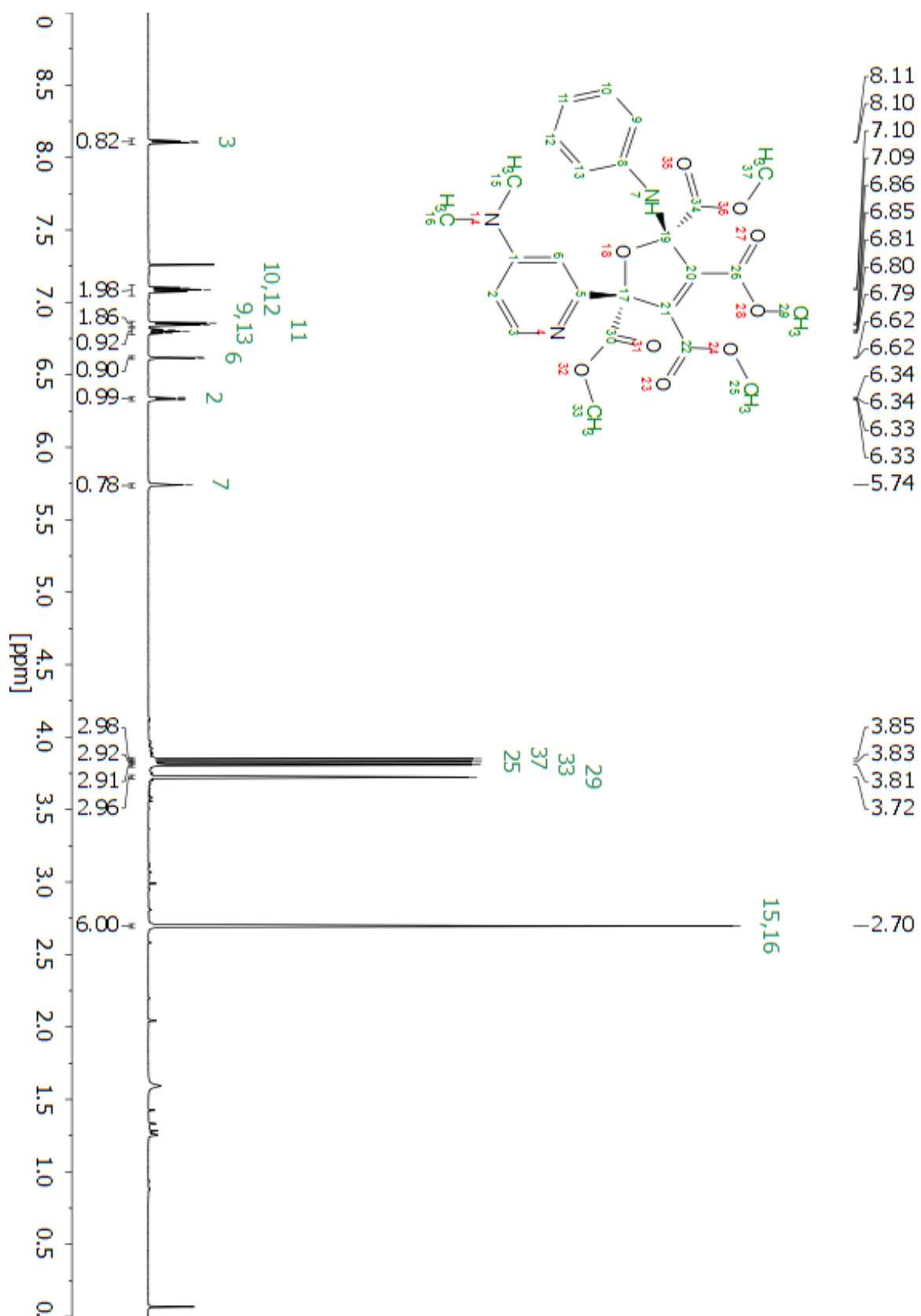
Figure S62. Proton assignments for compound trans -20 and atom numeration.
