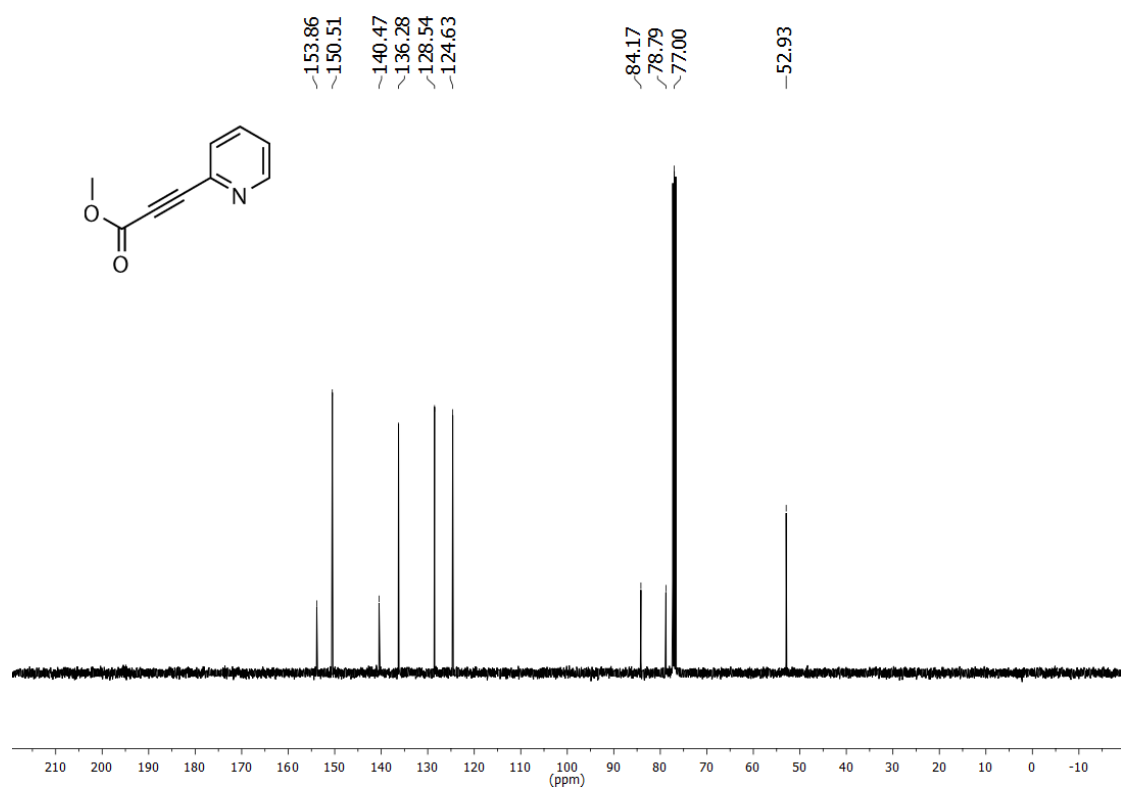
Figure S29. 13 C NMR spectrum of compound S4.
