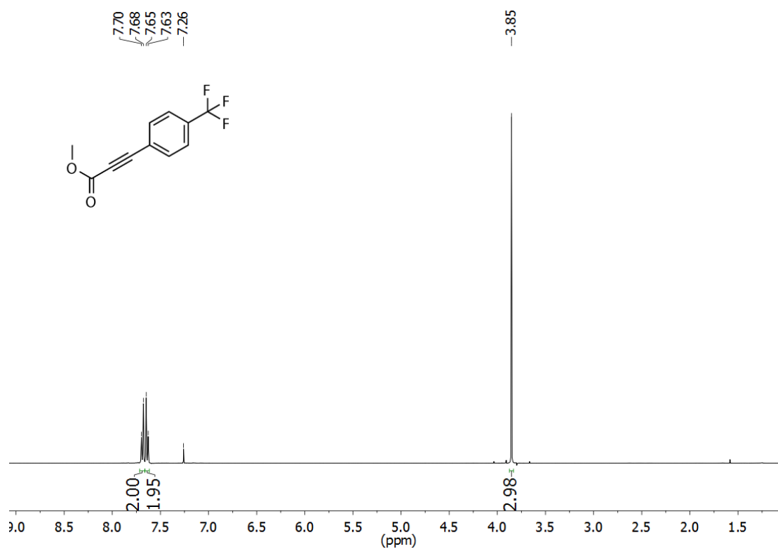
Figure S30. 1 H NMR spectrum of compound S5.
