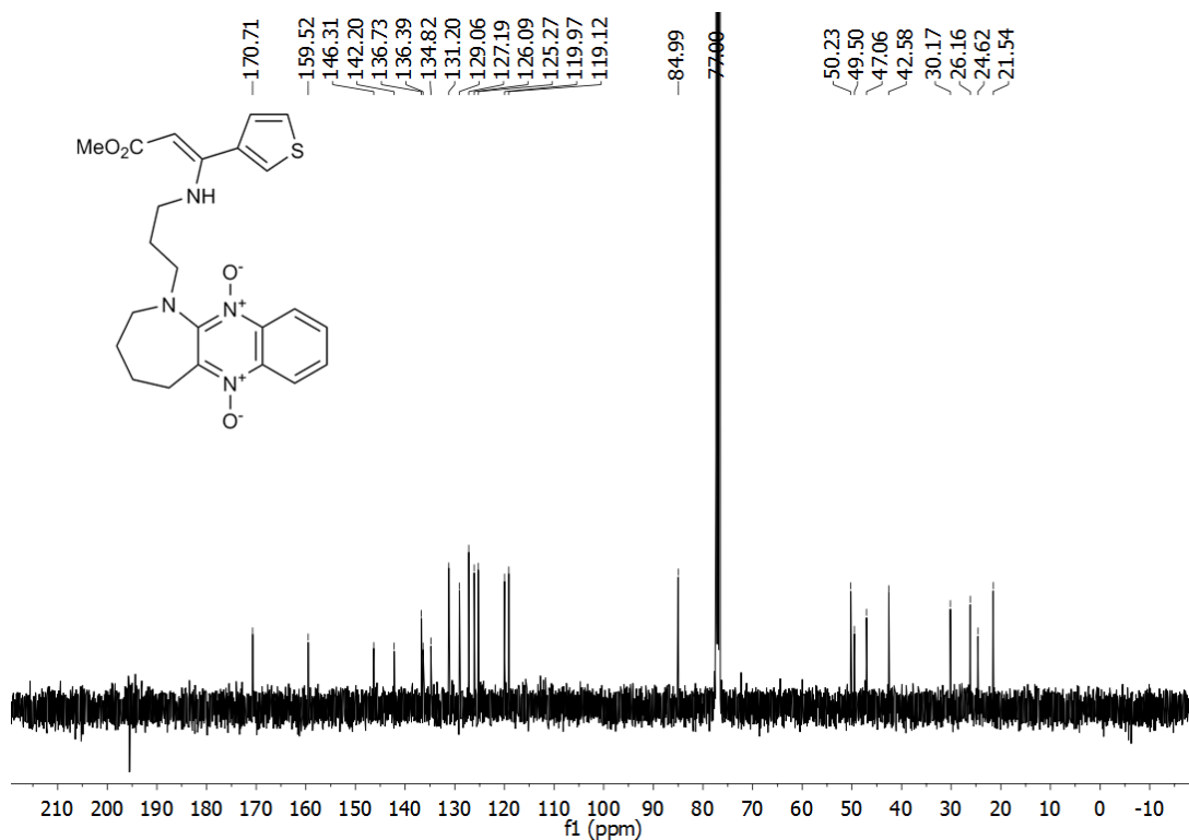
Figure S27. 13 C NMR spectrum of compound 19f.
