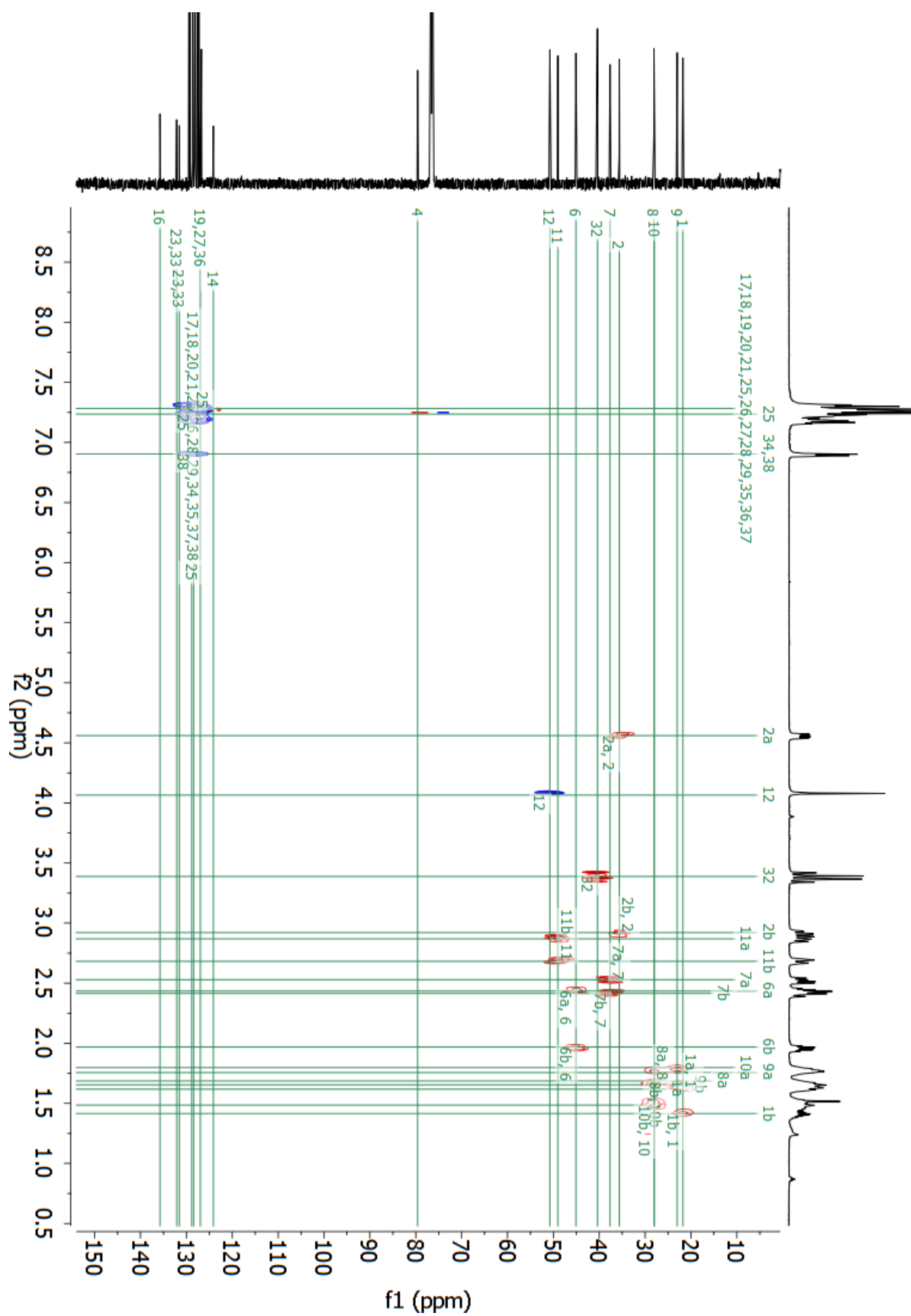
Figure S46. Phase sensitive HSQC spectra of compound 22.
