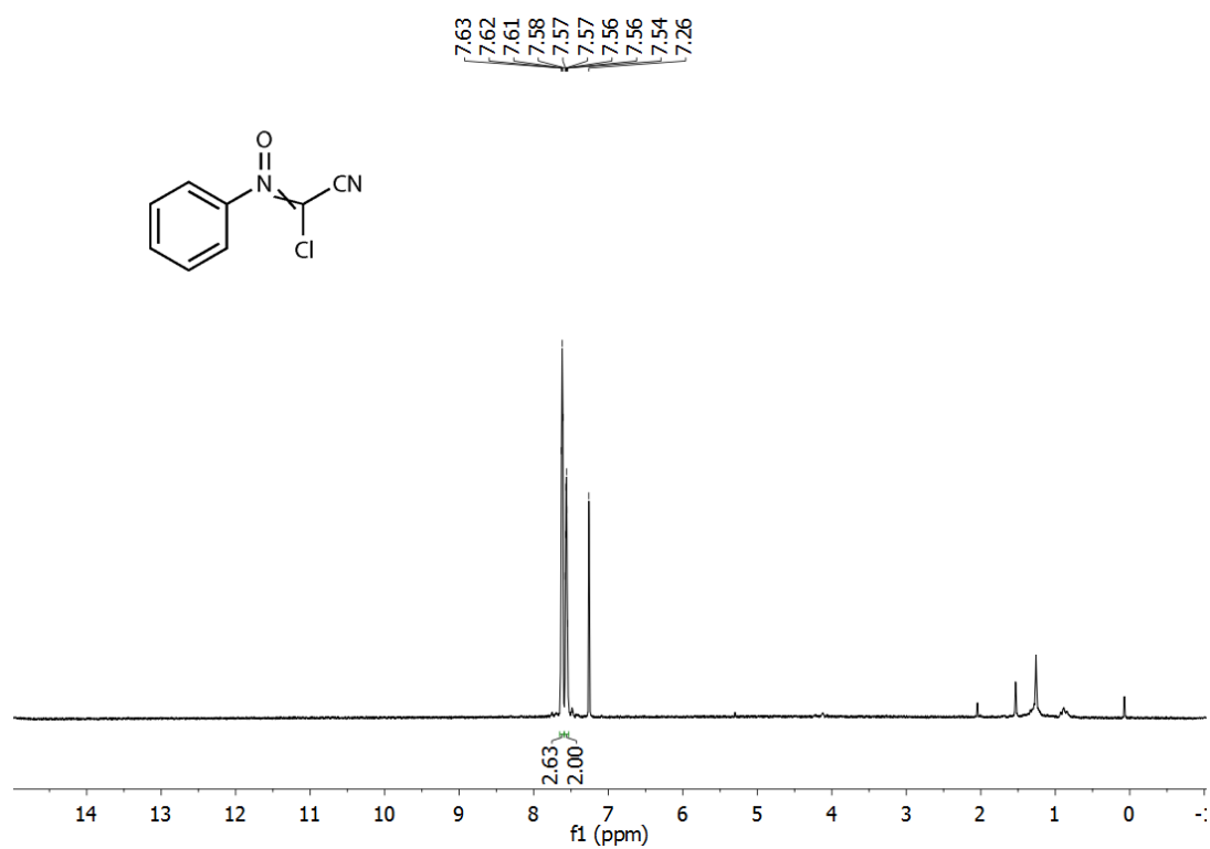
Figure S38. 1 H NMR spectrum of compound 21 .
