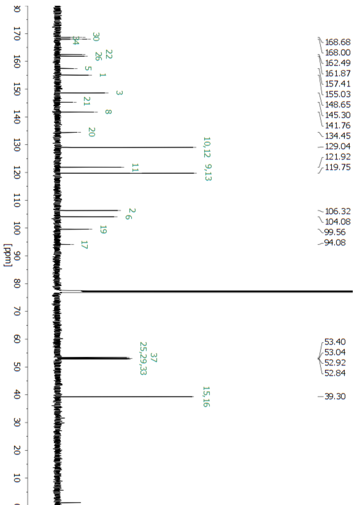
Figure S58. Carbon assignments for compound cis -20 and atom numeration.
