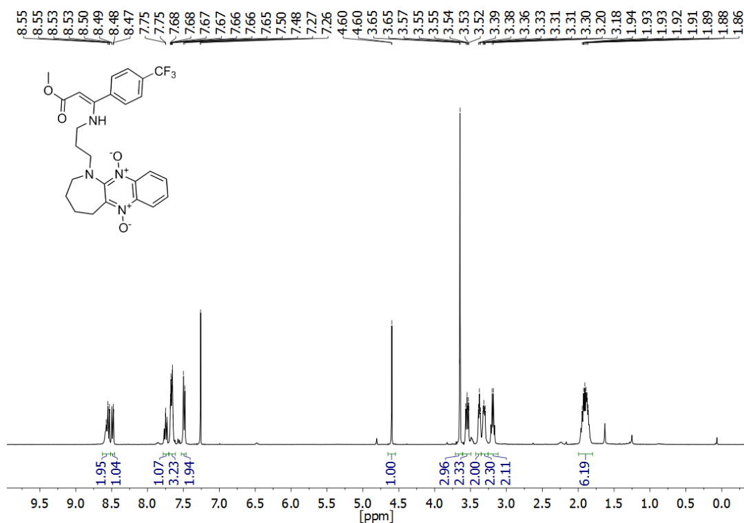
Figure S20. ^1\text{H} NMR spectrum of compound 19c .
