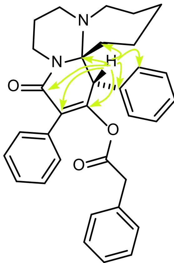
Figure S50. Key ^1\text{H} - ^{13}\text{C} correlations from HMBC spectrum confirming structure of 22 .
