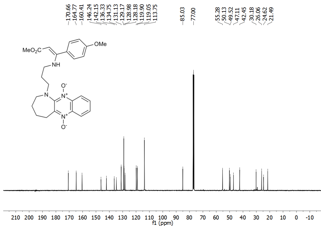
Figure S25. 13 C NMR spectrum of compound 19d .
