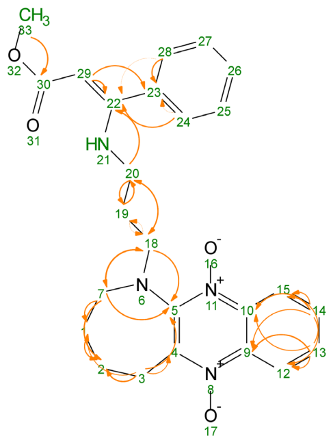
Figure S55. a) Key ^1\text{H} - ^{13}\text{C} correlations from HMBC spectrum b) ^1\text{H} - ^1\text{H} correlation from COSY confirming structure of 19b .
