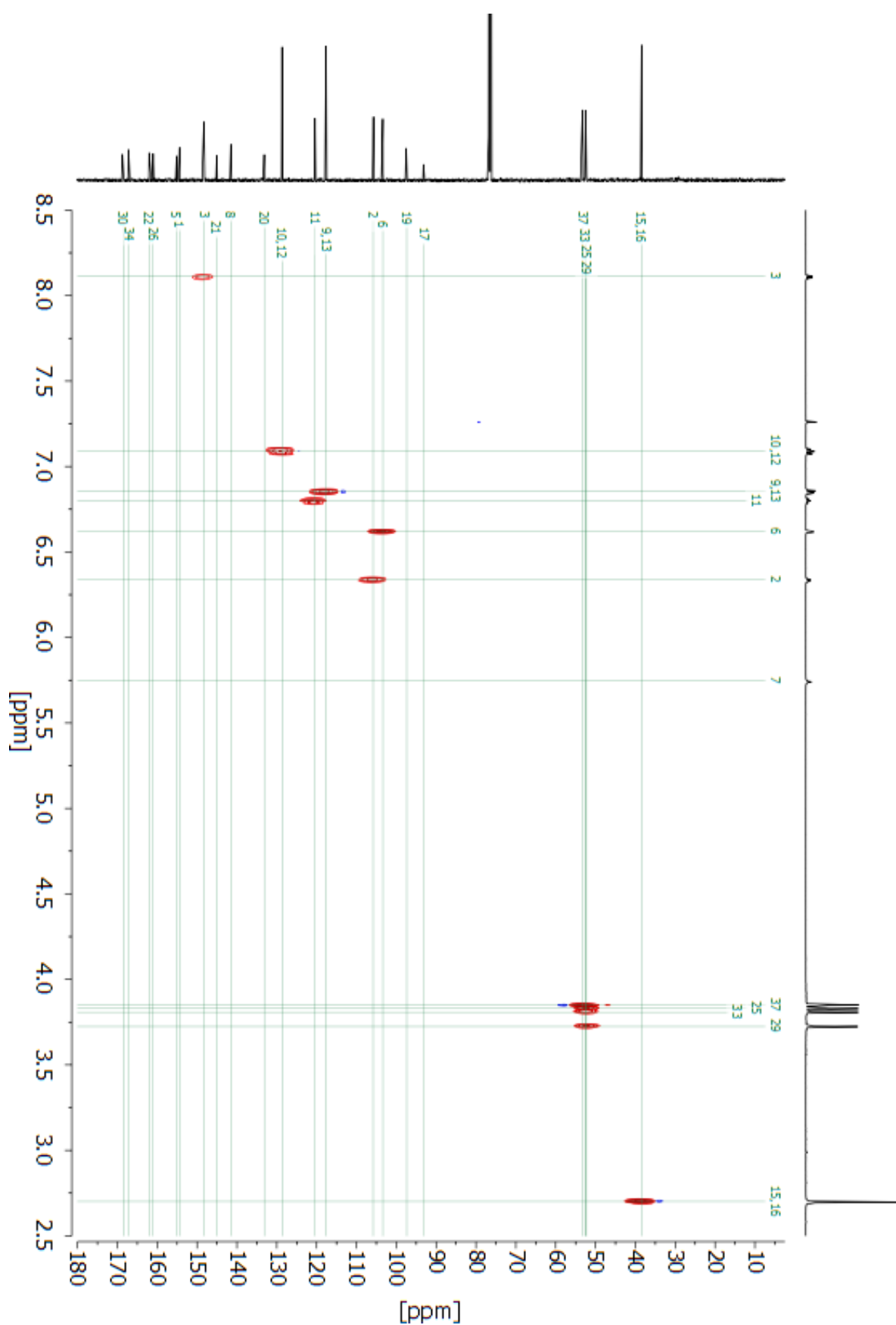
Figure S64. ^1\text{H} - ^{13}\text{C} HSQC correlation for compound trans -20 and signal assignment.
