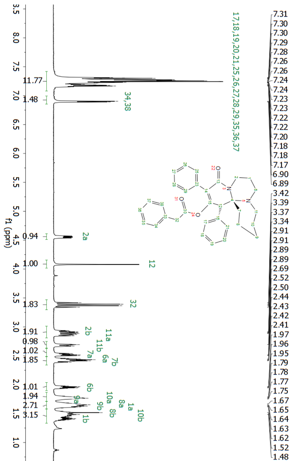
Figure S44. Proton assignments for compound 22 and atom numeration.
