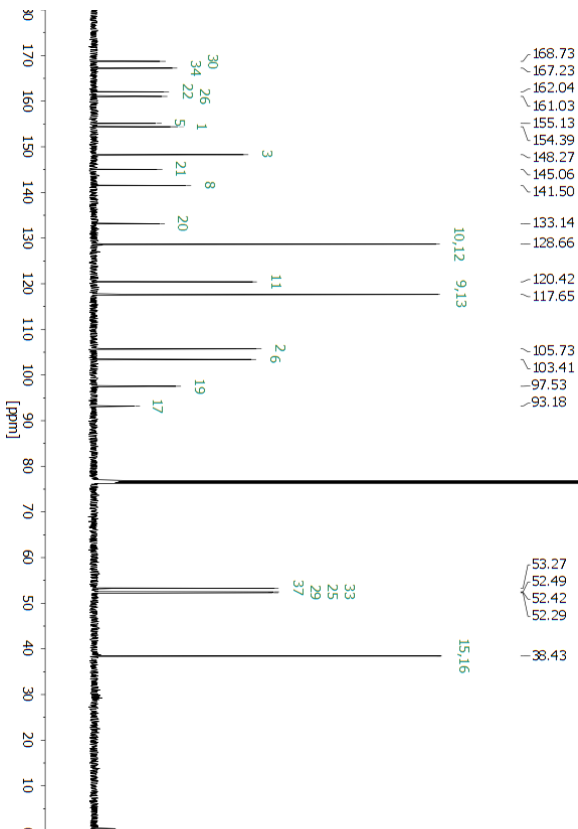
Figure S63. Carbon assignments for compound trans -20 and atom numeration.
