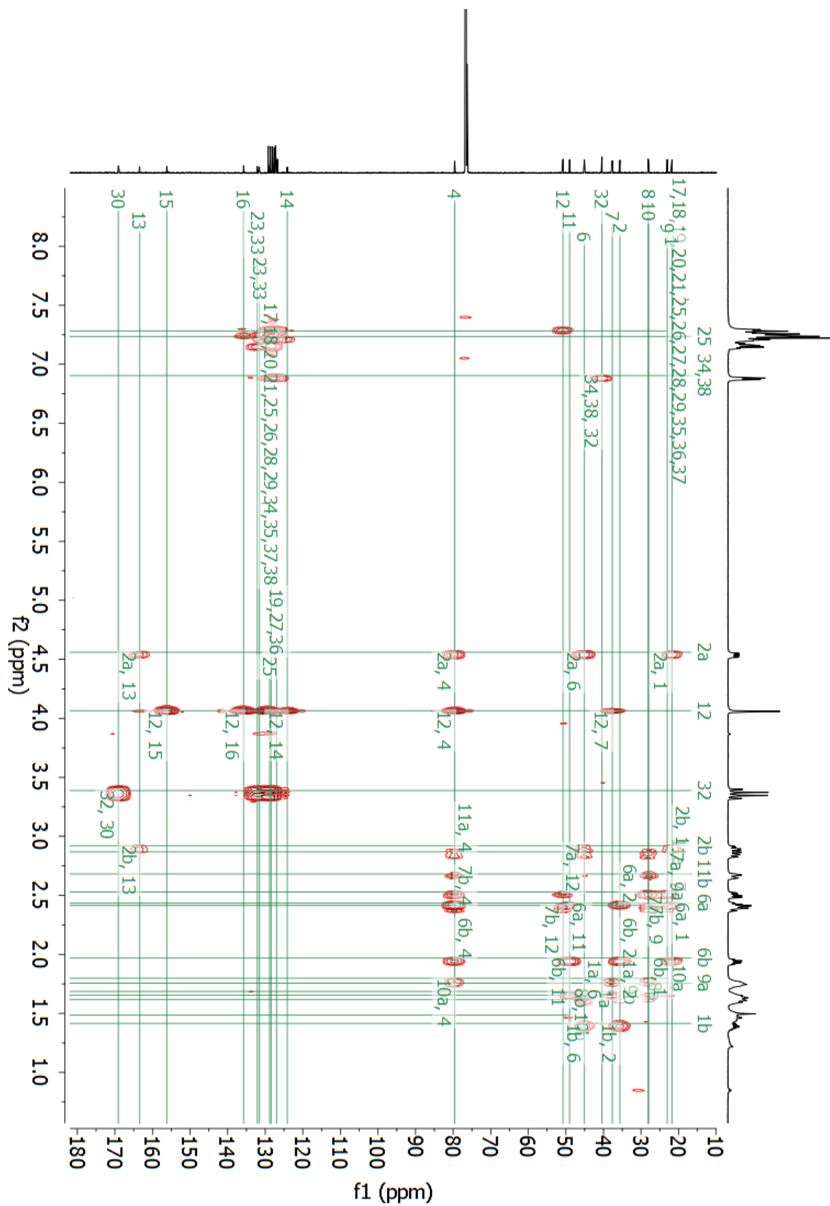
Figure S47. HMBC spectrum of compound 22.
