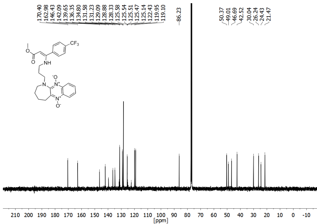
Figure S21. ^{13}\text{C} NMR spectrum of compound 19c .
