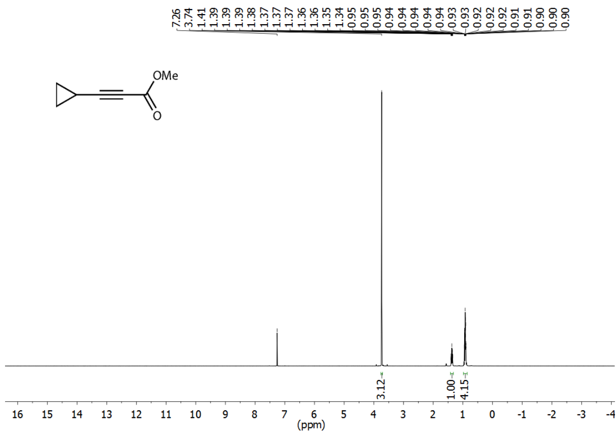
Figure S32. 1 H NMR spectrum of compound S1.
