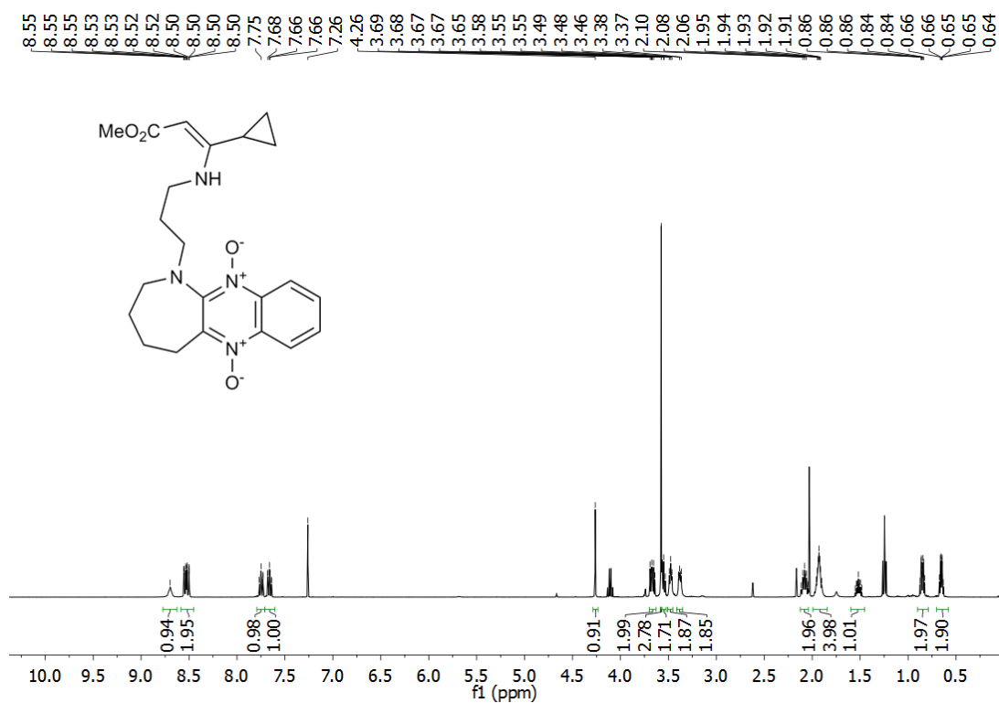
Figure S22. 1 H NMR spectrum of compound 19g.
