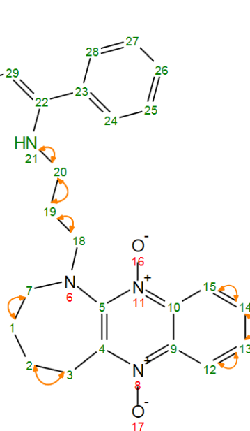
Figure S55. a) Key ^1\text{H} - ^{13}\text{C} correlations from HMBC spectrum b) ^1\text{H} - ^1\text{H} correlation from COSY confirming structure of 19b .
