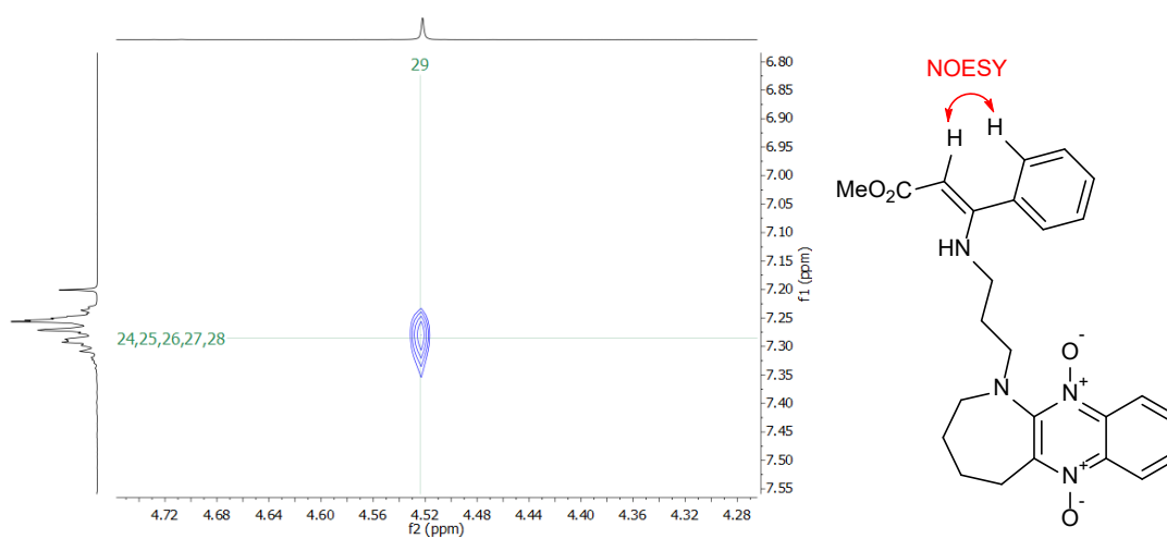
Figure S56. 2D NOESY cross-peak confirming the Z configuration of compound 19b .
