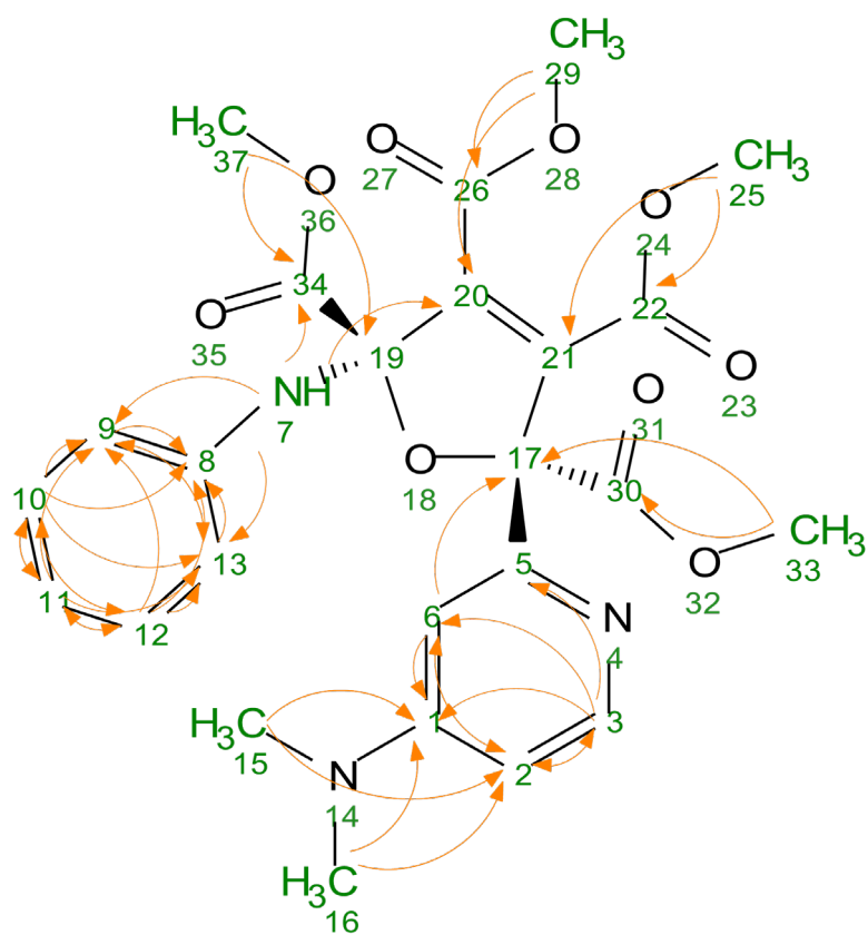
Figure S61. Key 1 H- 13 C correlations from HMBC spectrum confirming structure of cis -20.
