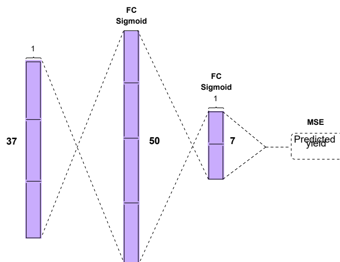
Figure S72. The structure of the neural network used for yield prediction.
