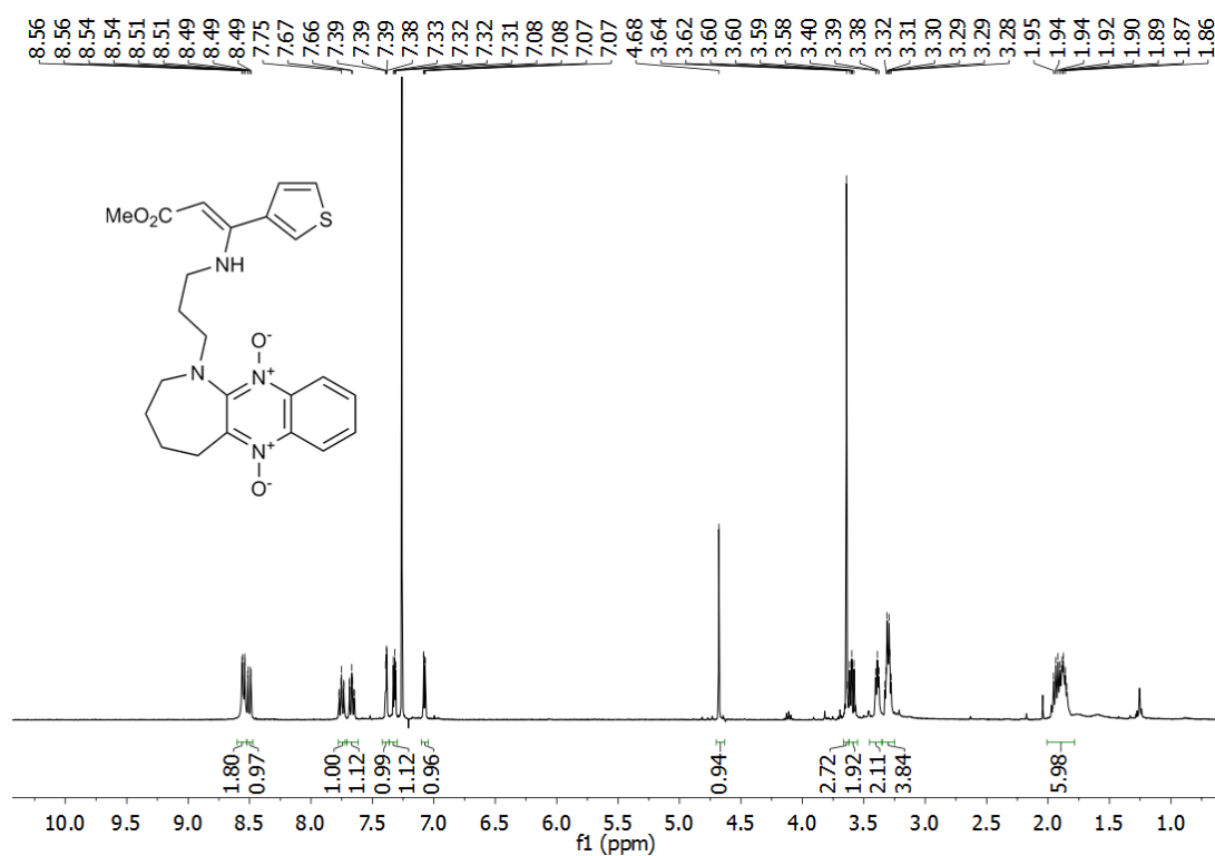
Figure S26. 1 H NMR spectrum of compound 19f.
