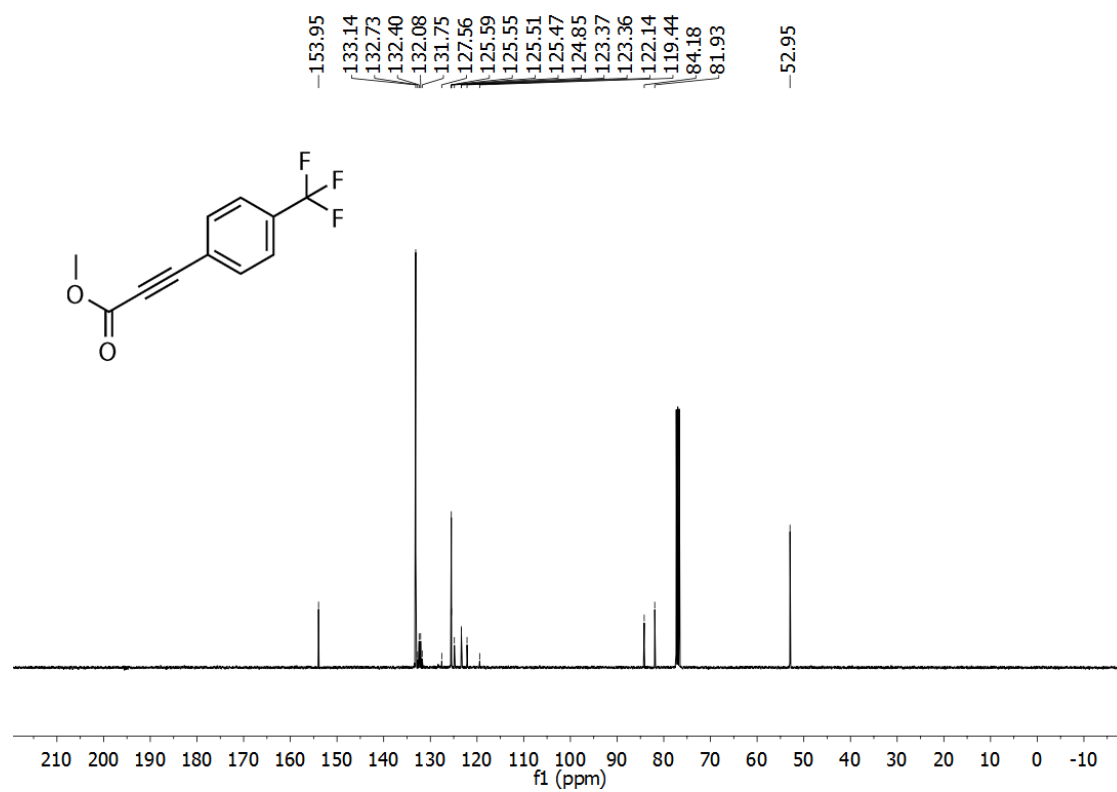
Figure S31. 13 C NMR spectrum of compound S5.
