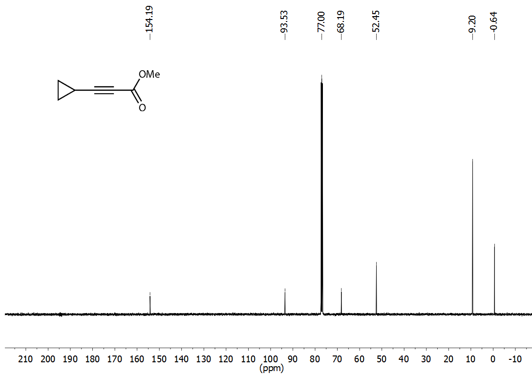
Figure S33. 13 C NMR spectrum of compound S1.
