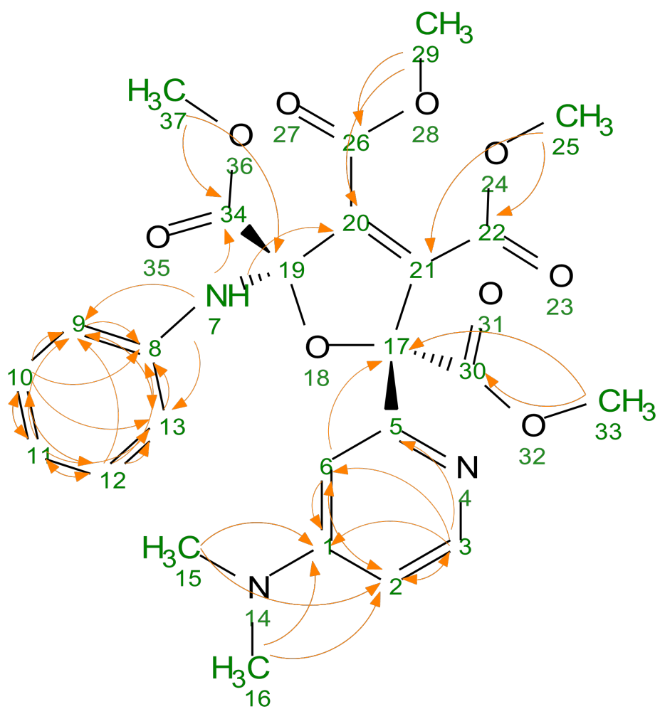
Figure S66. Key ^1\text{H} - ^{13}\text{C} correlations from HMBC spectrum confirming structure of trans -20.
