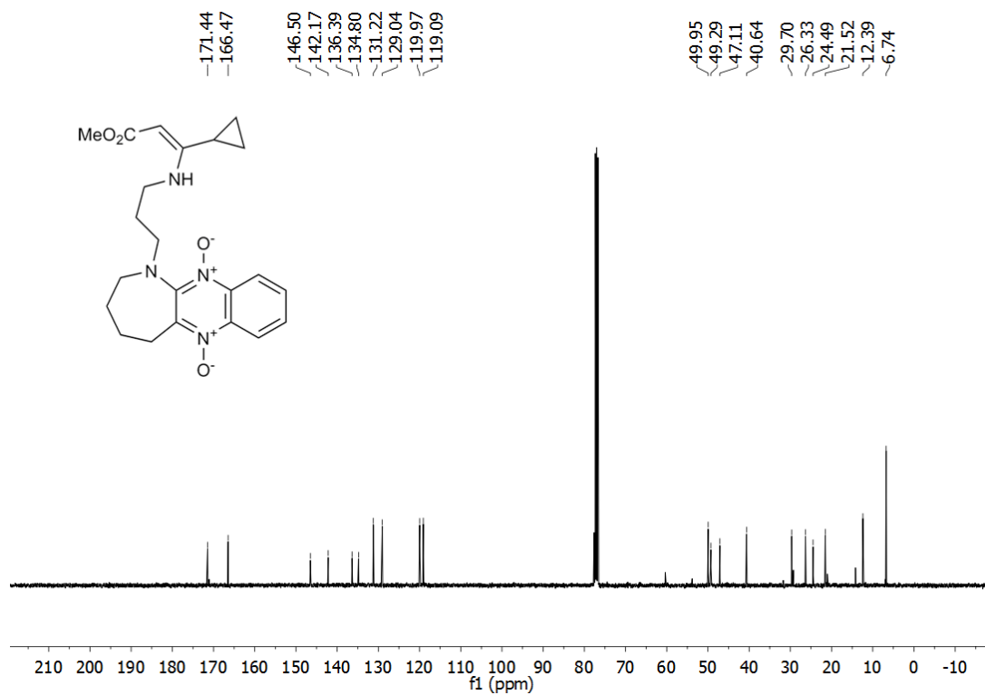
Figure S23. 13 C NMR spectrum of compound 19g.
