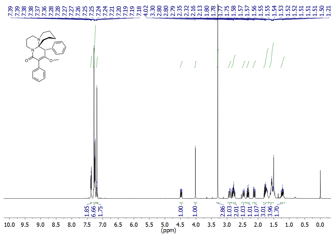
Figure S42. 1 H NMR spectrum of compound S6.
