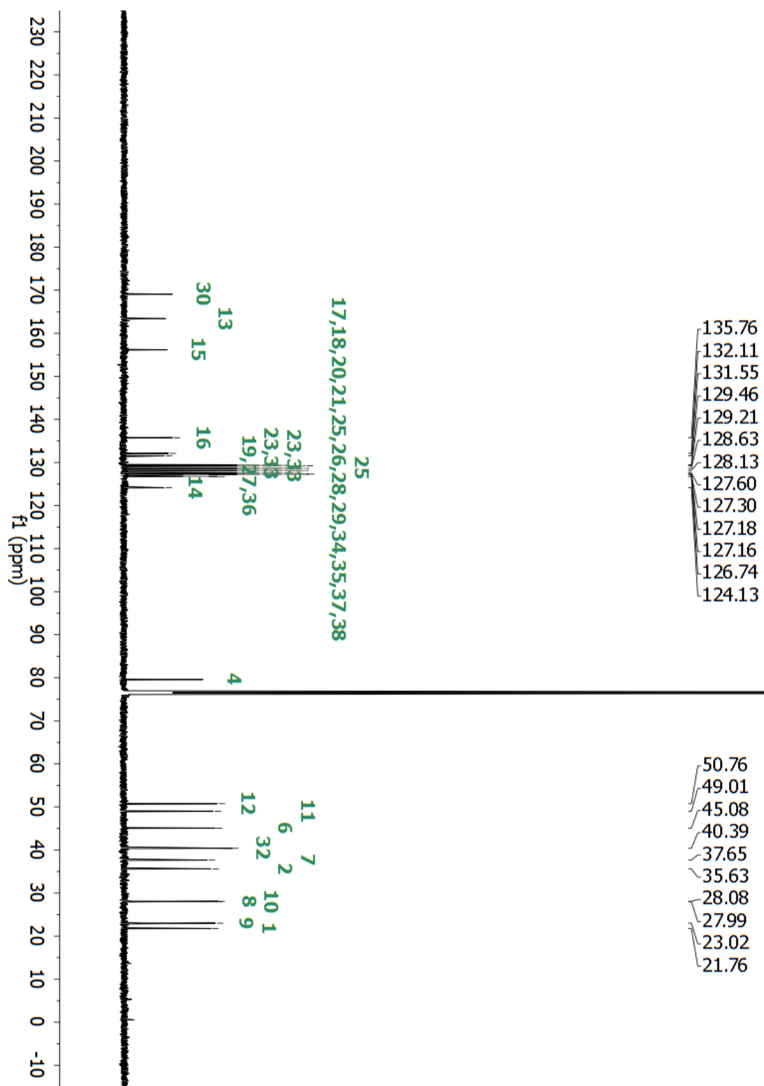
Figure S45. Carbon assignments for compound 22.
