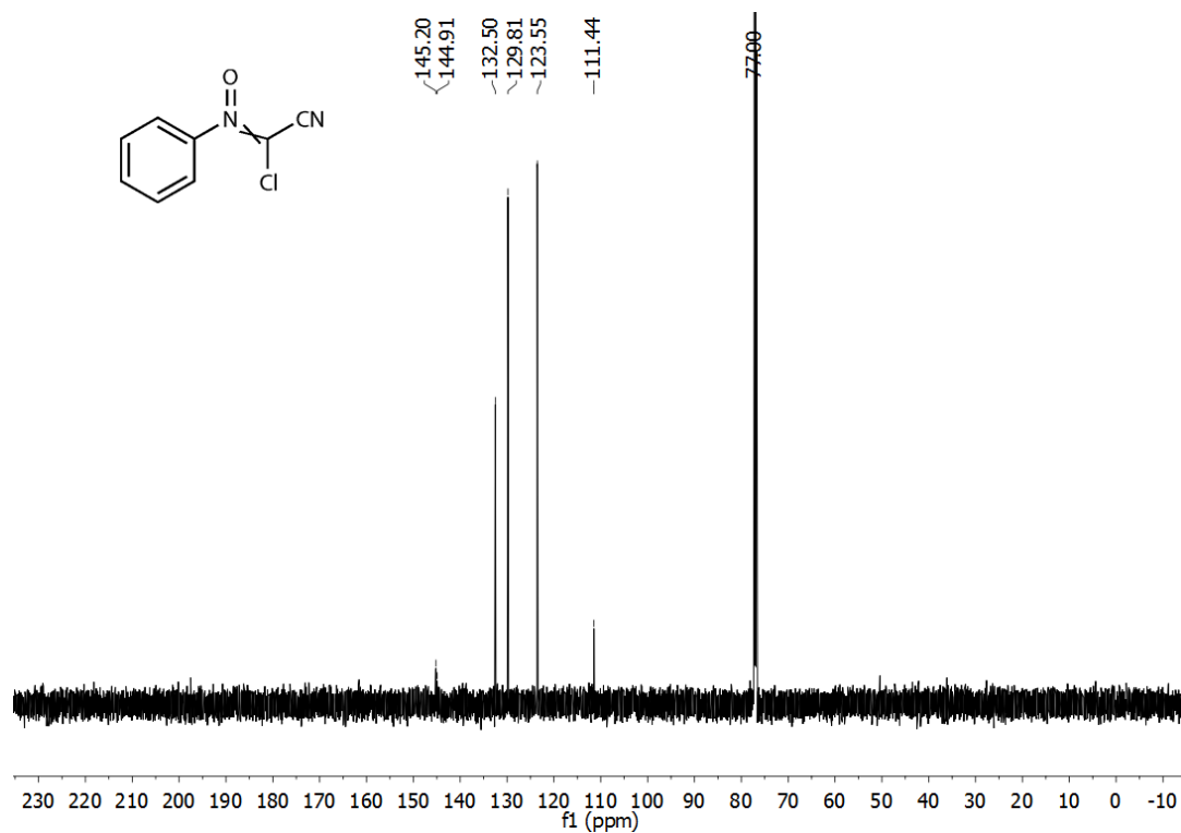
Figure S39. 13 C NMR spectrum of compound 21 .
