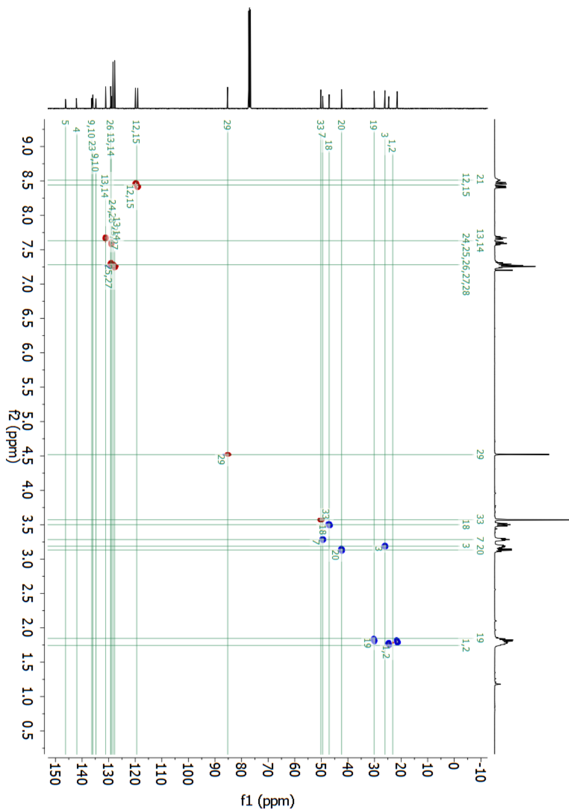
Figure S53. ^1\text{H} - ^{13}\text{C} HSQC spectrum of compound 19b and signal assignment.
