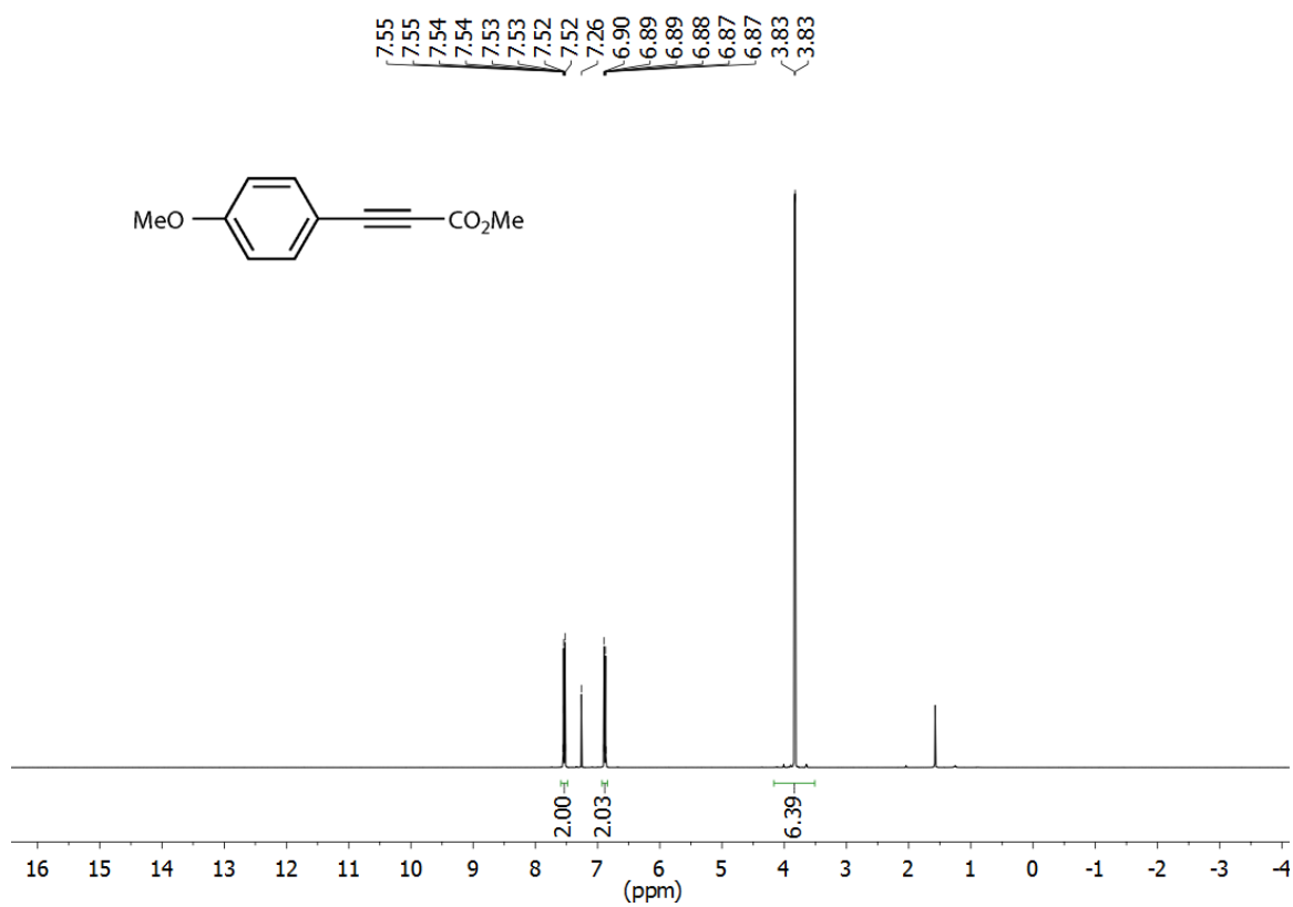
Figure S34. 1 H NMR spectrum of compound S2.
