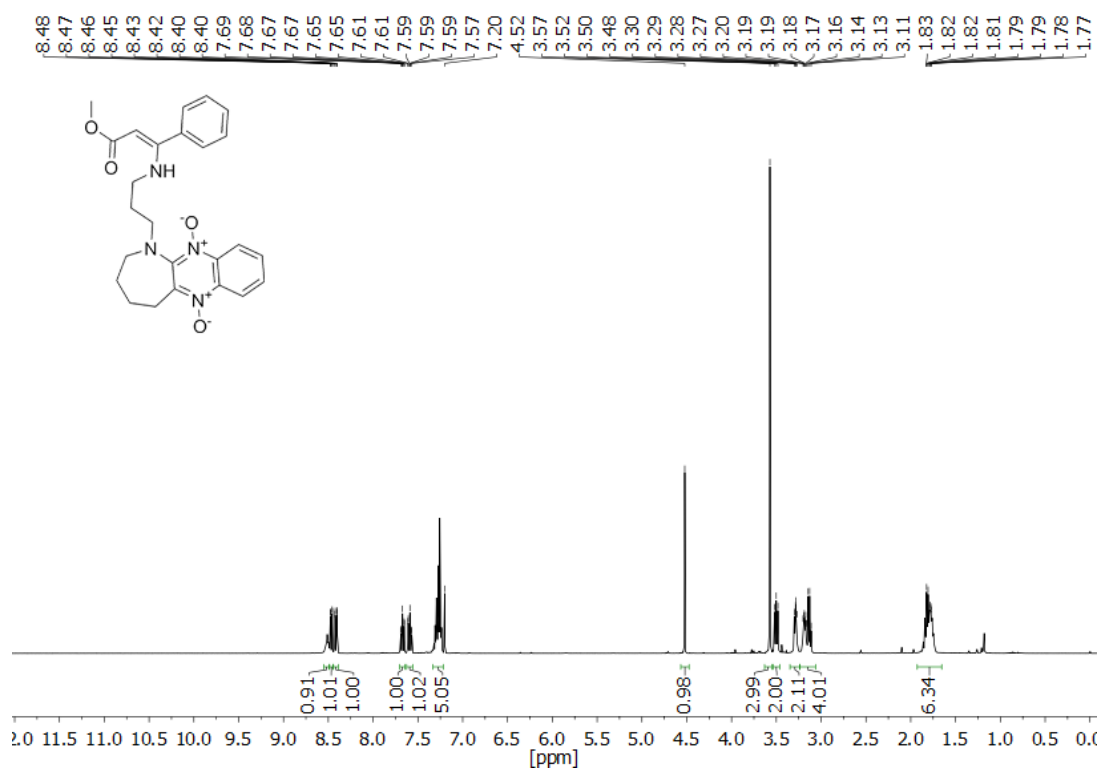
Figure S16. ^1\text{H} NMR spectrum of compound 19b .
