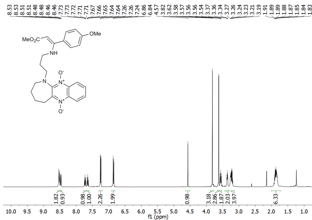
Figure S24. 1 H NMR spectrum of compound 19d .
