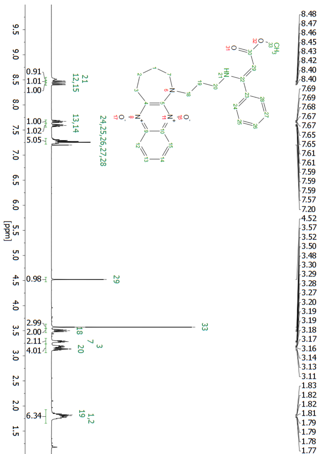
Figure S51. Assignments of 1 H NMR signals for compound 19b and numeration of atoms.
