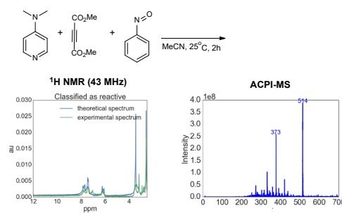
Figure S12. Real time spectra recorded for the new transformations.
