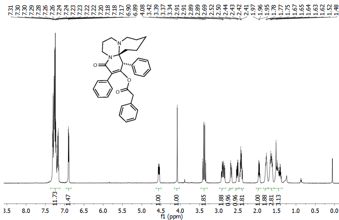
Figure S40. 1 H NMR spectrum of compound 22 .
